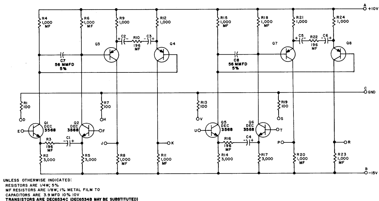
Figure 4-23 Difference Amplifier, Type W532
