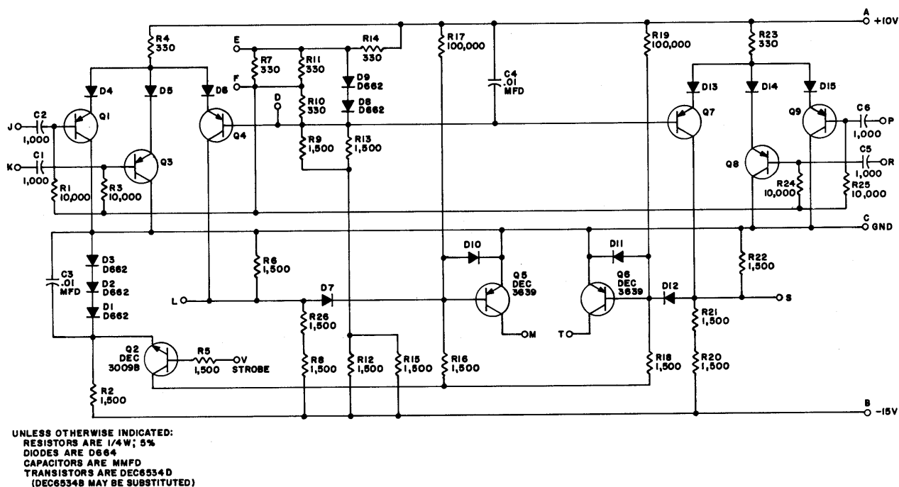
Figure 4-24 Rectifying Slicer, Type W533
