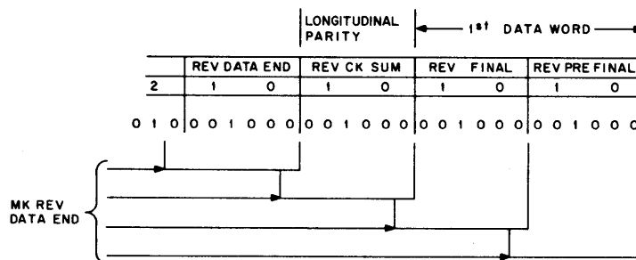
Figure 3-11 Data End Mark Decoding
