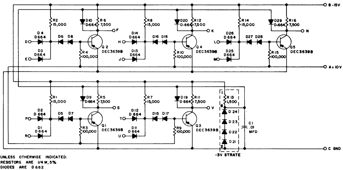
Figure 4-8 Diode Gate, Type R113
