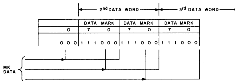
Figure 3-12 Data Mark Decoding
