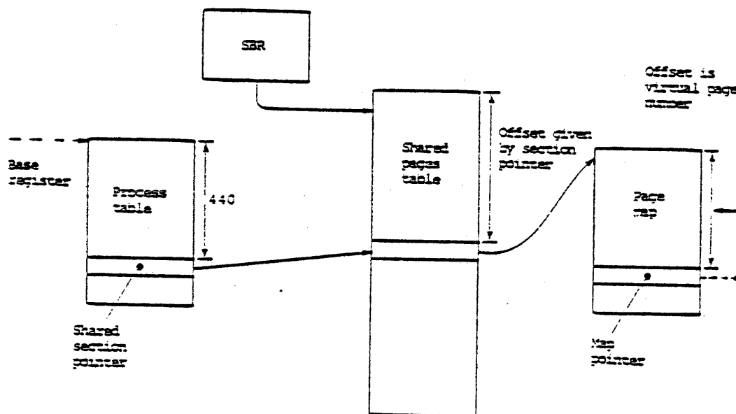
Shared Section Pointer Structure
