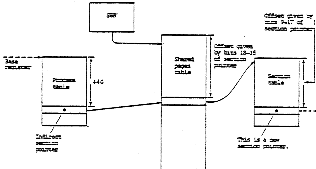
Indirect Section Pointer Structure
