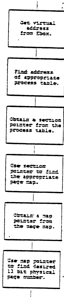
KL-Style Paging Algorithm
