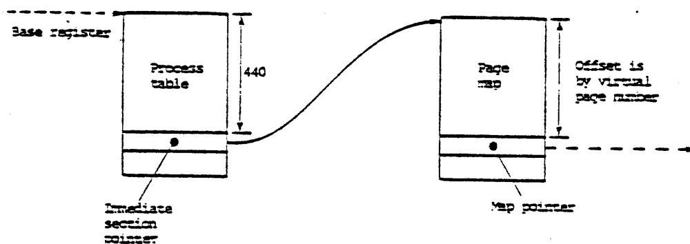
Immediate Section Pointer Structure
