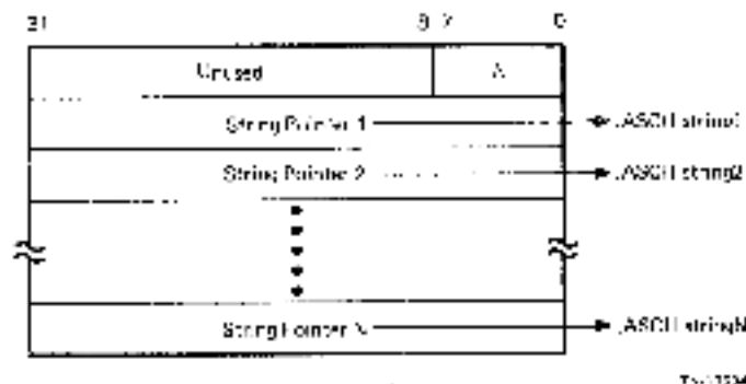
Figure 4-4 "Valtab" Table Format
