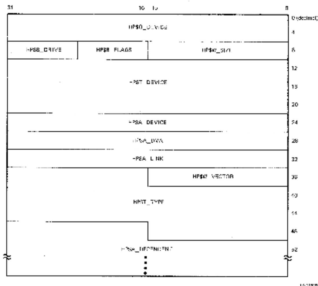
Figure 3-4 P-Table Layout
