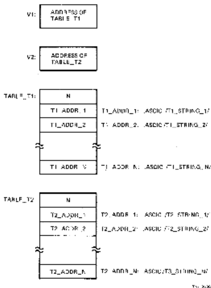
Figure 4-6 SDS_CVTRES Value Mnemonics Table Usage
