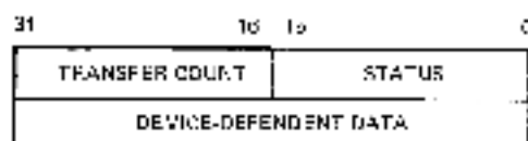
Figure 3-18 I/O Status Block Format
