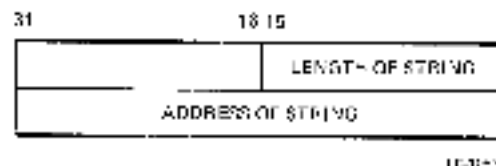
Figure 4-1 Quadword String Descriptor
