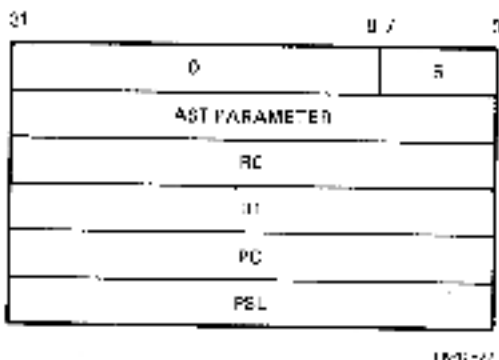
Figure 3-12 Argument List Passed to an AST Routine
