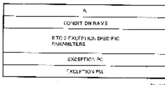
Figure 3-14 Format of Signal Array
