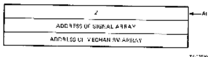
Figure 3-13 Argument List Passed to a Condition Handler
