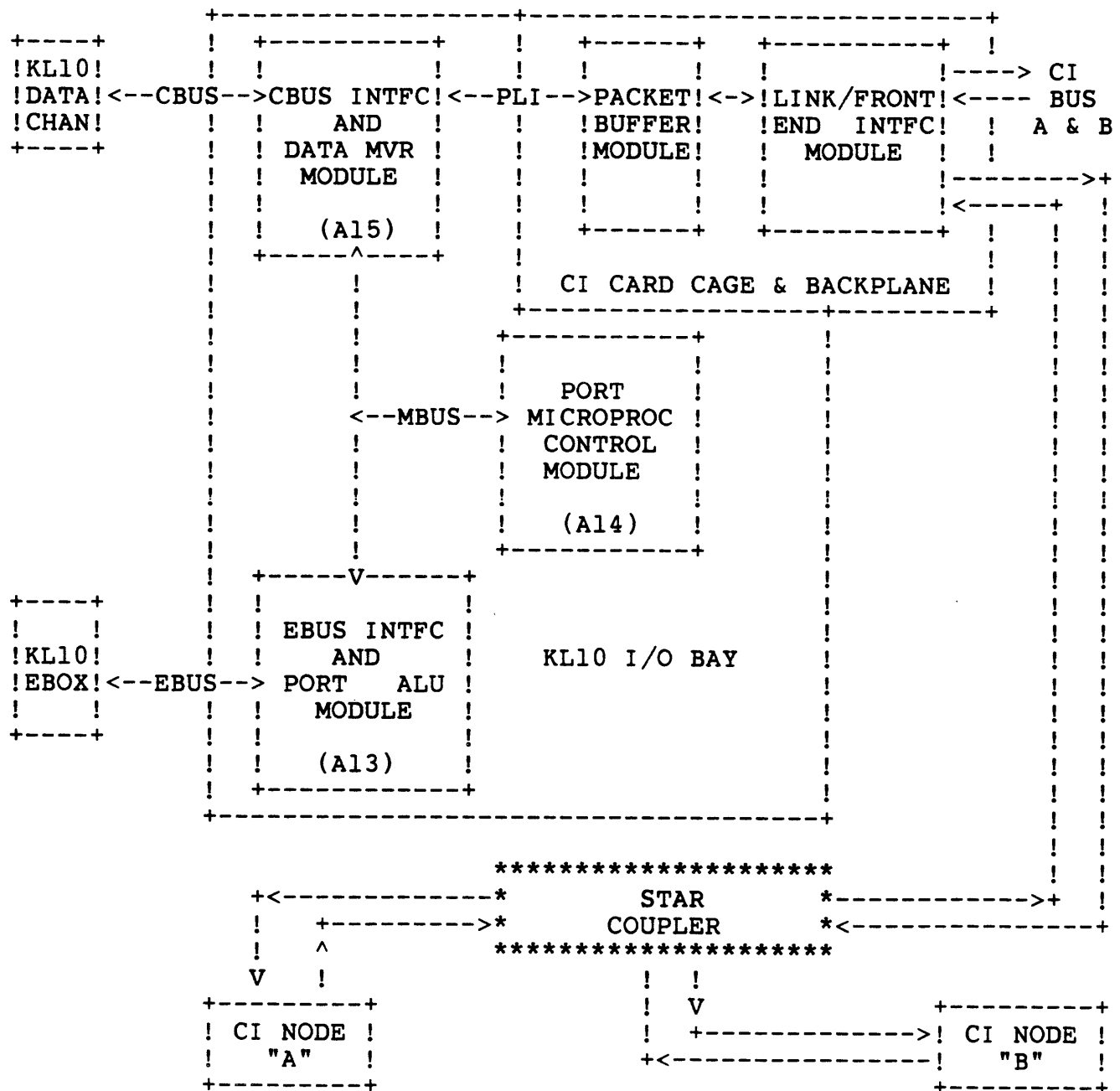
SIMPLIFIED CI20 PORT/LINK INTERFACE BLOCK DIAGRAM
