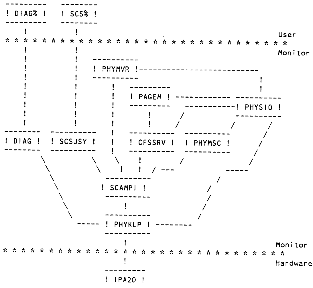
Figure 1 - CI-20 Software Components
