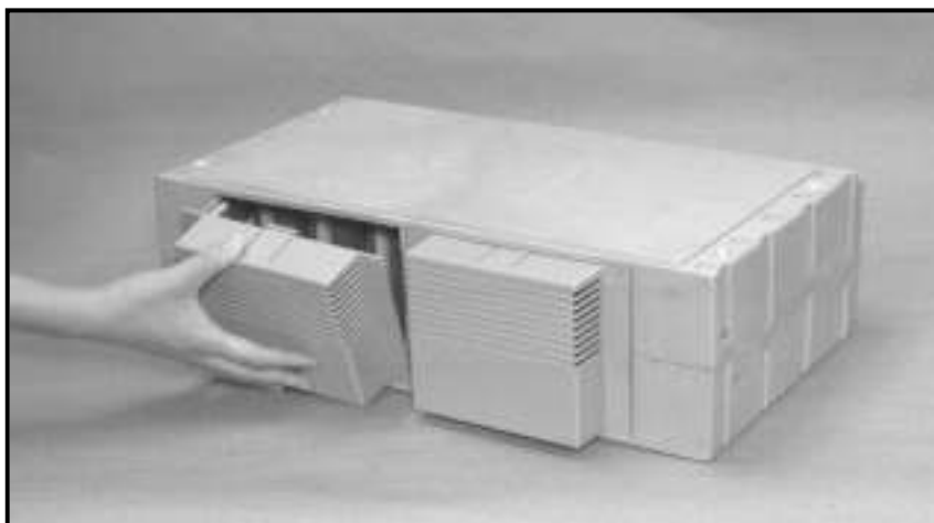
Figure 1–5 Replacing Blowers
