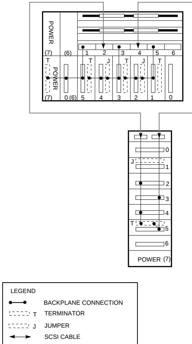
Figure 3–2 5x2 Bus Schematic
