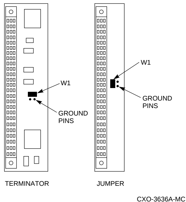
Figure 1–3 SHELF_OK Signal Jumper W1
