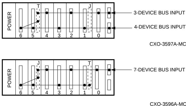
Figure 3–1 BA350–LA SCSI Buses
