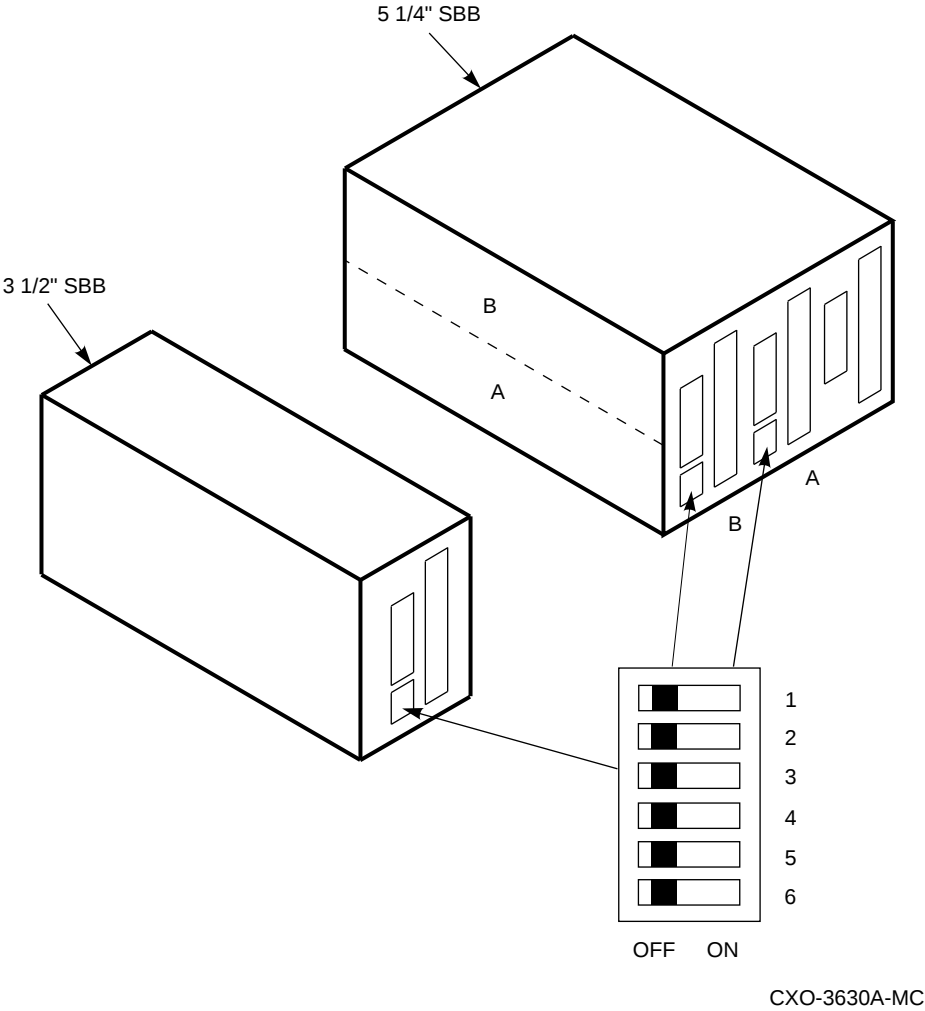
Figure 2–1 SBB Device Address Switch
