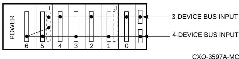
Figure 3–3 Single BA350–LA Shelf for Two SCSI Buses
