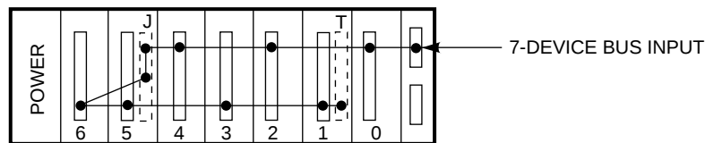
Figure 3–2 Single BA350–LA Shelf for One SCSI Bus
