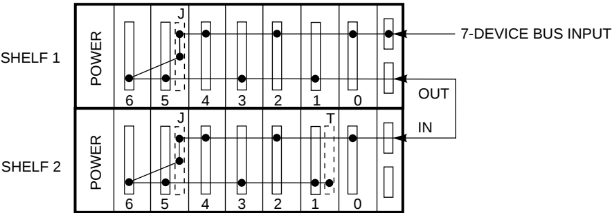
Figure 3–4 Single SCSI Bus on Two BA350–SA Shelves
