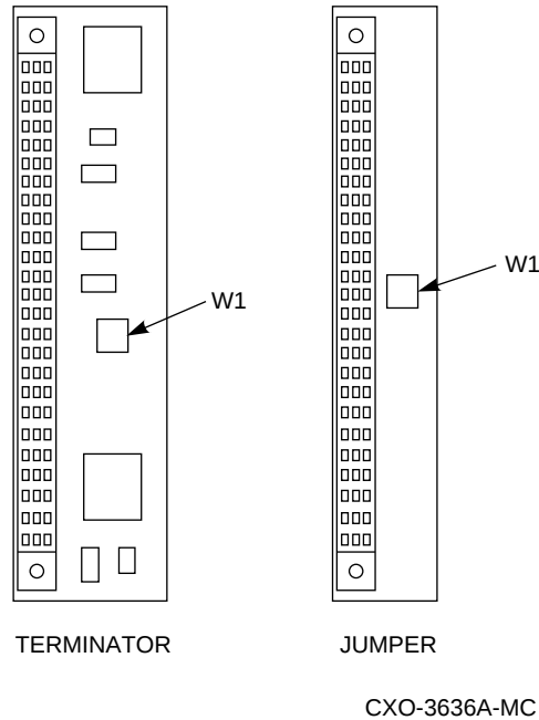
Figure 1–3 SHELF_OK Signal Jumper W1
