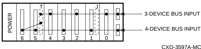
Figure 3–3 BA350–SA SCSI Buses
