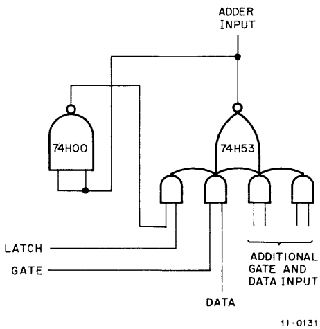
Figure 4-6 Latch Input Gating
