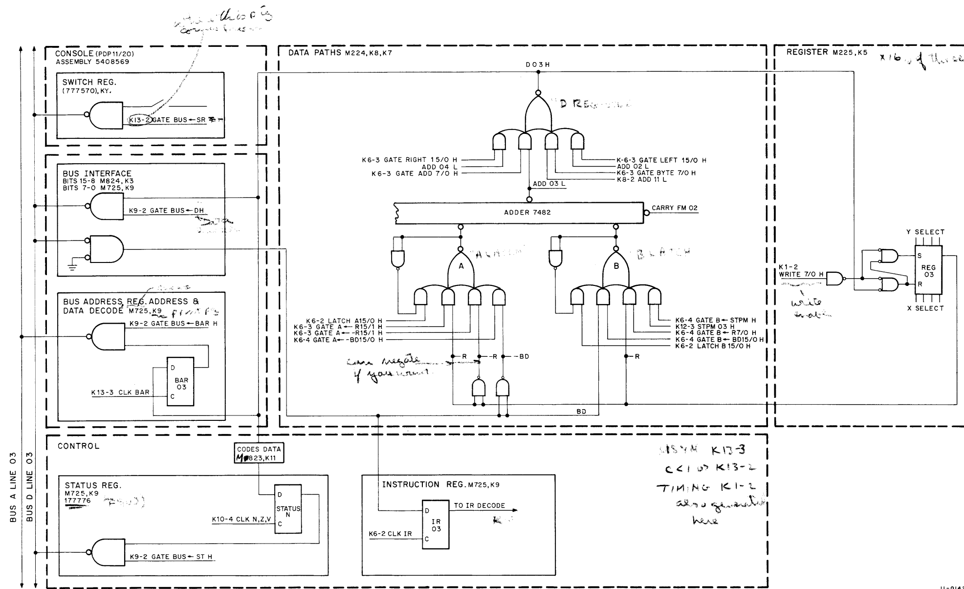
Figure 1-2 Processor Block Diagram Showing One-Bit (03) Data Slice
