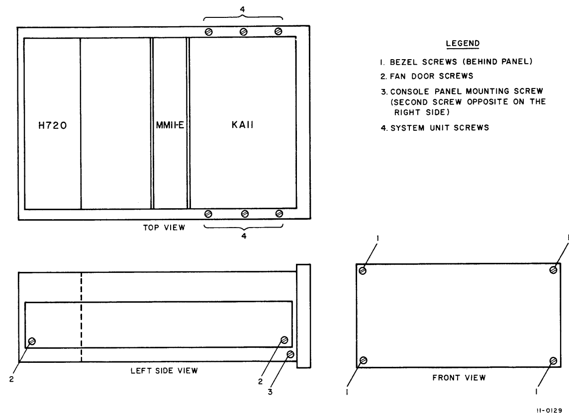
Figure 5-2 Mounting Hardware
