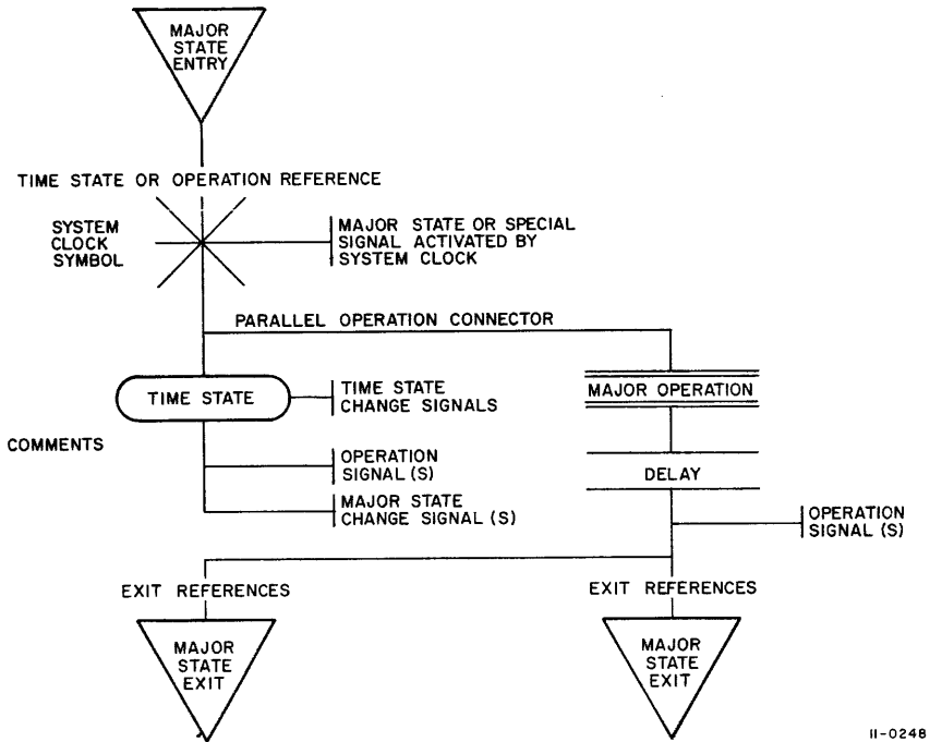
Figure 3-4 PDP-11 Processor Flow Chart Composite Layout and Symbol System
