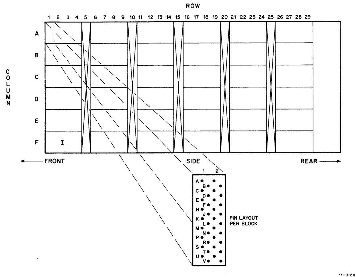
Figure 5-1 Typical System Layout
