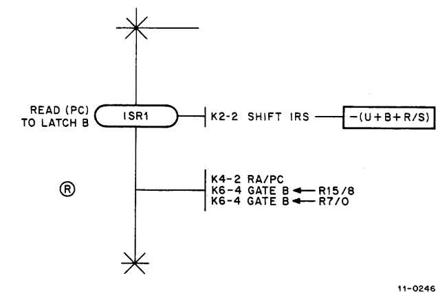
Figure 3-2 Portion of EXECUTE * JSR Flow Chart
