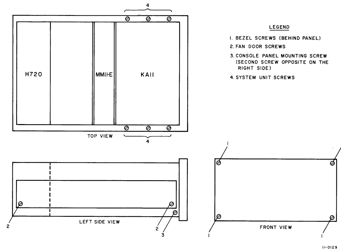
Figure 5-2 Mounting Hardware
