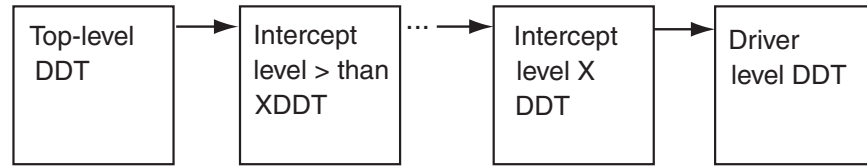
Figure 4-1 DDT Intercepts
