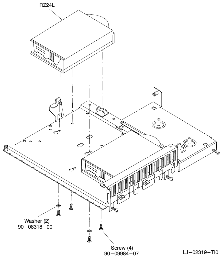
Figure 1–8 Lower Drive Shelf Mounting
