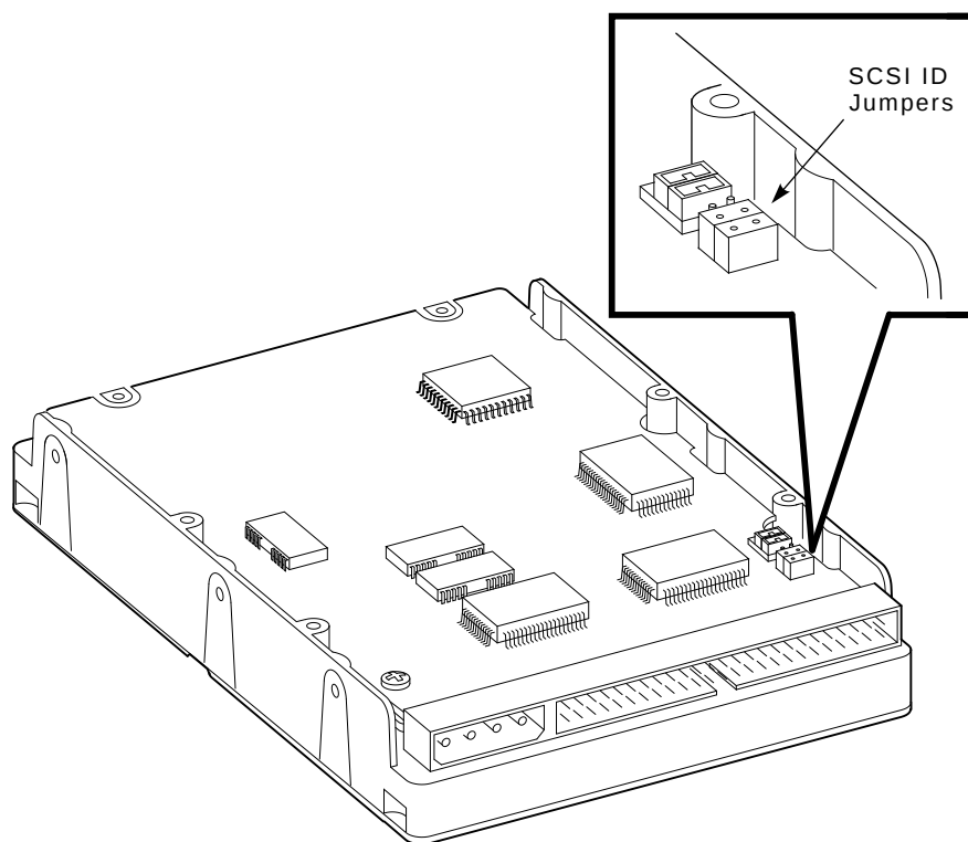
Figure 1–1 RZ24L SCSI ID Jumper Location
