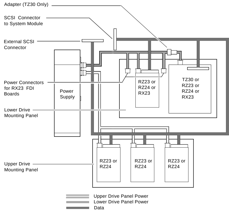
Figure 2–4 Cable Disconnections
