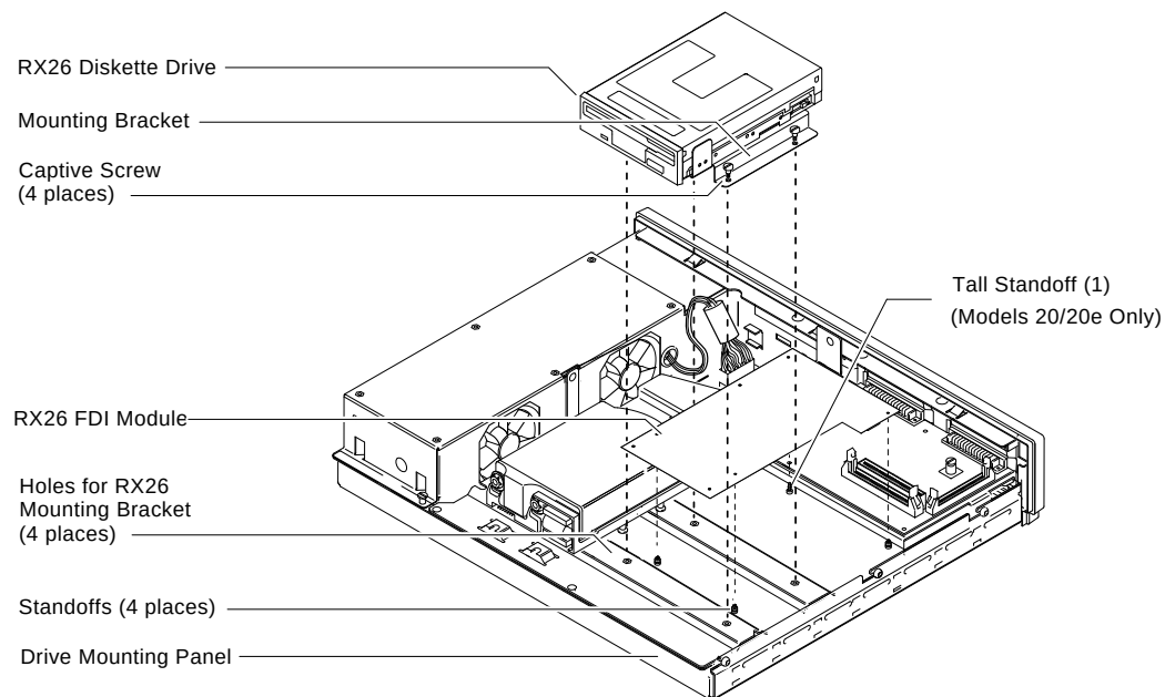
Figure RX26-4–RX26 Diskette Drive Installation
