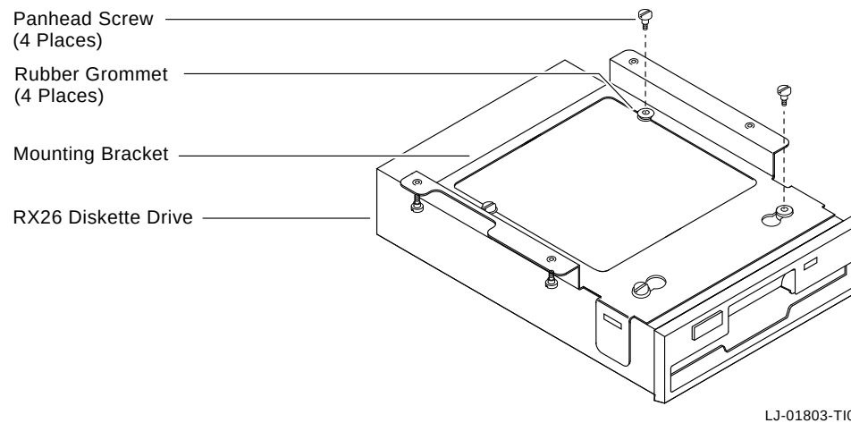
Figure RX26-3—Securing Mounting Bracket to RX26 Drive
