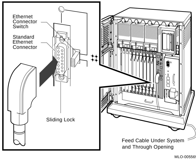
Figure 23: Making a Standard Ethernet Connection at the CPU Cover Panel
