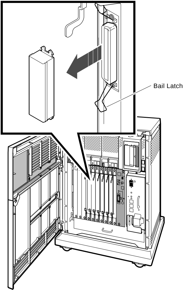
Figure 34: Removing the KZQSA Terminator
