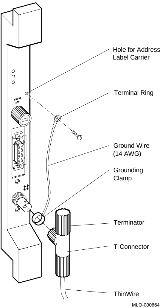
Figure 28: Grounding the ThinWire Ethernet at the DESQA Module
