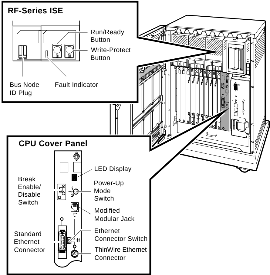
Figure 7: System Controls and Indicators — Integrated Storage Element and CPU Cover Panel
