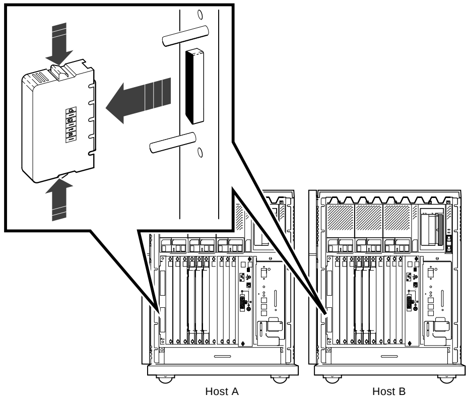
Figure 41: Removing the DSSI Terminators
