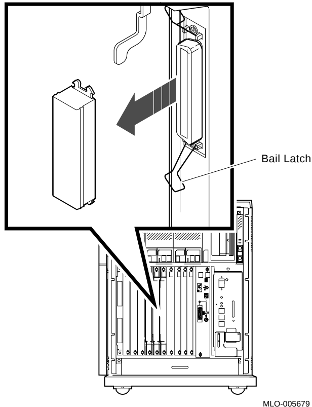
Figure 39: TLZ04/KZQSA Module Connection — Removing the Terminator
