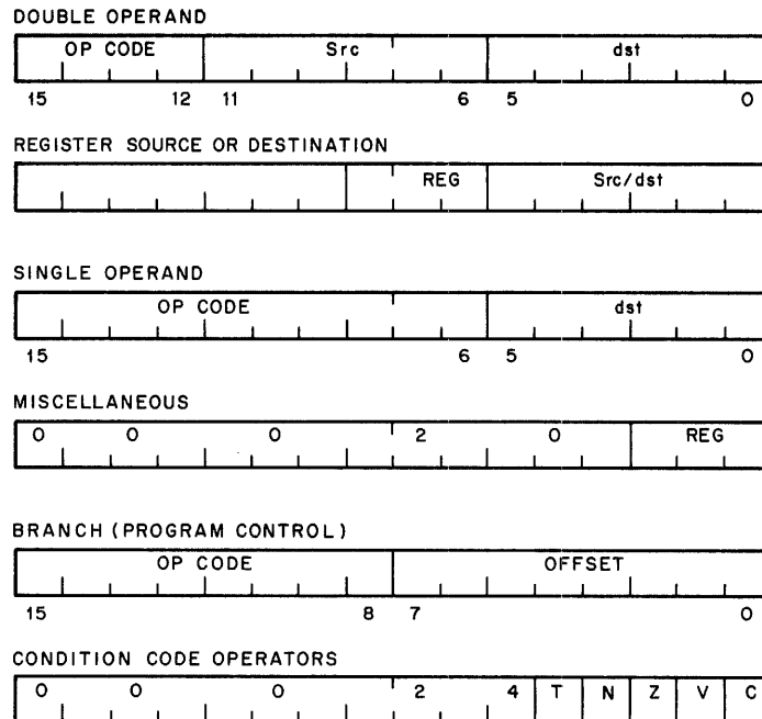
Figure 4-2 Instruction Formats
