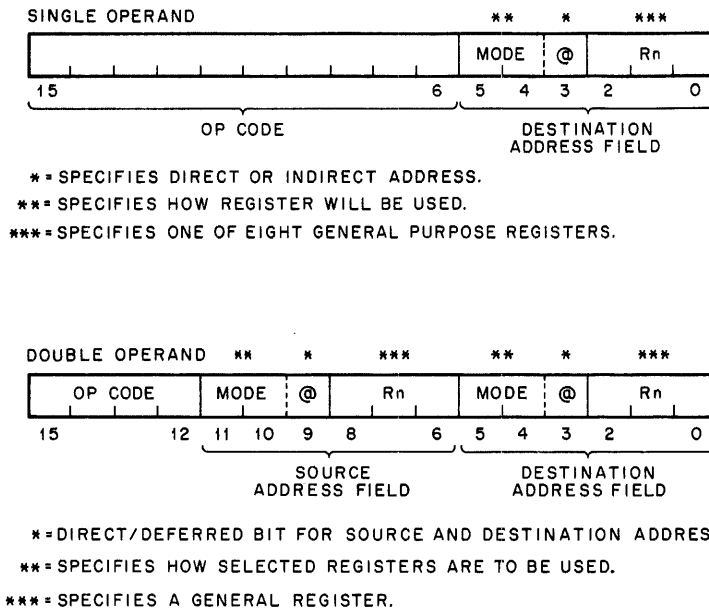
Figure 4-1 Double and Single Operand Addressing
