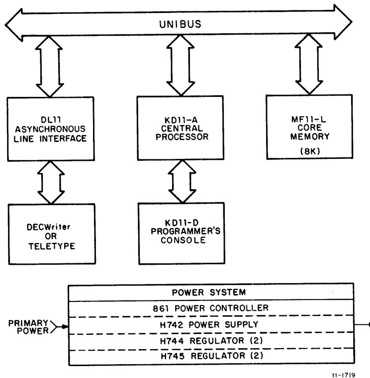
Figure 1-1 PDP-11/40 Basic System Block Diagram
