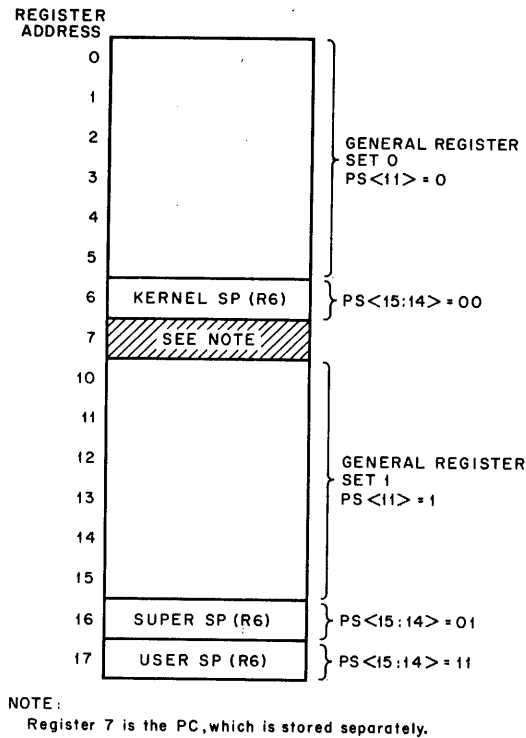
Figure 5-2 General Register Storage in GS and GD Storage Elements
