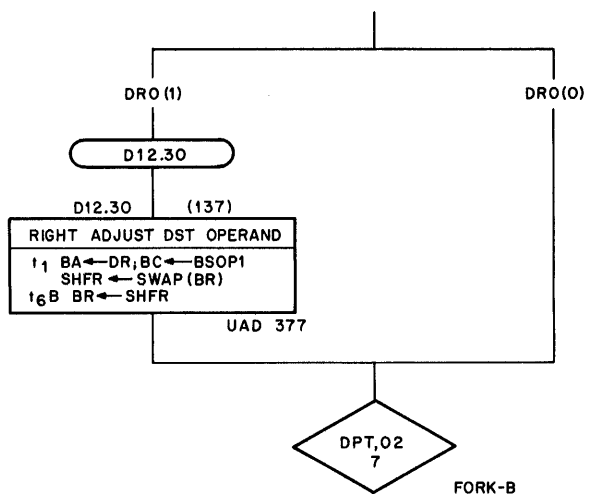
Figure 6-4 Conditional Enabling of Fork Logic
