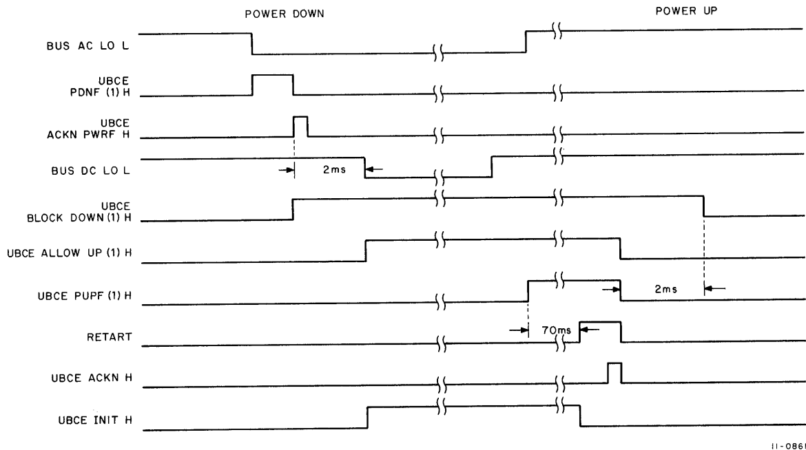
Figure 7-12 Power-Down/Power-Up Sequence
