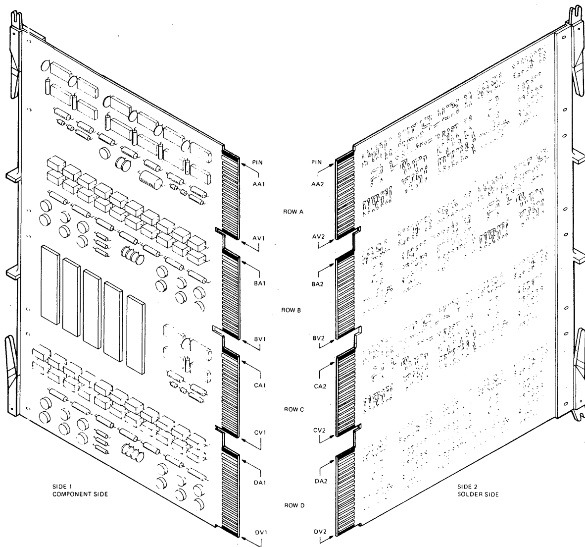
Figure 2-3 KDJ11-B Module Contacts
