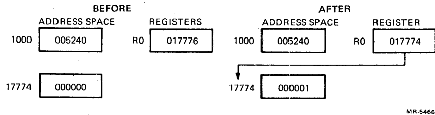
Figure 8-13 INC -(R0) Increment
