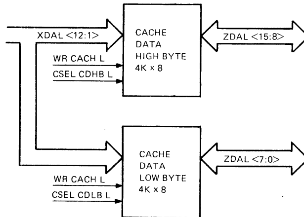
Figure 5-23 Cache Memory
