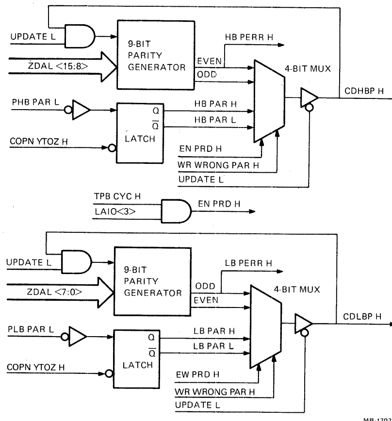
Figure 5-25 Cache Data Parity Logic
