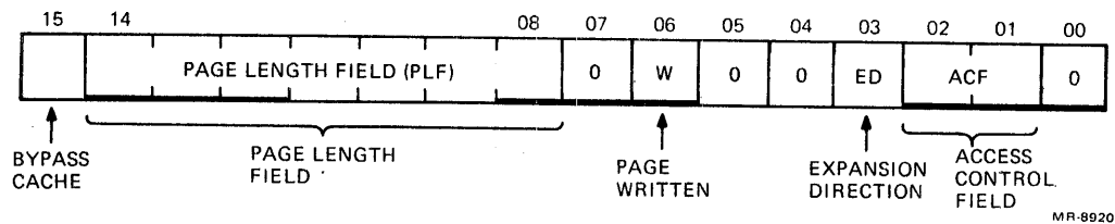
Figure 1-14 Page Descriptor Register
