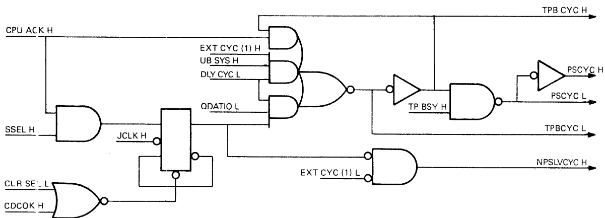
Figure 5-12 PMI Cycle Request
