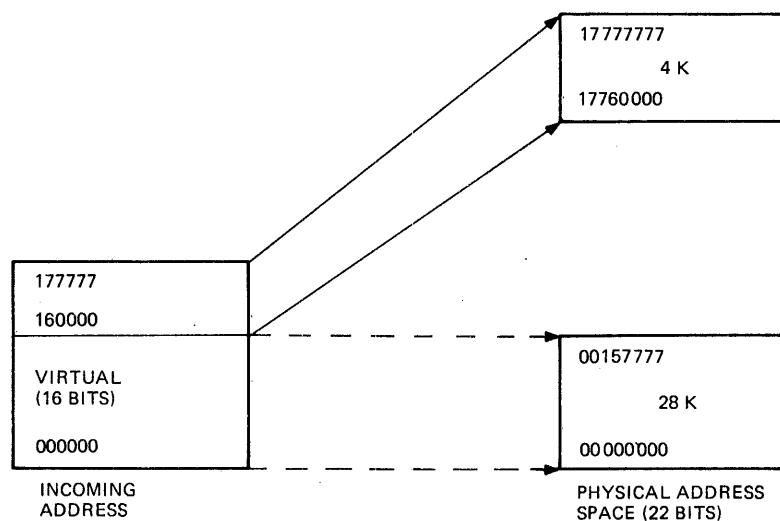
Figure 1-5 16-Bit Mapping
