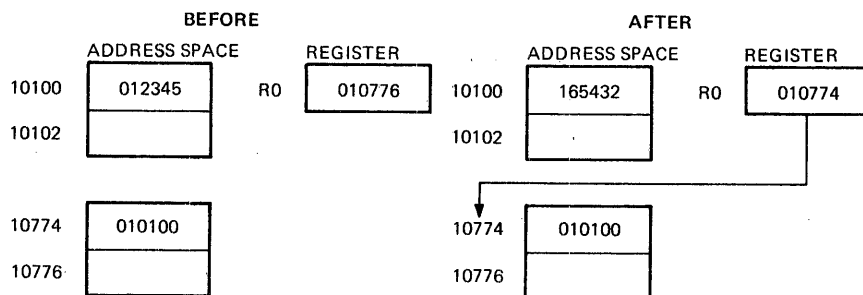
Figure 8-25 COM @-(R0) Complement
