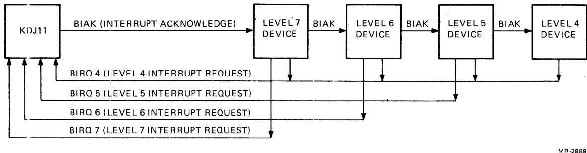
Figure 6-12 Position-Dependent Configuration
