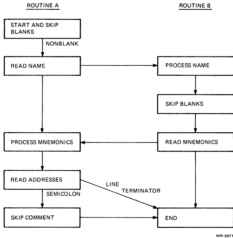
Figure 11-10 Coroutine Path
