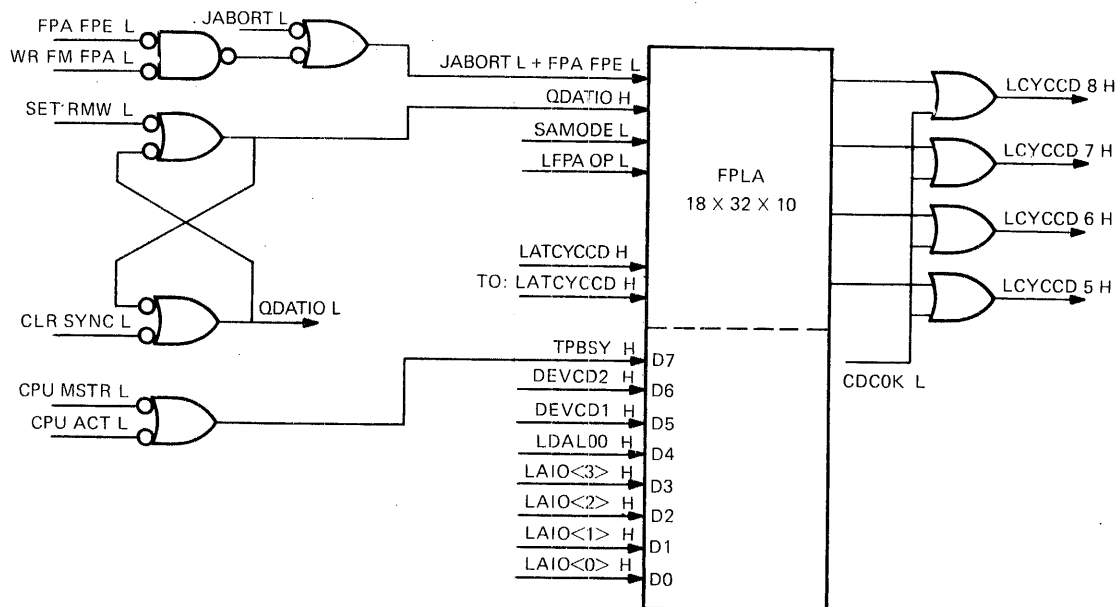
Figure 5-14 Cycle Encoder
