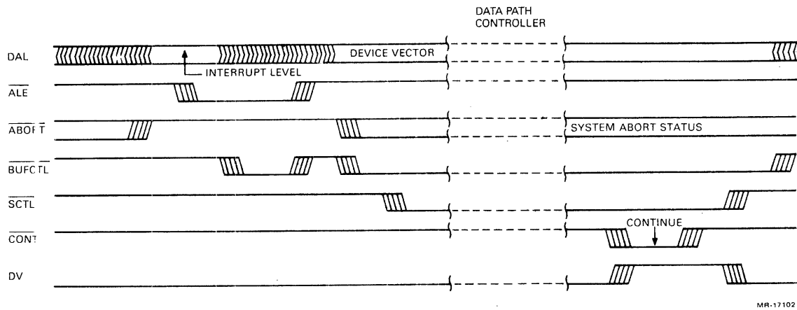
Figure 5-10 Interrupt Acknowledge Transaction
