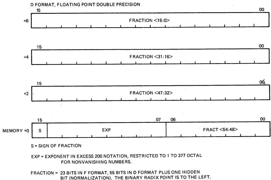
Figure 10-2 Double-Precision Format
