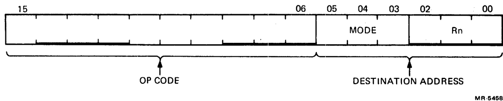
Figure 8-1 Single-Operand Addressing
