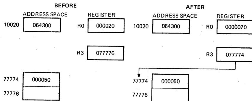
Figure 8-15 ADD -(R3),R0 Add
