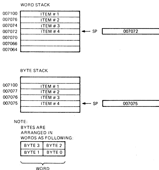
Figure 11-1 Word and Byte Stacks
