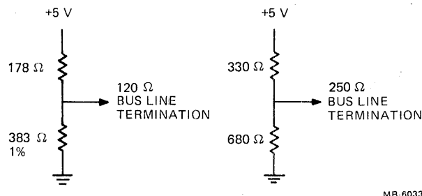
Figure 6-14 Bus Line Termination
