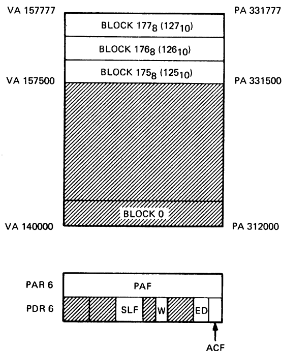
Figure 1-20 Typical Stack Memory Page
