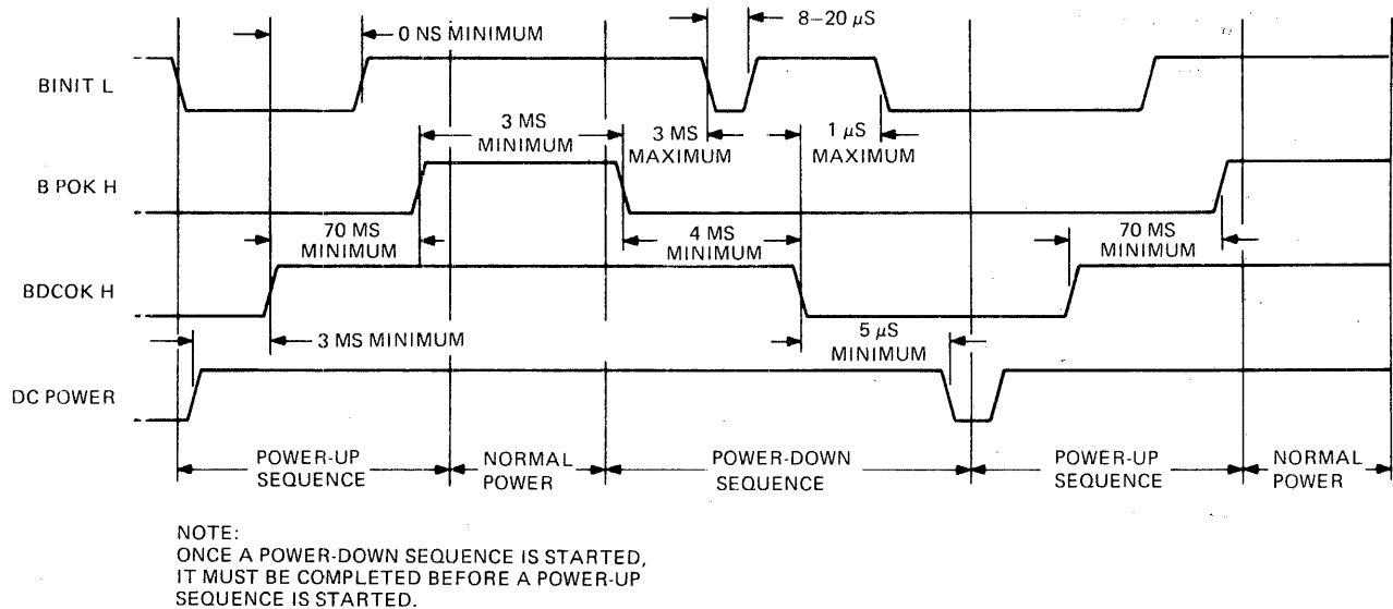
Figure 6-13 Power-Up/Power-Down Timing
