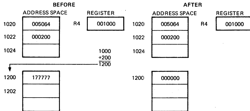
Figure 8-16 CLR 200(R4) Clear
