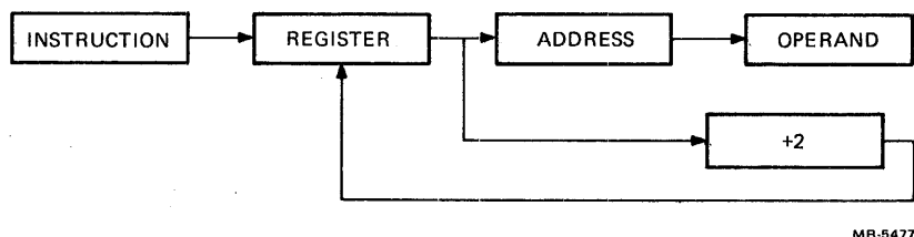
Figure 8-20 Mode 3, Autoincrement-Deferred
