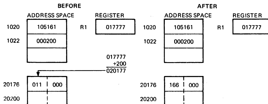
Figure 8-17 COMB 200(R1) Complement Byte
