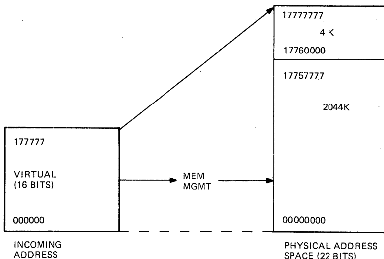
Figure 1-7 22-Bit Mapping
