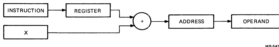
Figure 8-22 Mode 7, Index-Deferred
