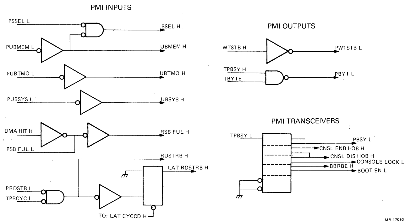
Figure 5-34 PMI Bus Control Signals
