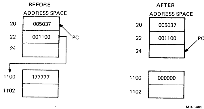
Figure 8-28 CLR @ #1100 Clear
