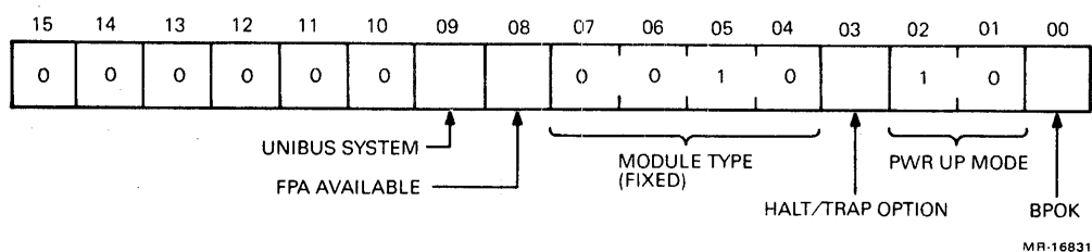
Figure 1-32 Maintenance Register
