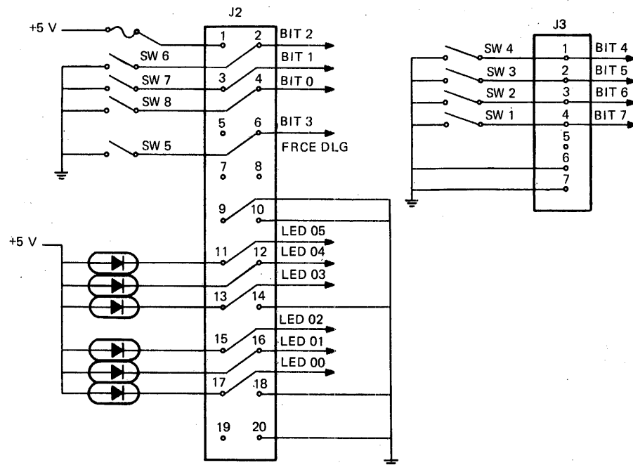
Figure 2-2 Pin Assignments for Connectors J2 and J3
