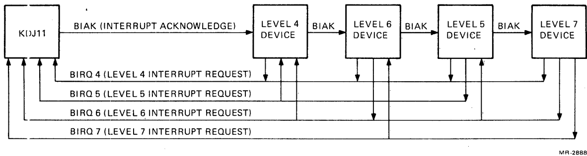
Figure 6-11 Position-Independent Configuration
