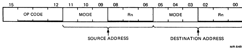
Figure 8-2 Double-Operand Addressing
