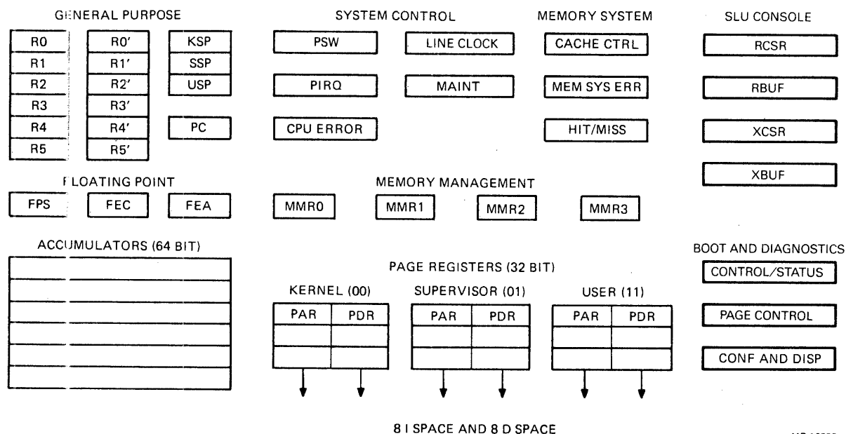
Figure 1-1 Programming Model
