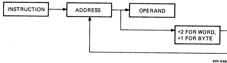
Figure 8-4 Mode 2, Autoincrement
