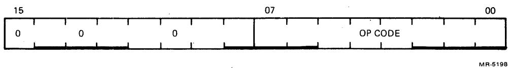
Figure 9-13 Operate Group
