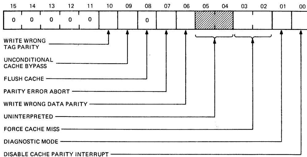
Figure 1-23 Cache Control Register (CCR)
