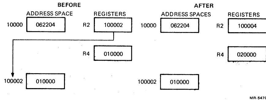
Figure 8-12 ADD (R2)+,R4 Add
