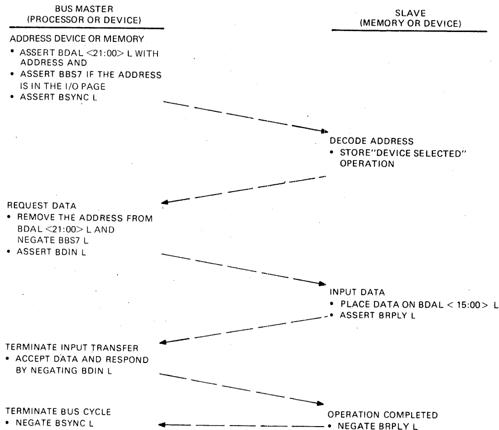
Figure 6-1 DATI Bus Cycle
