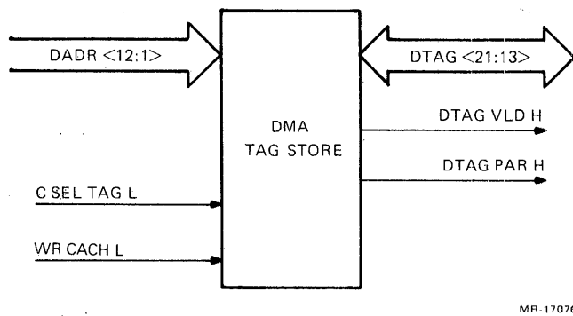
Figure 5-27 DMA Tag Store
