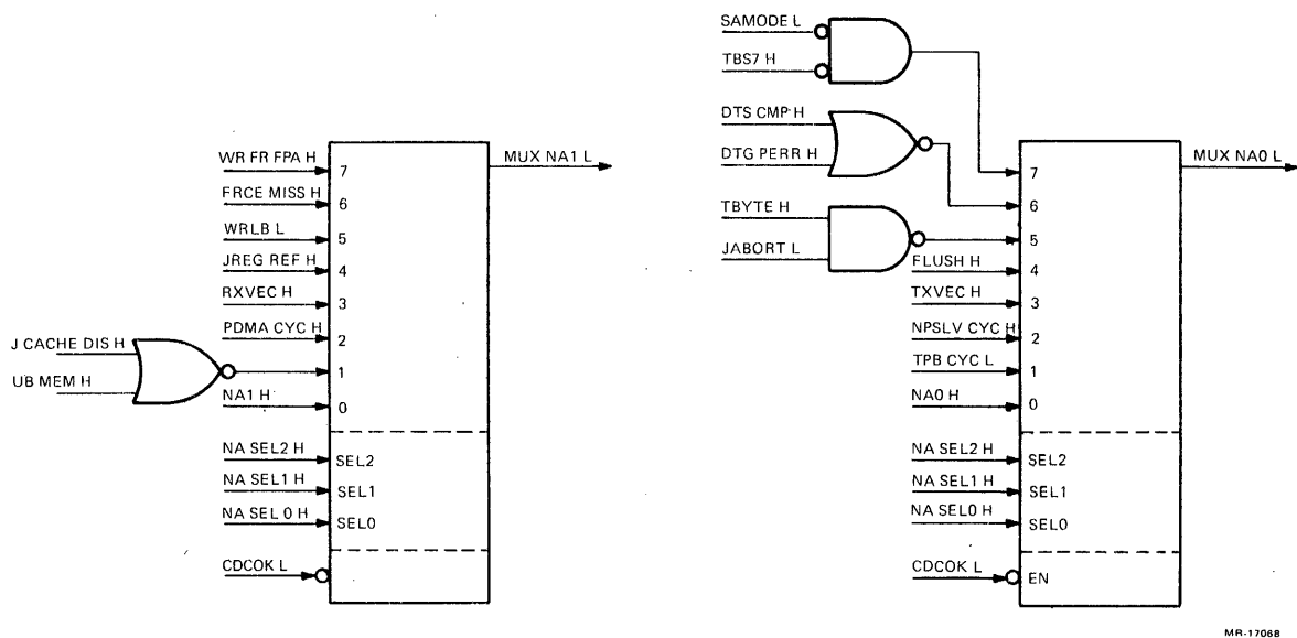
Figure 5-17 Next Address Multiplexer
