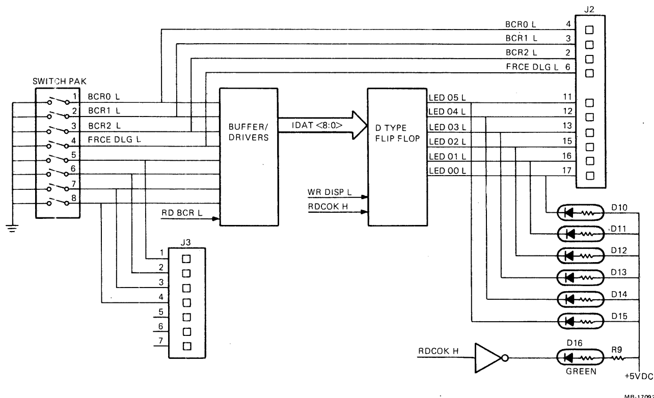
Figure 5-37 Configuration and Display Circuits
