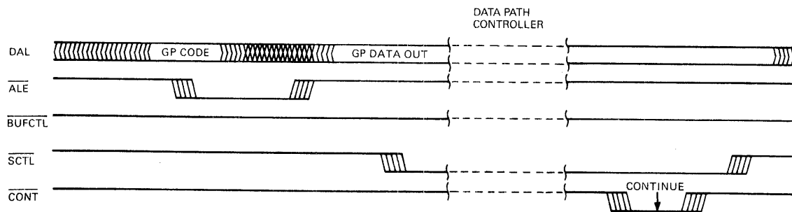
Figure 5-9 General Purpose Write Transaction
