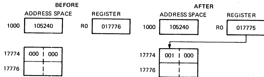
Figure 8-14 INCB -(R0) Increment Byte
