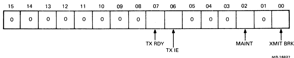
Figure 1-28 Transmitter Control/Status Register
