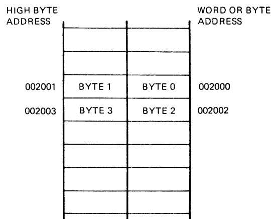
Figure 9-16 Byte Instructions
