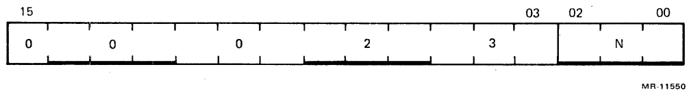
Figure 9-12 Set Priority Level
