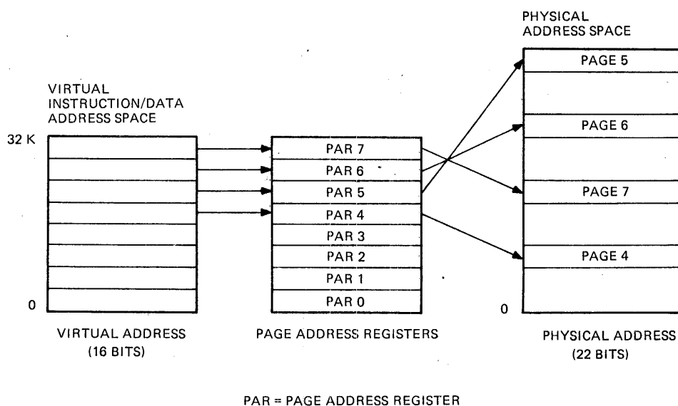
Figure 1-8 Virtual Address Mapping into Physical Address
