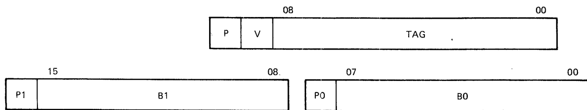
Figure 5-22 Cache Data Format
