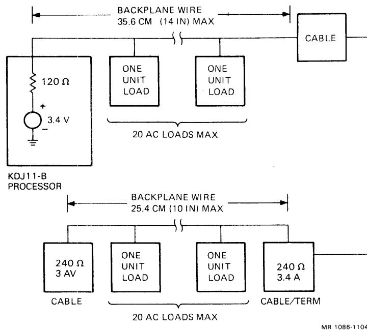
Figure 6-16 Multiple-Backplane Configuration
