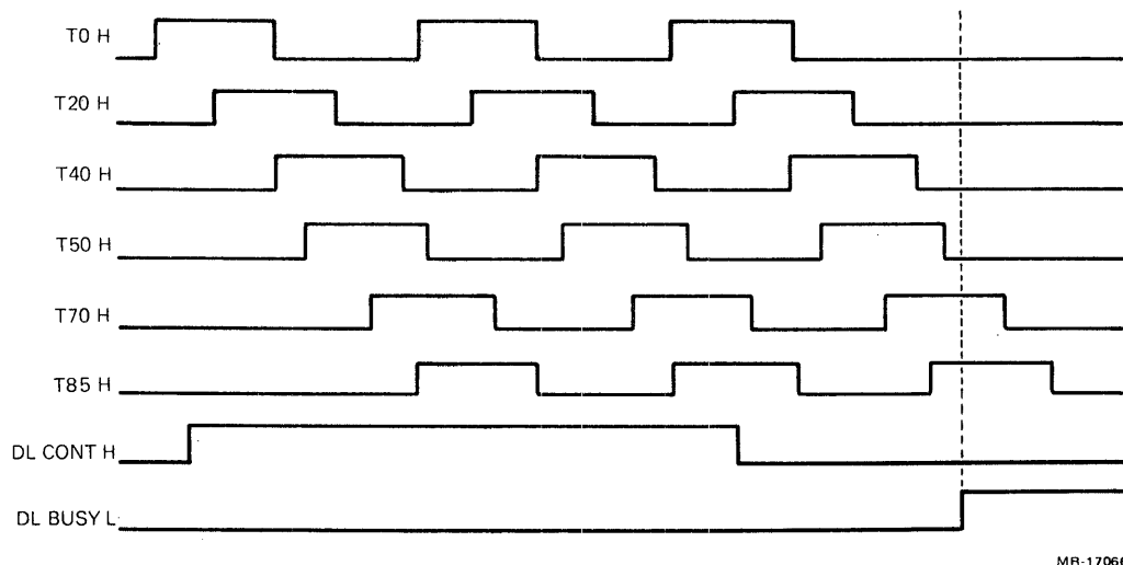
Figure 5-15 Oscillator Outputs
