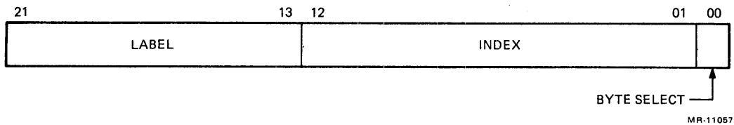
Figure 1-21 Cache Physical Address
