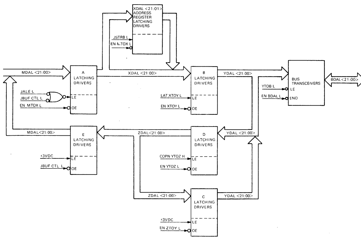
Figure 5-32 Internal Bus Control
