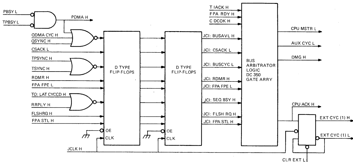
Figure 5-11 Bus Arbitrator
