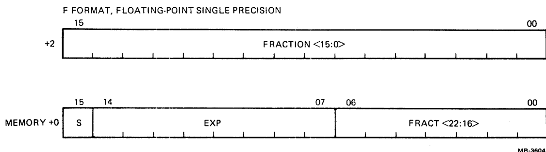
Figure 10-1 Single-Precision Format
