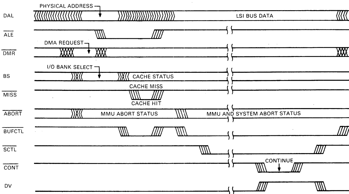
Figure 5-6 Stretched Bus Read Transaction
