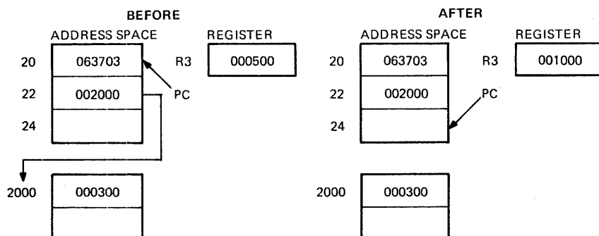
Figure 8-29 ADD @ #2000 Add
