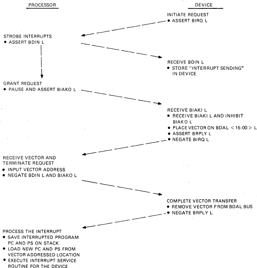
Figure 6-9 Interrupt Request/Acknowledge Sequence
