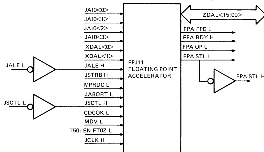
Figure 5-40 Floating-Point Accelerator
