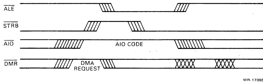
Figure 5-3 NOP Transaction
