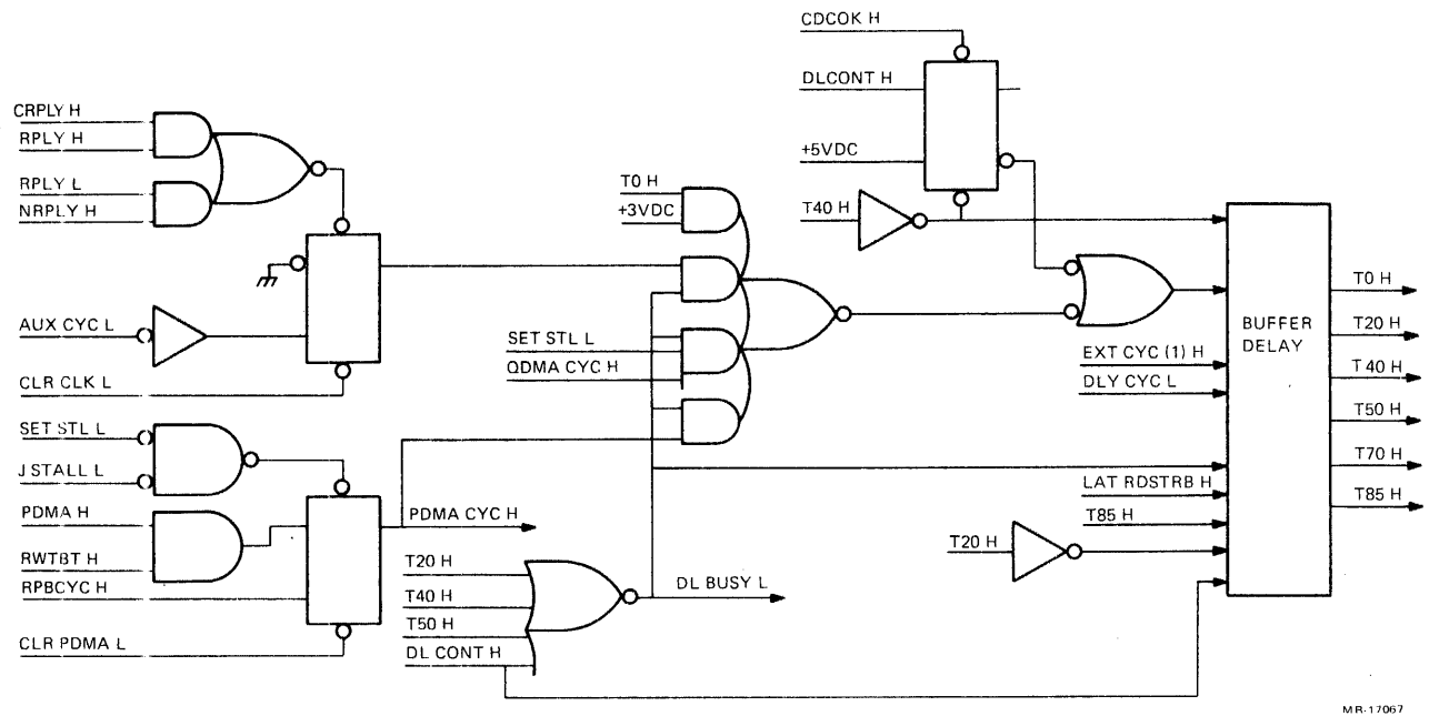
Figure 5- 6 Oscillator Control
