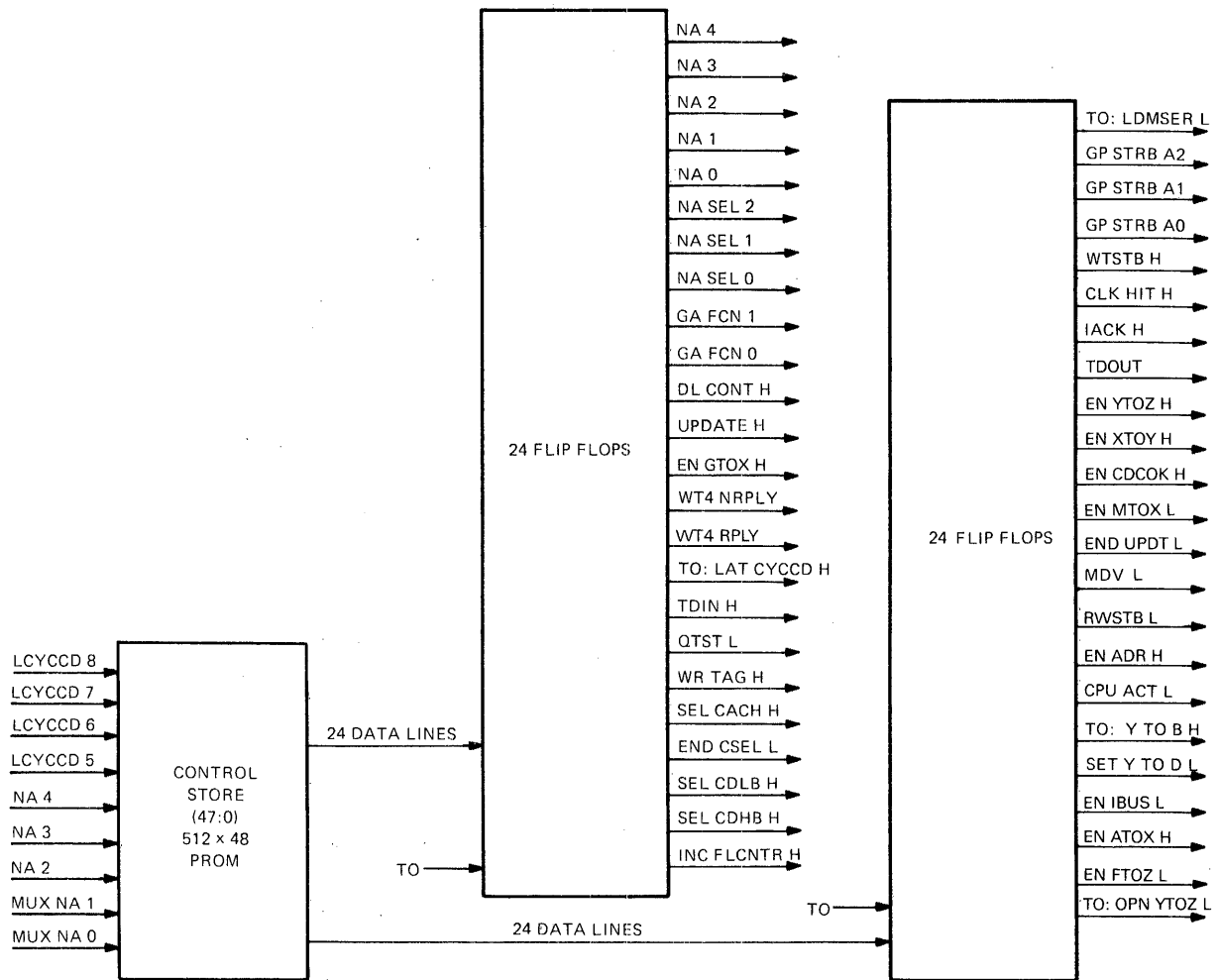
Figure 5-18 Control Store
