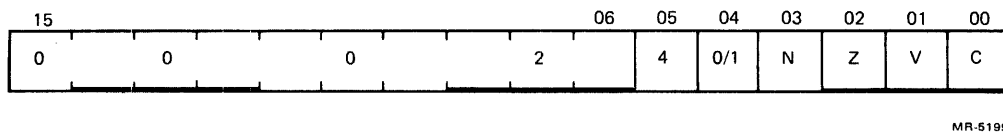
Figure 9-14 Condition Group
