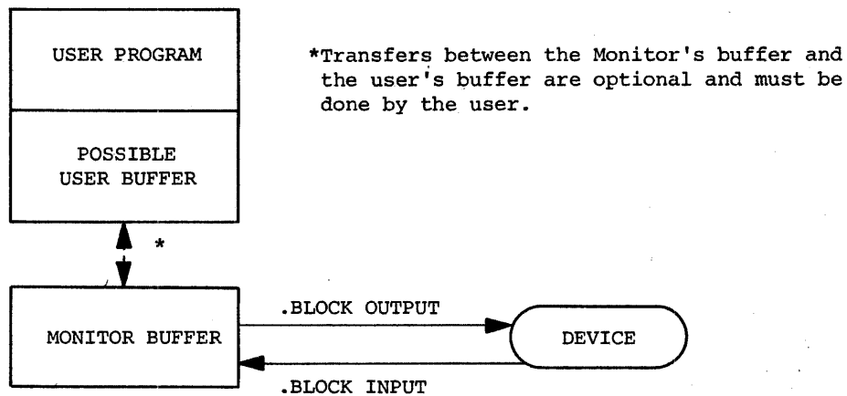
Figure 3-4a The Transfer Path
