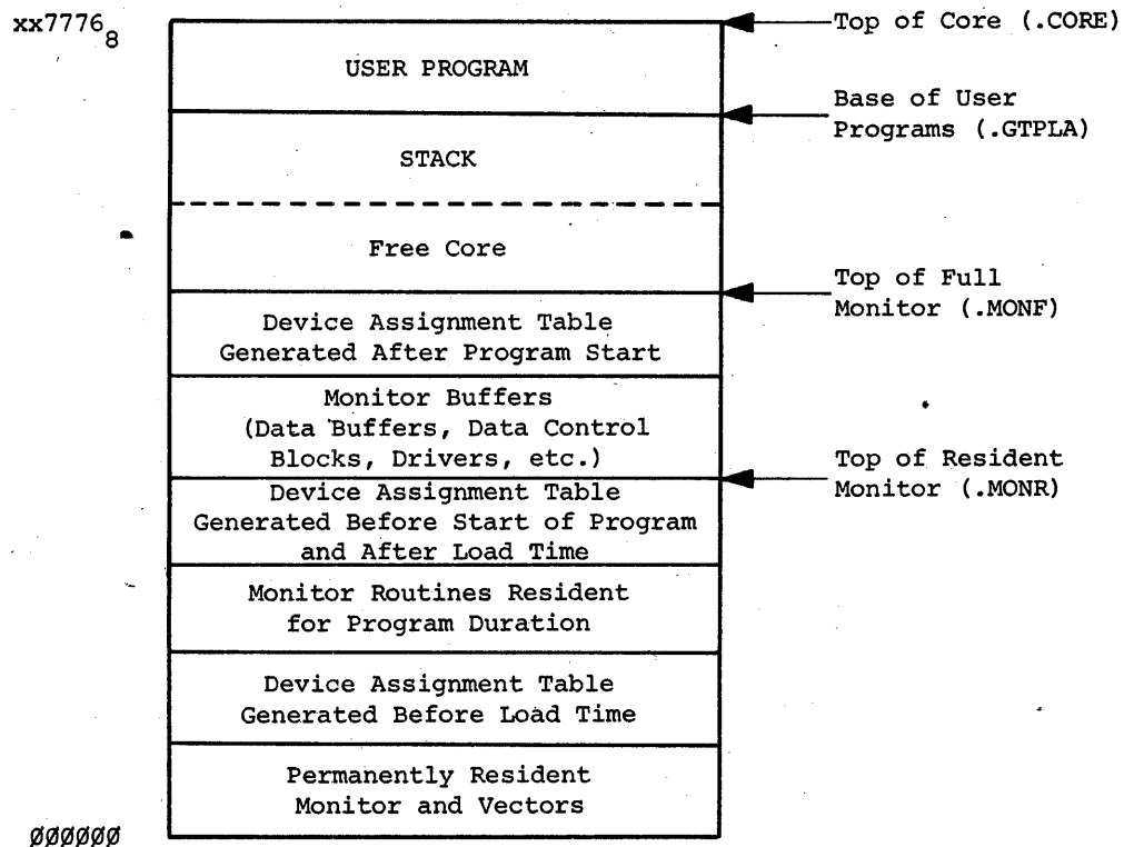
Figure 3-1 The Monitor Core Map
