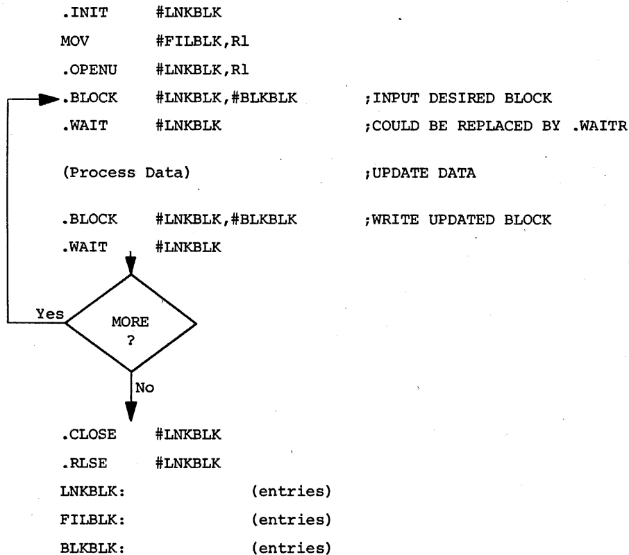
Figure 3-4b The Sequence of Requests for .BLOCK
