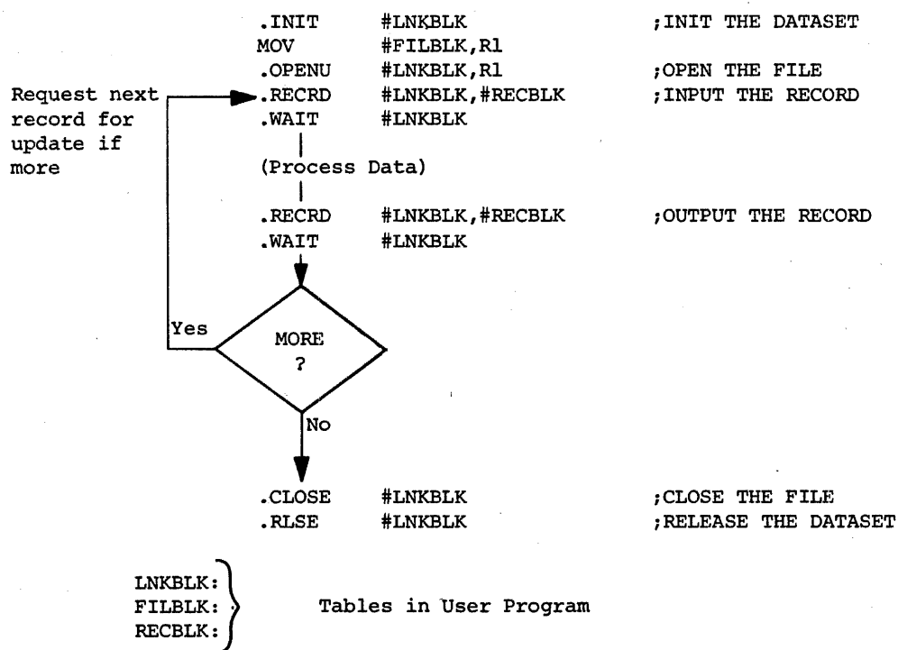
Figure 3-3b Sequence of Requests for .RECRD
