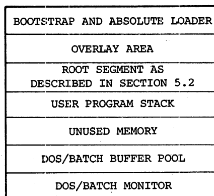
Figure 9-10 Overall Memory Allocation
