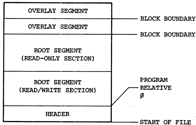
Figure 9-15 Overlay Disk Format
