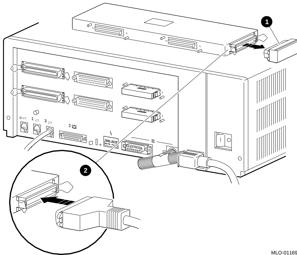
Figure B–5 SCSI Cable Ports
