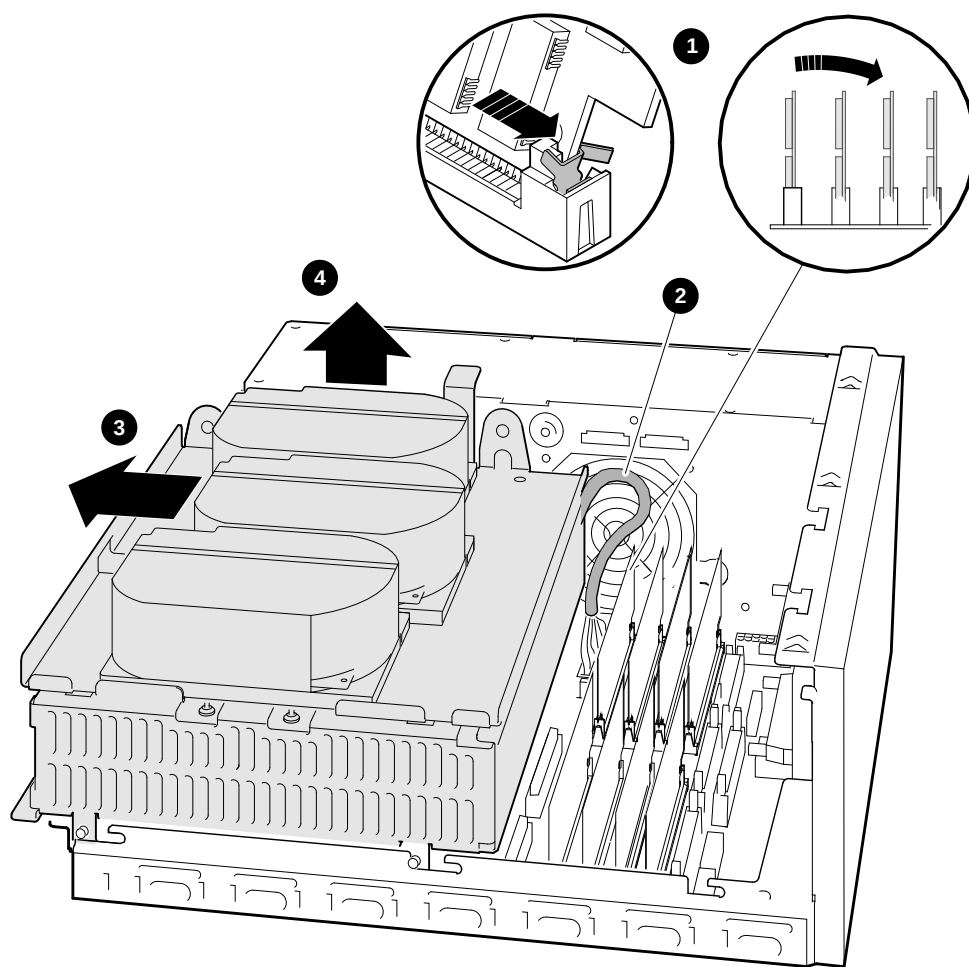
Figure 1-13 Disconnecting the Internal SCSI Cable
