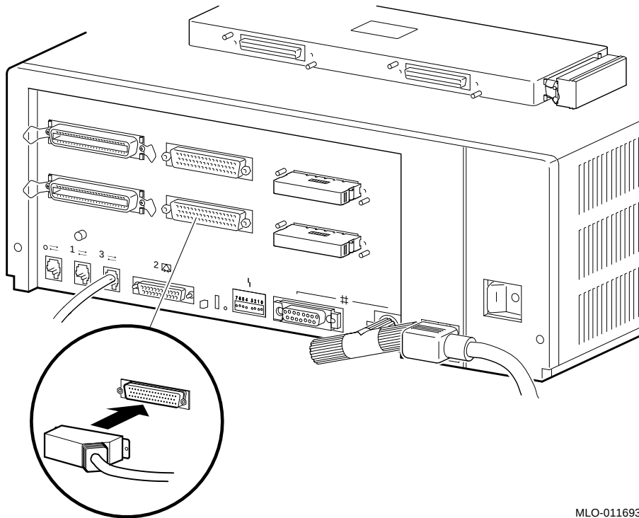
Figure B-4 Connecting a Peripheral Cable to Synchronous Port 0 and 1, and to the Modem Port
