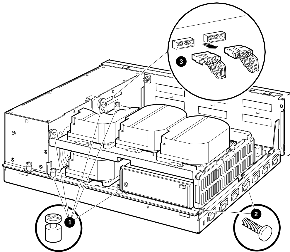
Figure 1-11 Disconnecting the Internal Power Cables
