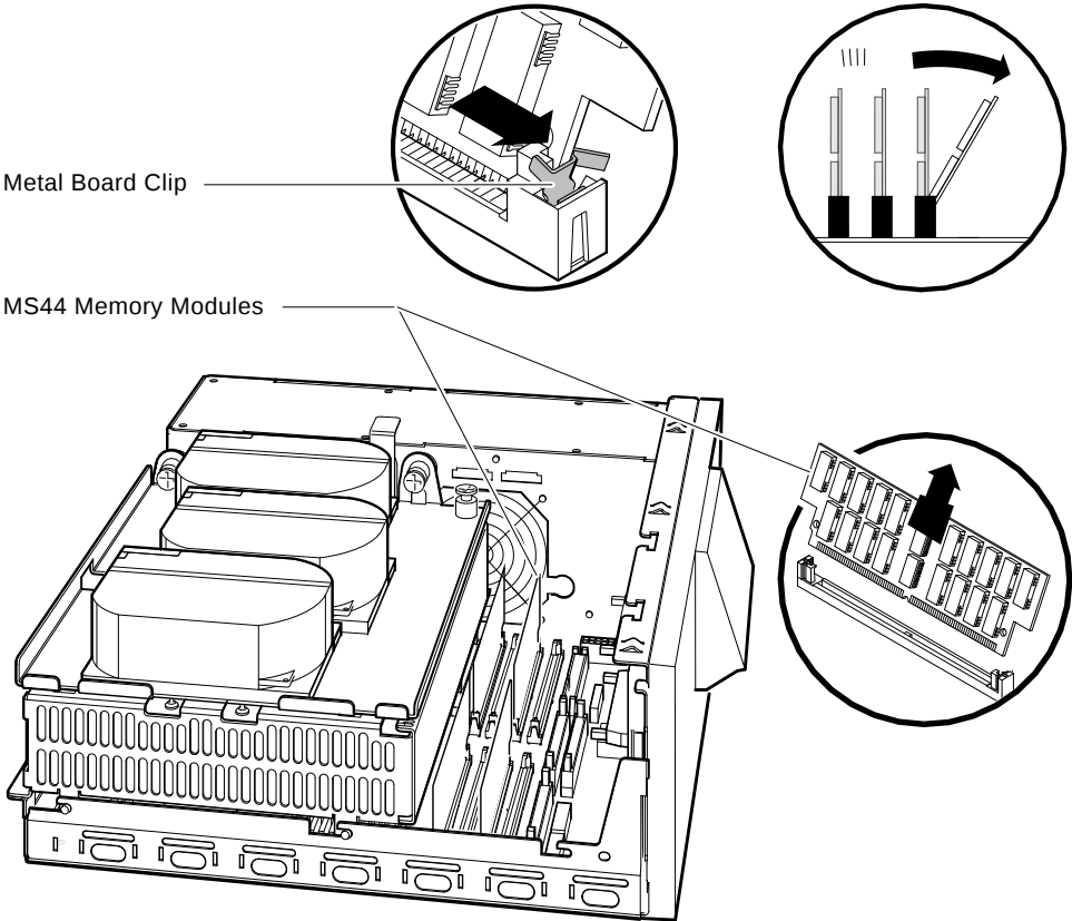
Figure 4-18 Removing a SIMM
