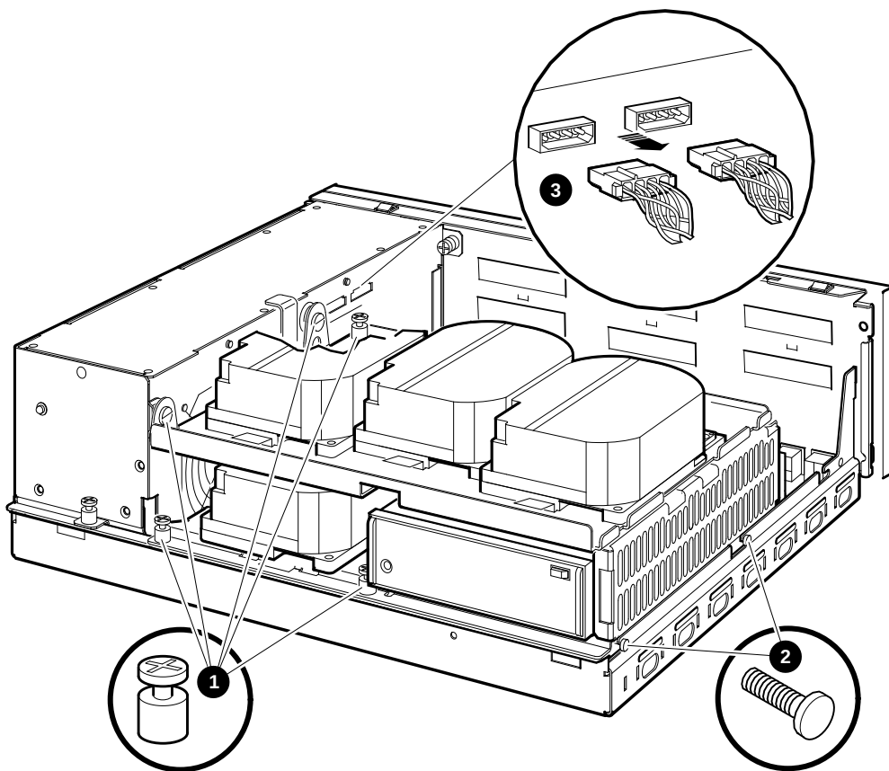
Figure 4-13 Disconnecting the Internal Power Cables
