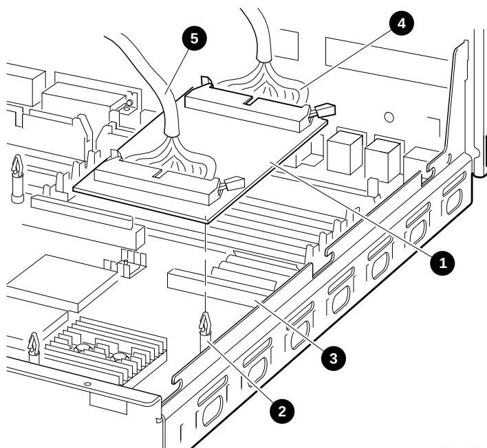
Figure C-7 Installing the Dual DSSI Card
