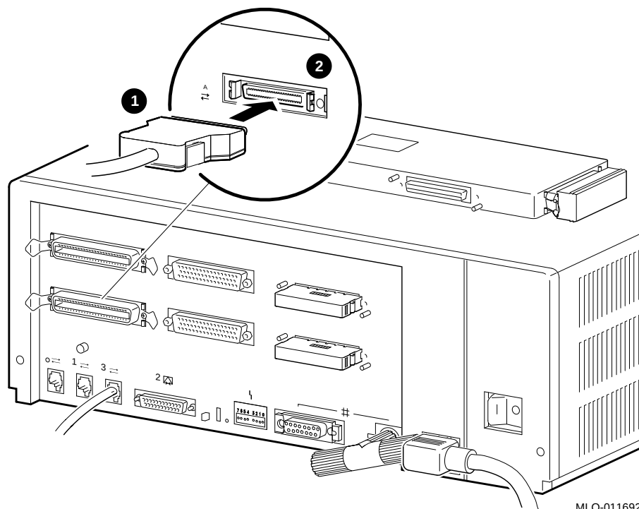
Figure B-3 Connecting a Peripheral Cable to Asynchronous Port A (DHW42-CA)
