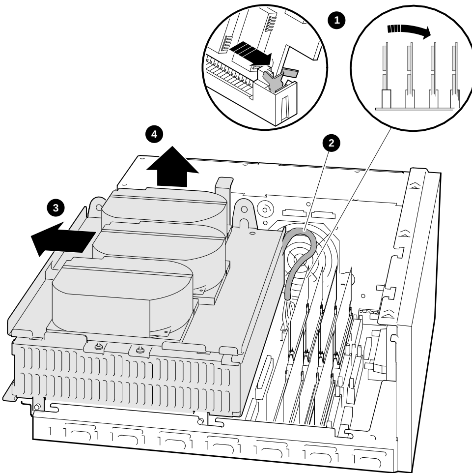
Figure C-5 Disconnecting the Internal SCSI Cable
