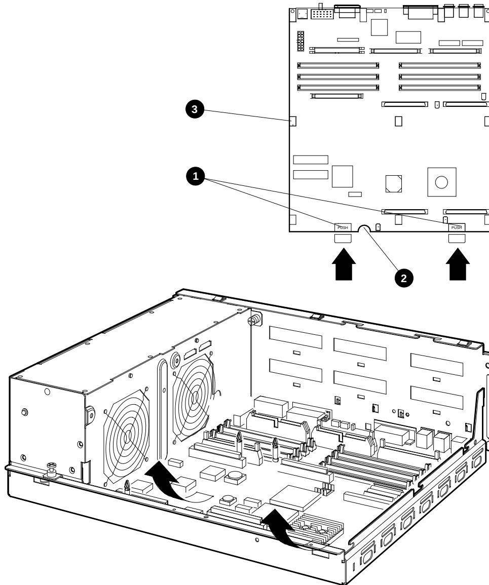
Figure 4-19 Removing the CPU Module
