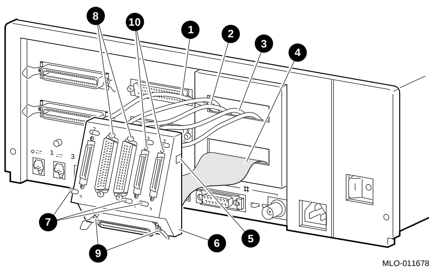
Figure 1-8 VAX 4000-10xx Port Cover
