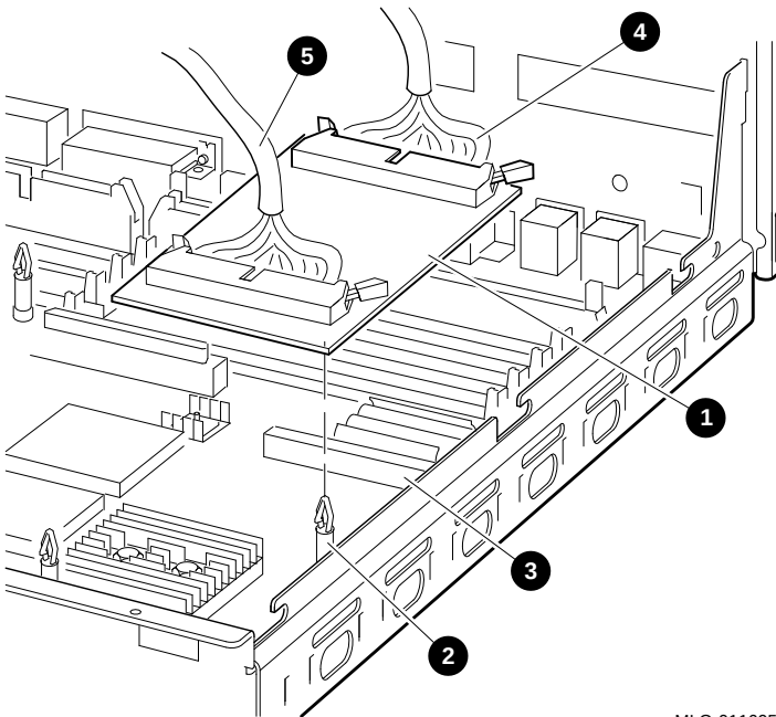
Figure 1-15 Installing the Dual DSSI Card
