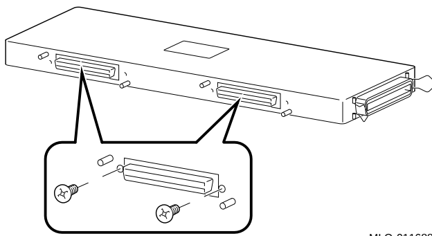
Figure 4-4 Removing and Installing the Two DSSI External Bus Connectors
