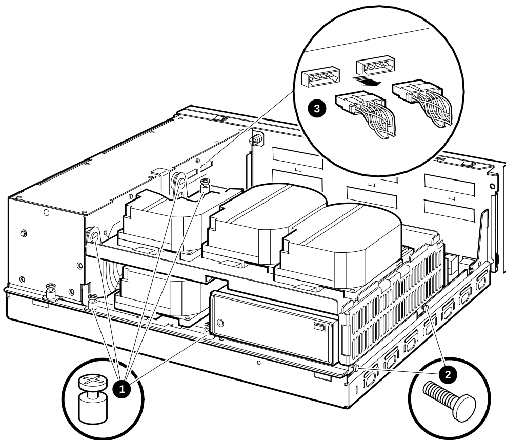
Figure 4-8 Disconnecting the Internal Power Cables
