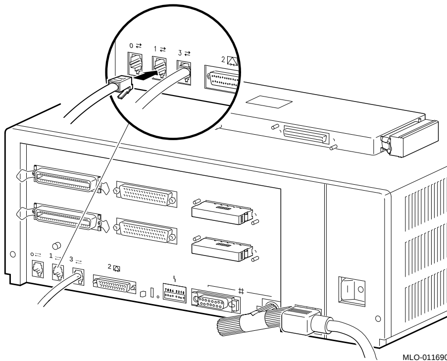
Figure B-1 Connecting a Peripheral Cable to MMJ Port 0 and 1
