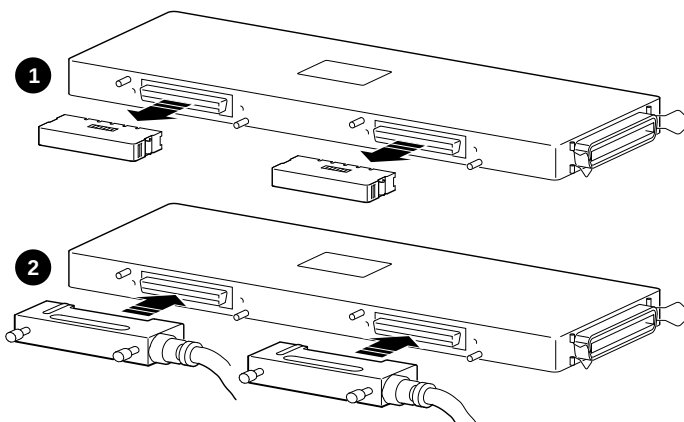
Figure B–8 DSSI Cable Ports
