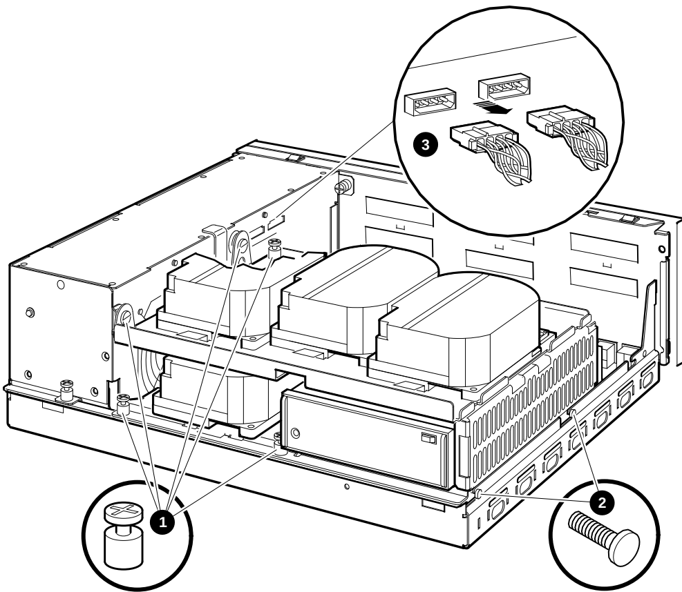
Figure C-3 Disconnecting the Internal Power Cables
