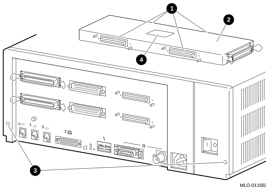
Figure 4-3 Removing the Rackmount Enclosure Cover
