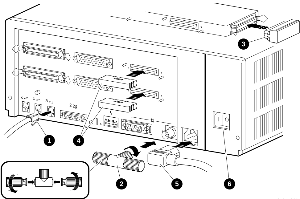
Figure 1-23 Making Console Connections
