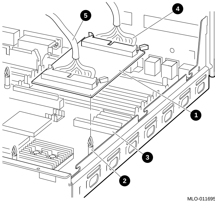
Figure 4-17 Installing the Dual DSSI Card
