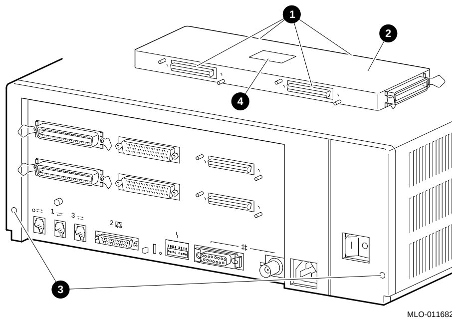
Figure 1-16 Installing New Rackmount Top Cover
