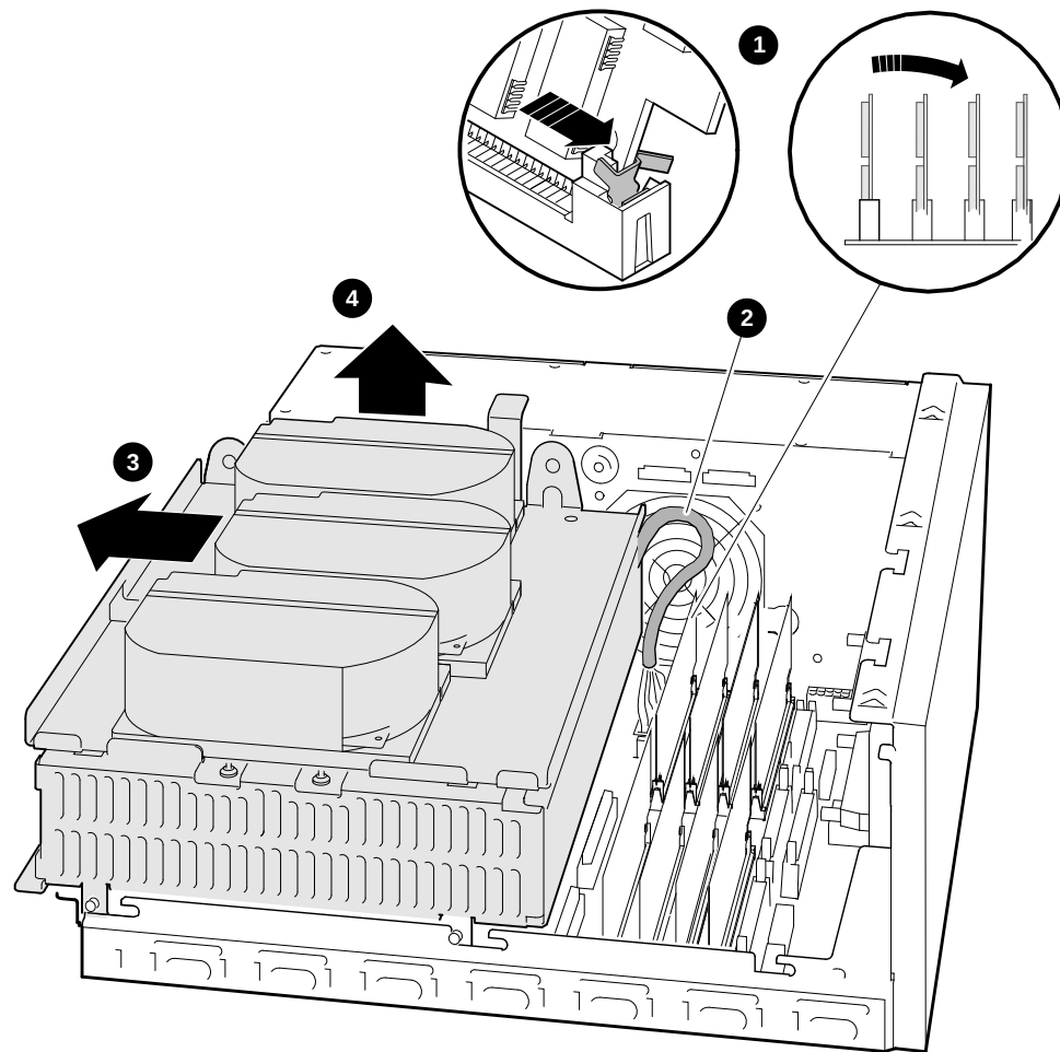
Figure 4-10 Disconnecting the Internal SCSI Cable
