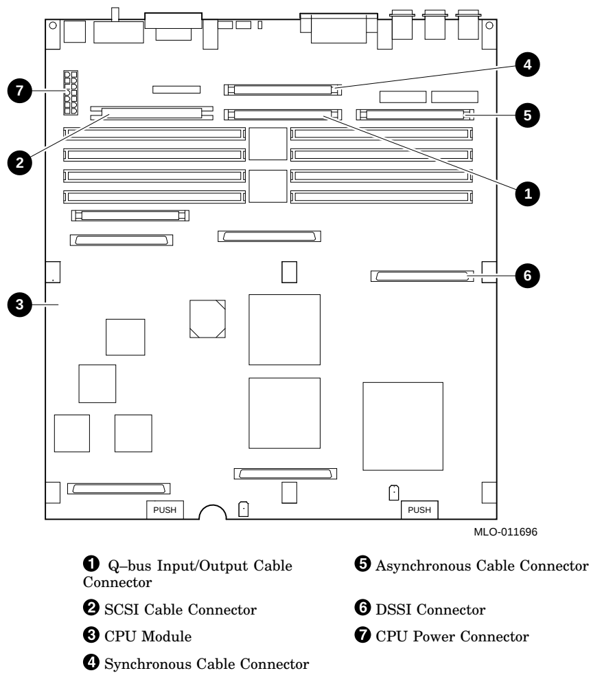
Figure 4-5 Internal Connectors
