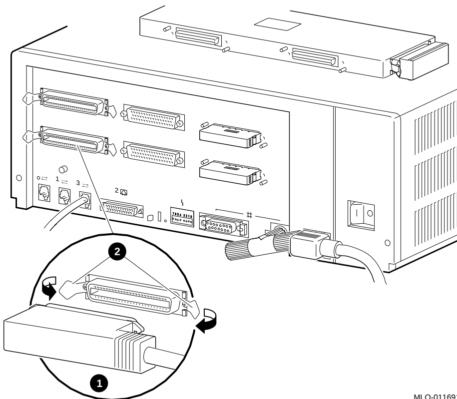
Figure B-2 Connecting a Peripheral Cable to Asynchronous Port A
