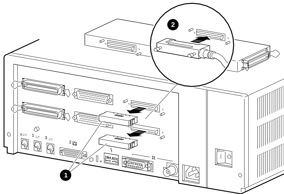
Figure B–6 DSSI Cable Ports
