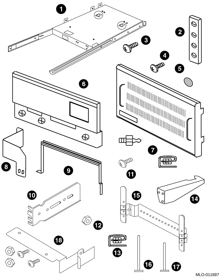
Figure 1-2 RM 4000-10xx Shelf Kit Contents (P/N 70-30949-01)
