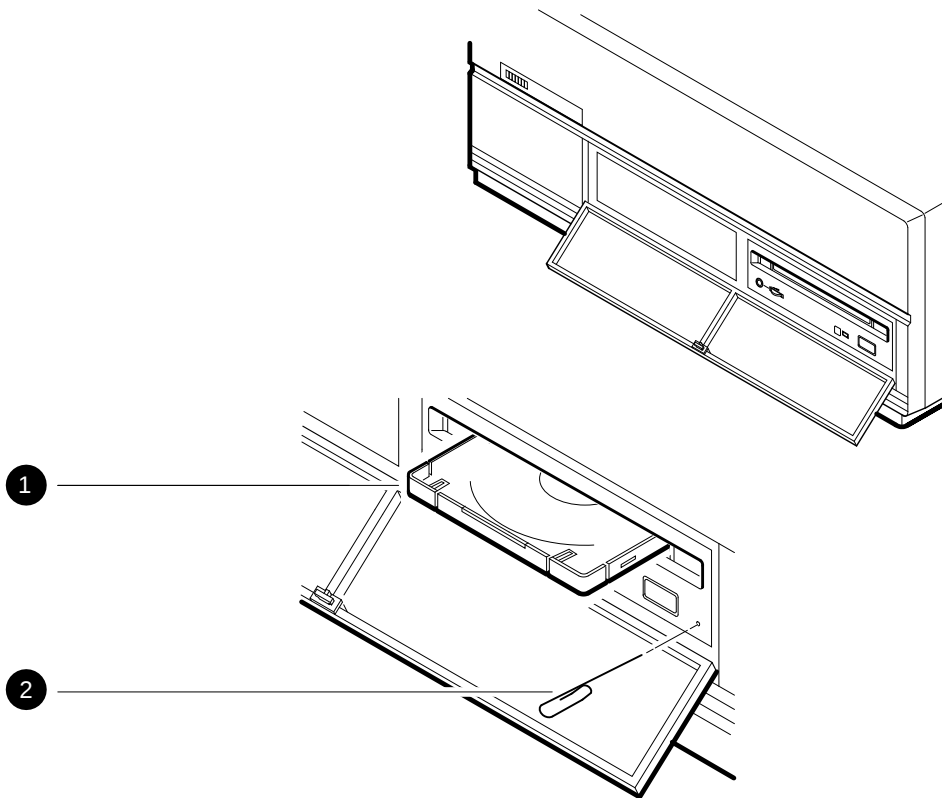
Figure 2-17 Removing Caddy Manually
