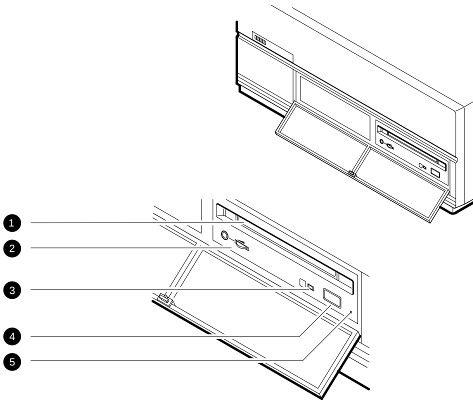
Figure 2–11 RRD42 Compact Disc Drive Front Panel
