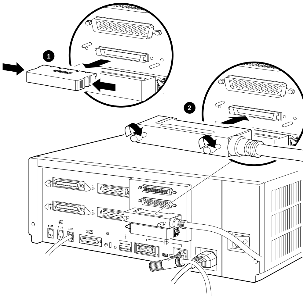
Figure 3-8 Connecting a DSSI Cable
