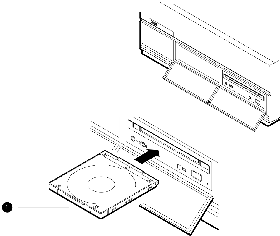
Figure 2–15 Inserting Caddy with Disc into RRD42
