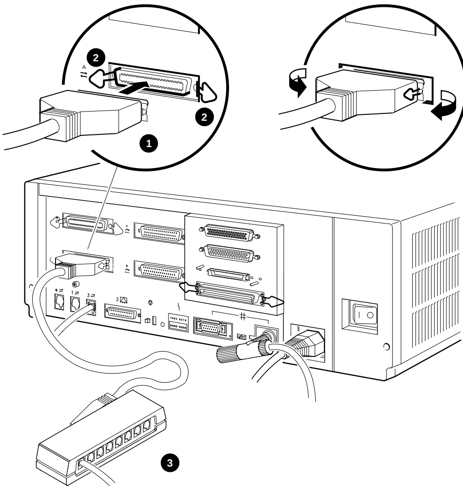
Figure 4-6 Connecting a Peripheral to Asynchronous Port A
