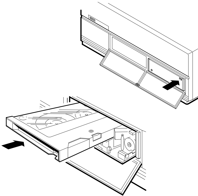
Figure 2-6 Inserting a QIC Tape
