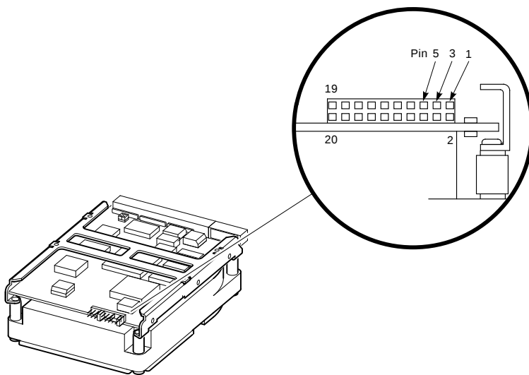
Figure C-1 Setting the DSSI Node ID on an RF31T or an RF35
