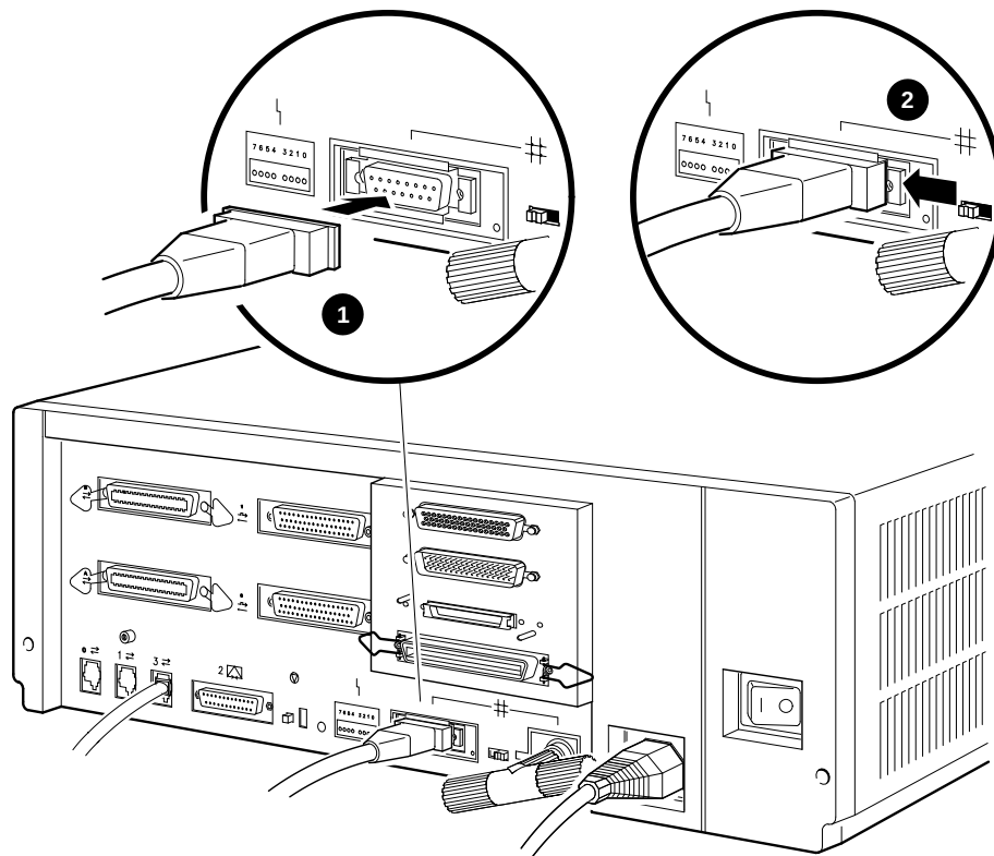
Figure 3-5 Connecting a Transceiver Cable
