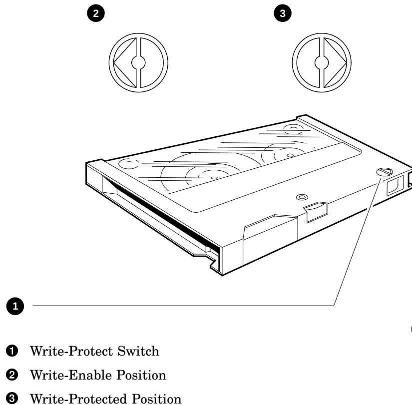
Figure B–5 QIC Tape Write-Protect Switch
