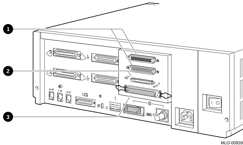
Figure 1-2 VAX 4000 Model 100 Expansion Ports
