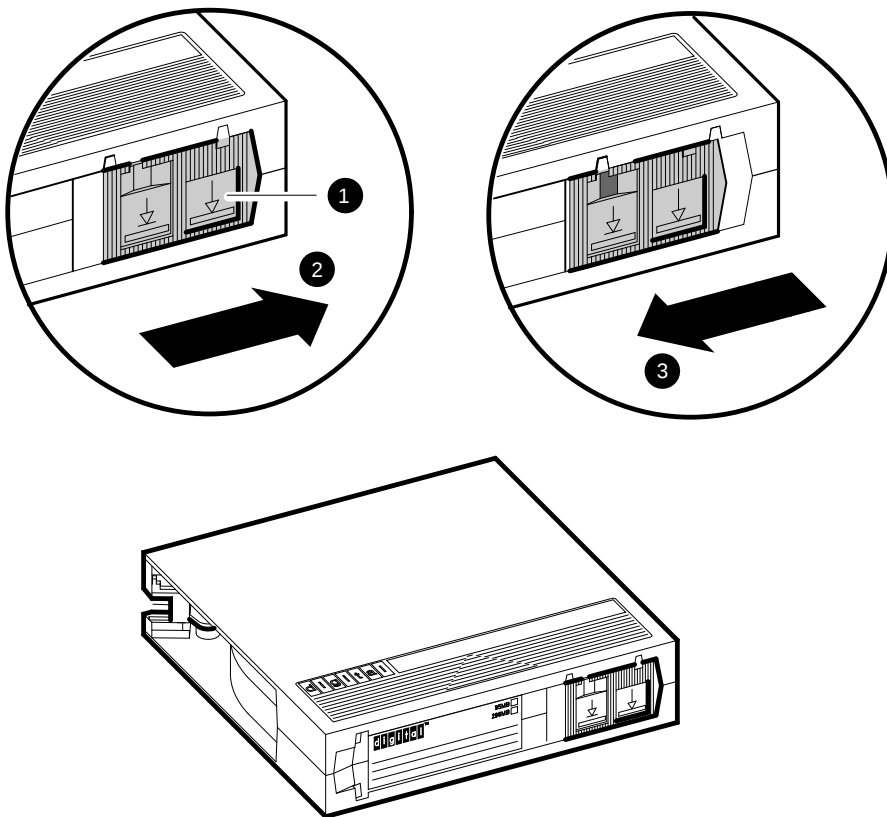
Figure B-3 Write-Protect Switch Positions
