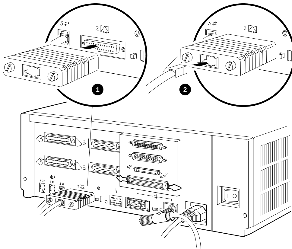
Figure 4-5 Connecting a Peripheral to the Asynchronous Modem Control Port Using an EIA-232 to DEC423 Adapter
