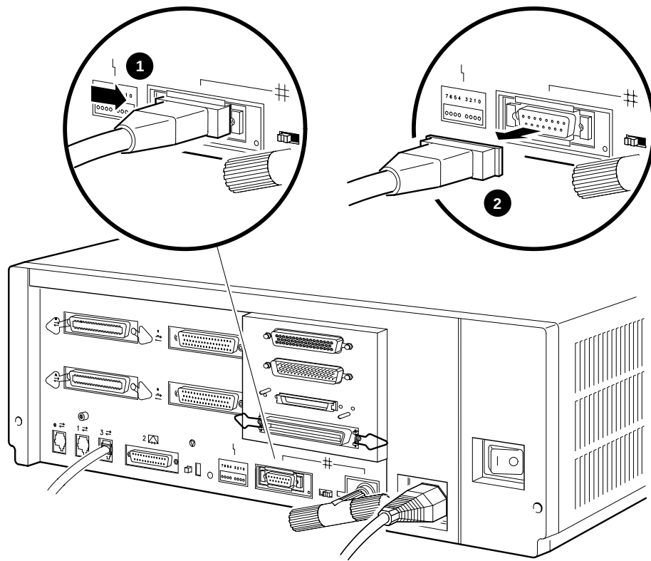
Figure 3-7 Disconnecting the System Unit from a Transceiver Cable
