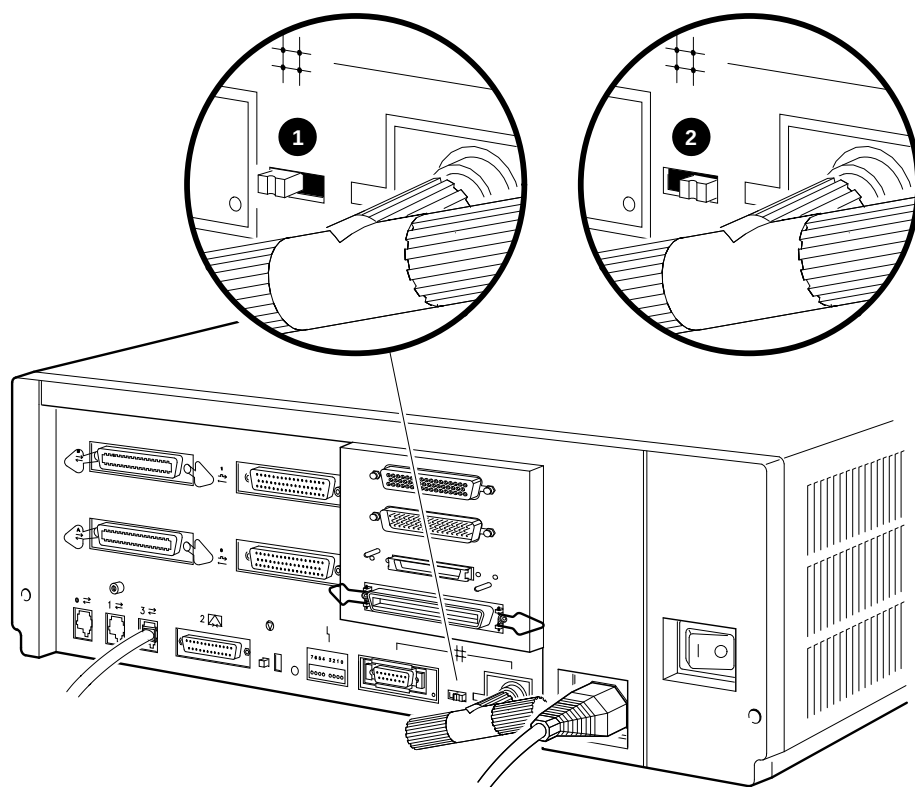
Figure 3-1 Network Select Switch Positions
