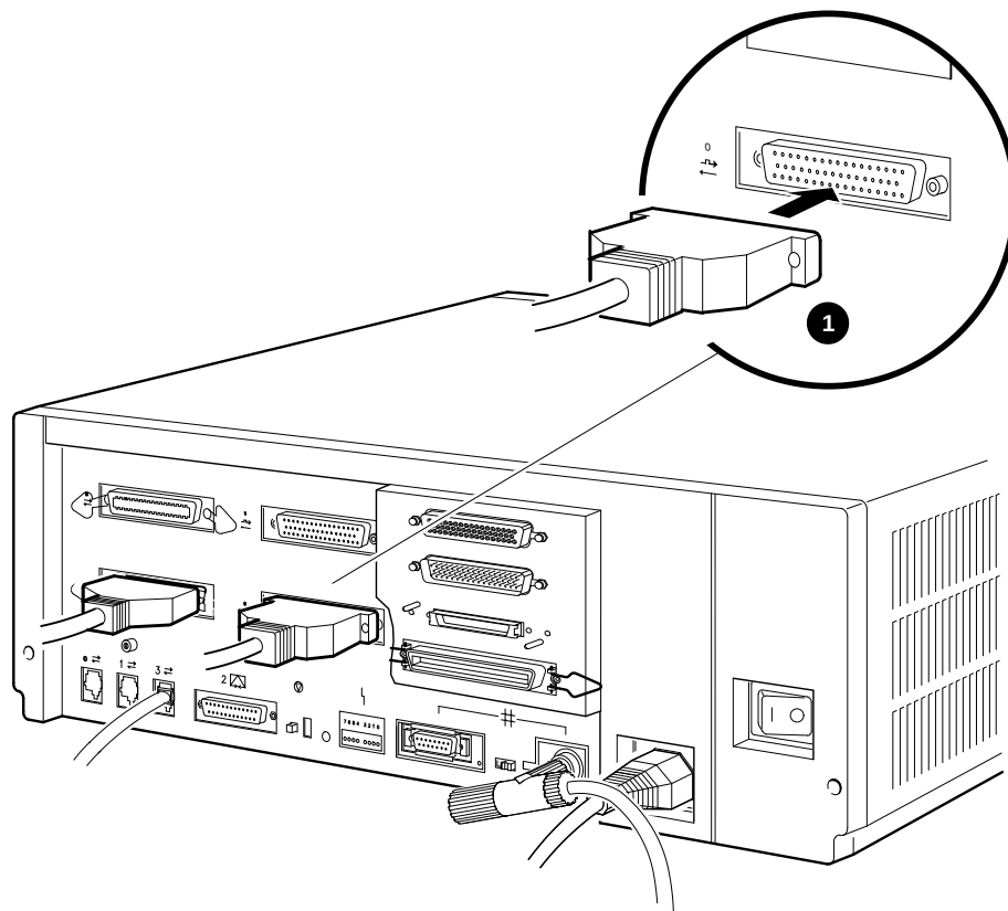
Figure 4-8 Connecting the Cable to Synchronous Port 0
