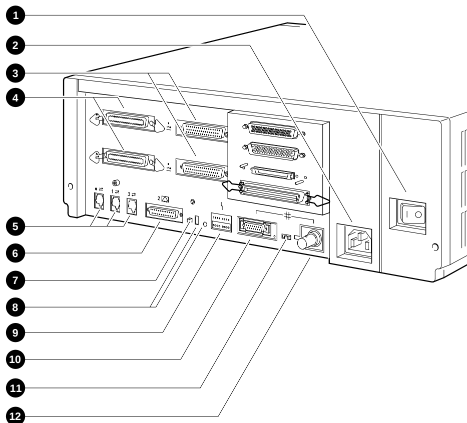
Figure 1-1 VAX 4000 Model 100 Ports, Controls, and LEDs
