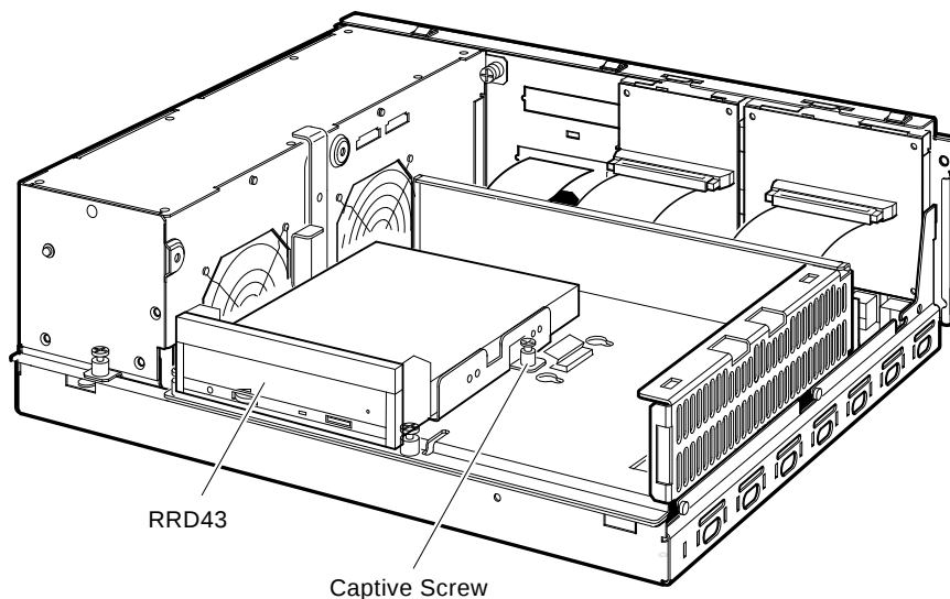
Figure 3-28 Removing the RRD43 CD-ROM Drive
