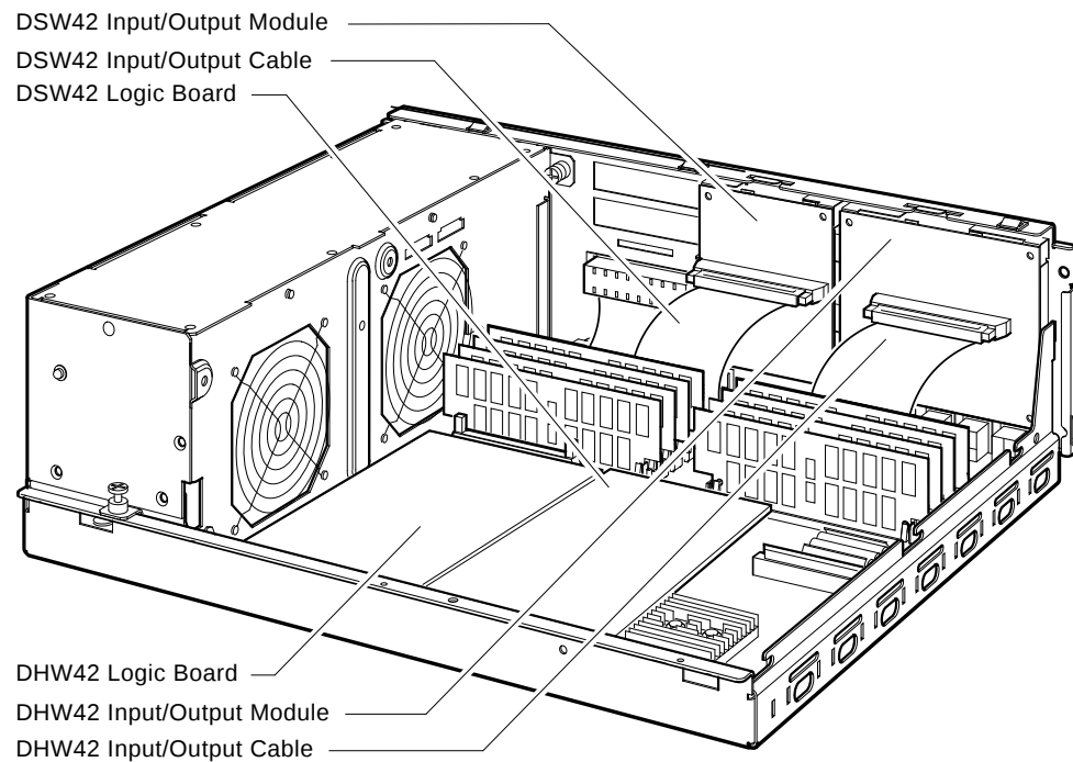
Figure 1–9 Communications Options in Model 100/100A/105A Systems
