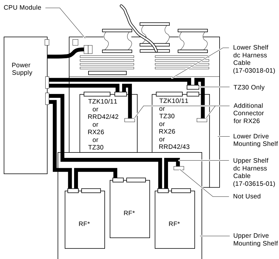
Figure 1–5 Power Distribution
