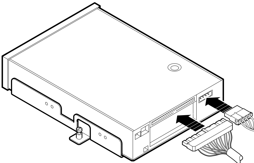
Figure 6-3 Connecting the Power Cable and the SCSI Cable
