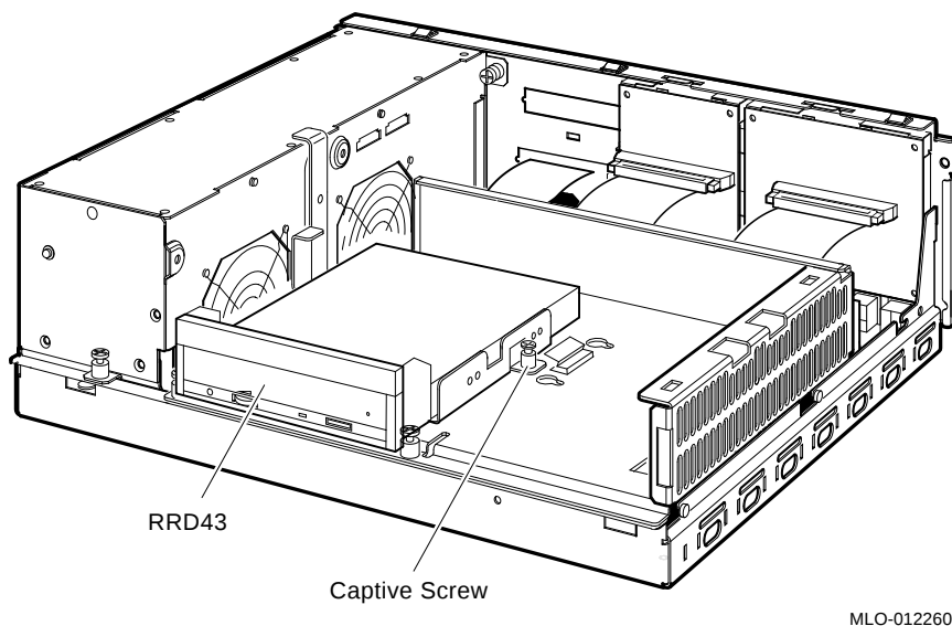
Figure 7-4 Installing the RRD43 Option
