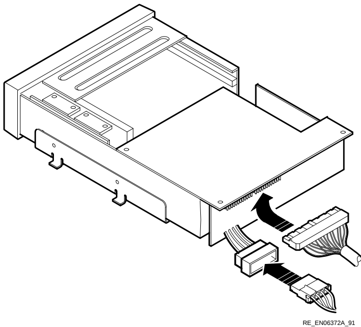
Figure 13–4 Connecting the Power Cable and the SCSI Cable
