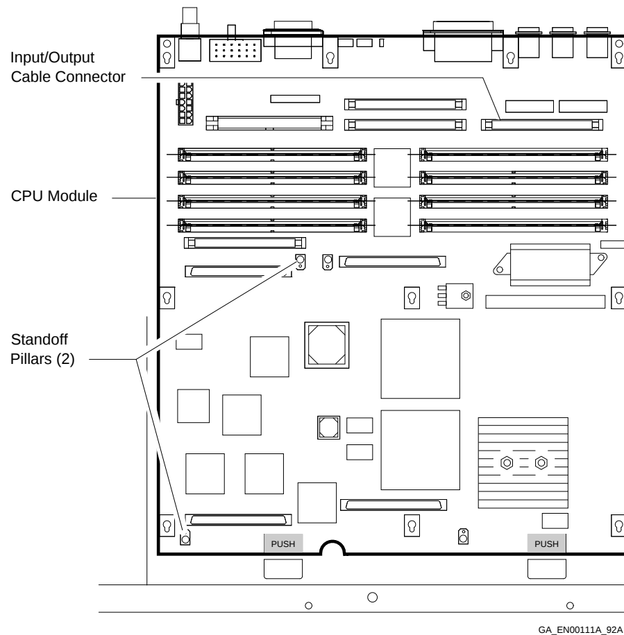
Figure 2–5 Location of the Standoff Pillars on the KA52/KA53 CPU Module
