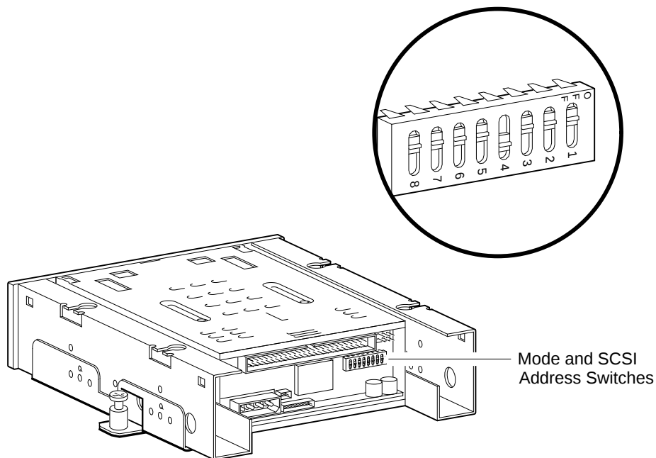
Figure 12-2 TLZ06/TLZ07 SCSI ID Jumper Switch Locations
