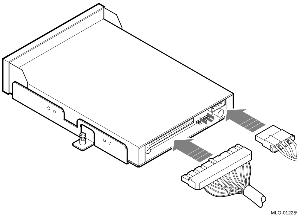
Figure 7-3 Connecting the Power and SCSI Cables
