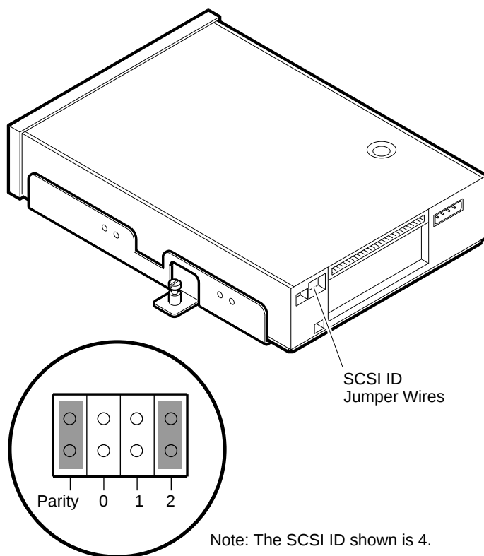
Figure 6-2 RRD42 SCSI ID Jumper Wire Locations
