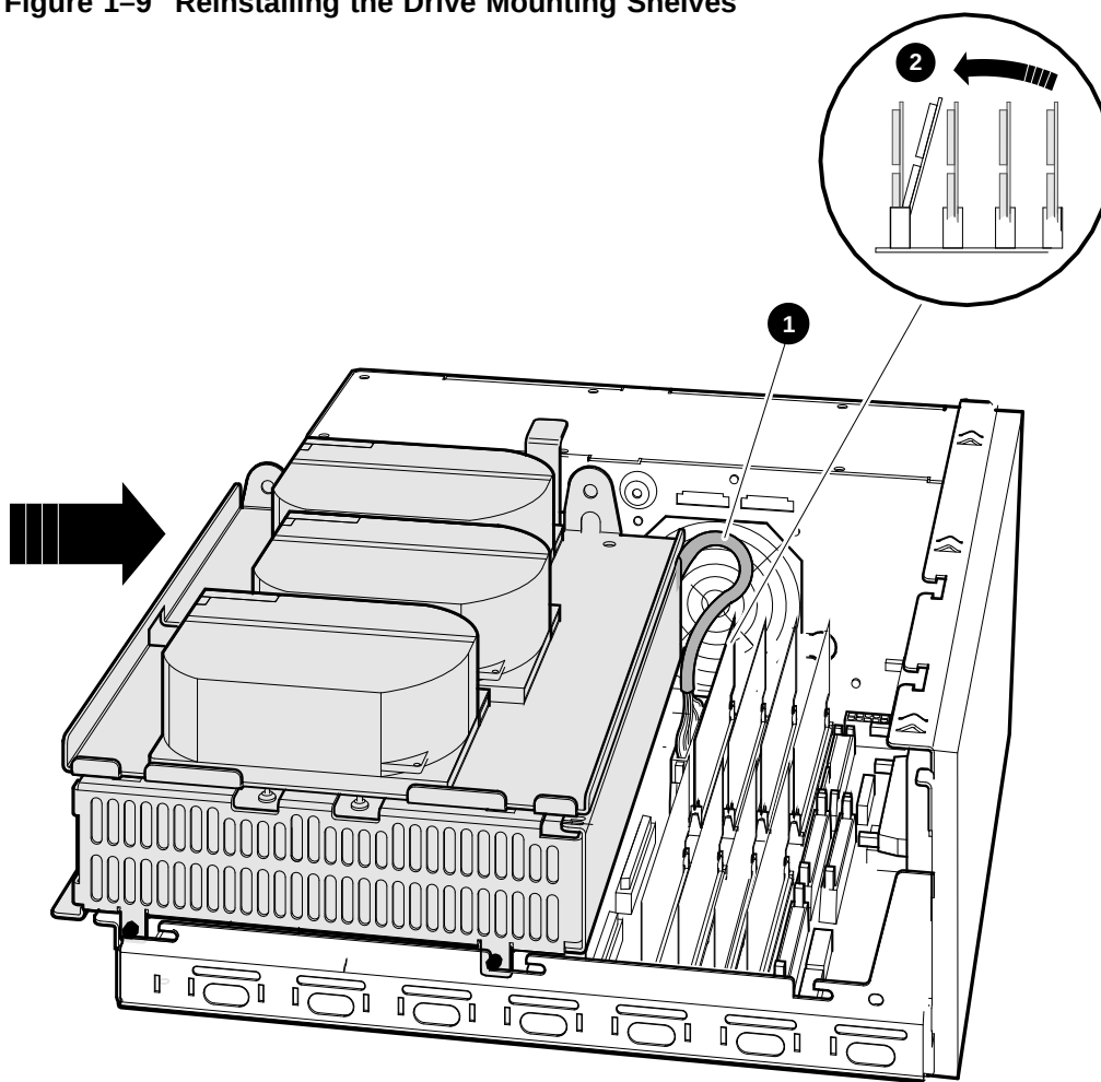
Figure 1-9 Reinstalling the Drive Mounting Shelves
