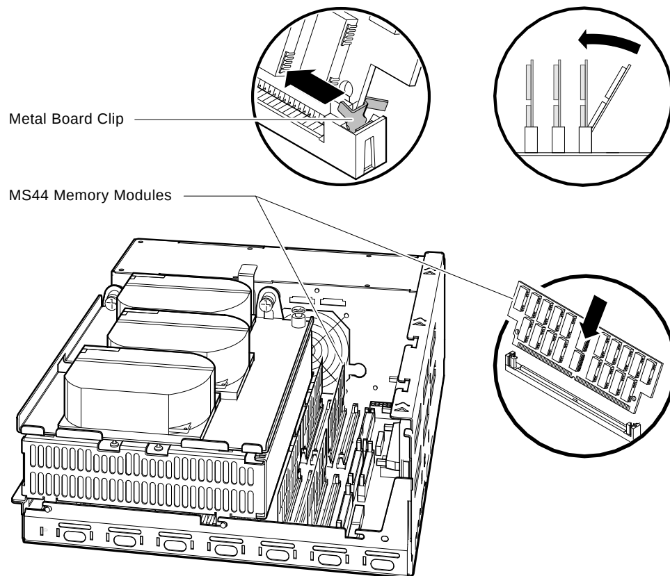
Figure 4-2 Memory Module Installation
