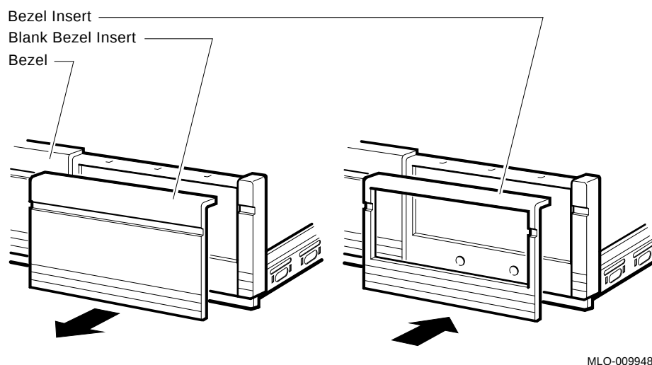
Figure 13–3 Installing the TZ30 Bezel Insert
