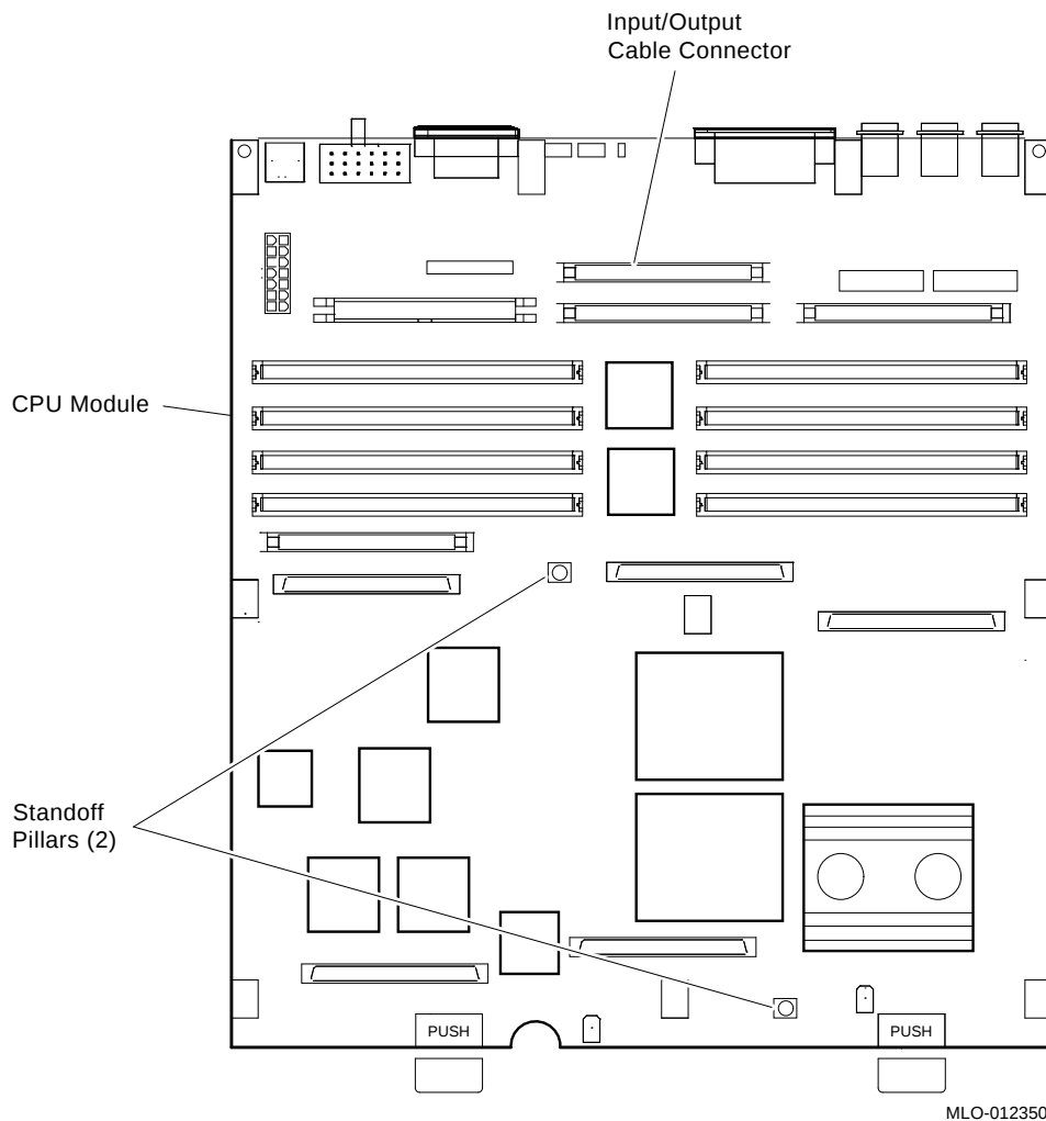
Figure 3-5 Location of the Standoff Pillars on the KA52/53/54 CPU Module
