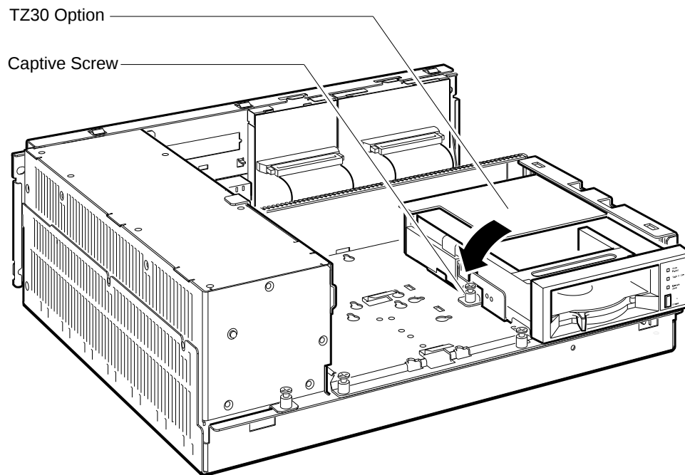
Figure 13–5 Installing the TZ30 Option
