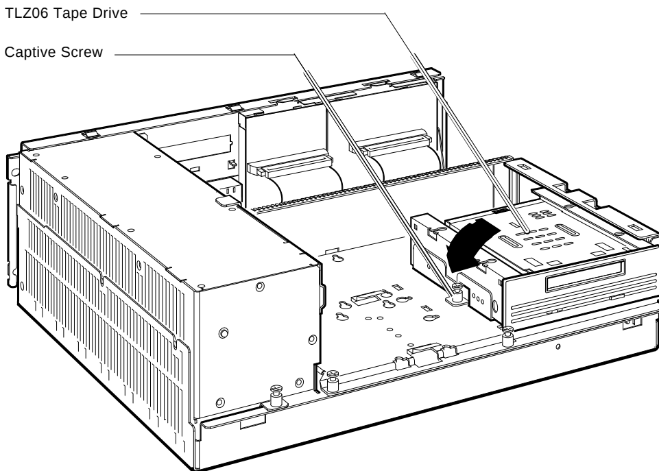
Figure 12–4 Installing the TLZ06/TLZ07 Tape Drive
