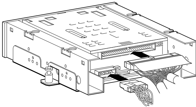
Figure 12–3 Connecting the Power Cable and the SCSI Cable
