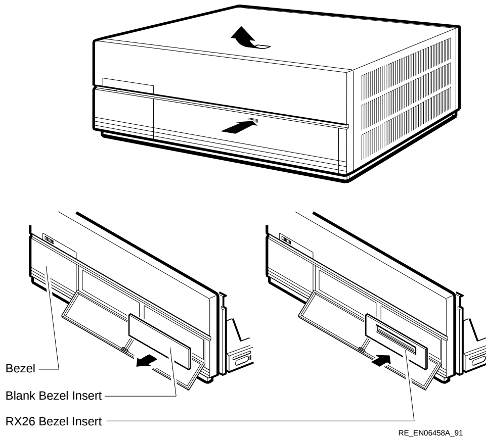
Figure 8-3 Installing the RX26/RX23 Bezel Insert in a BA42B-Based System
