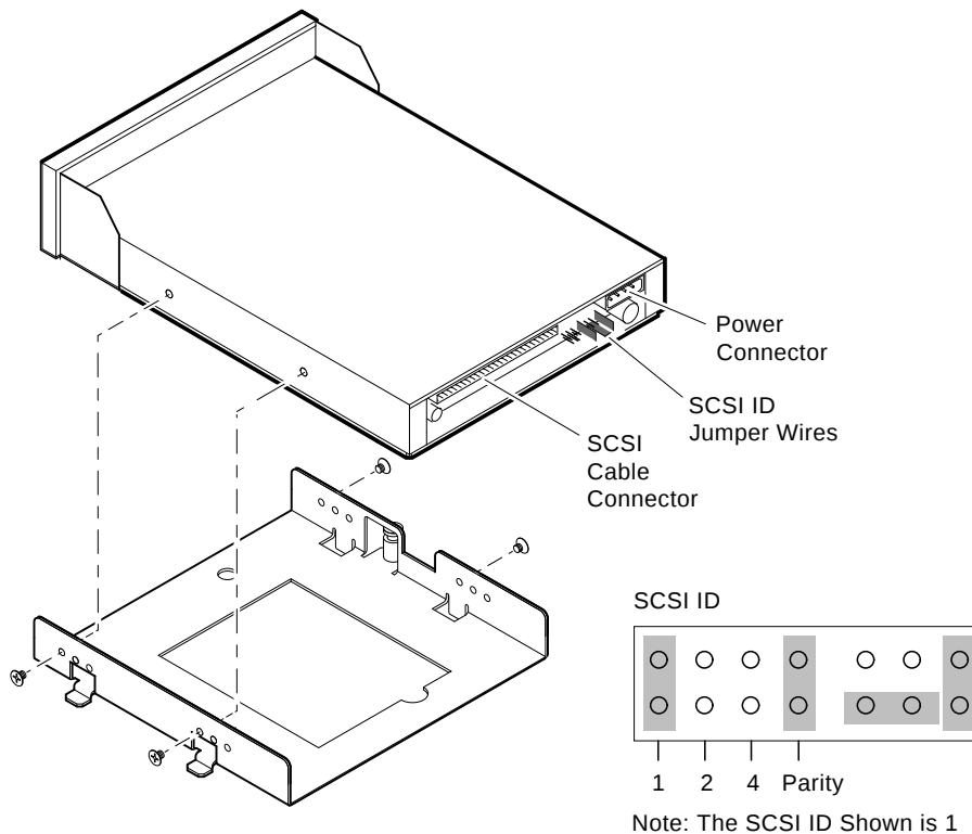
Figure 7-2 RRD43 CD-ROM Drive Jumper Locations
