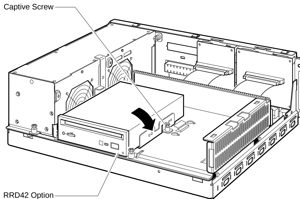
Figure 6-4 Installing the RRD42-EK Option
