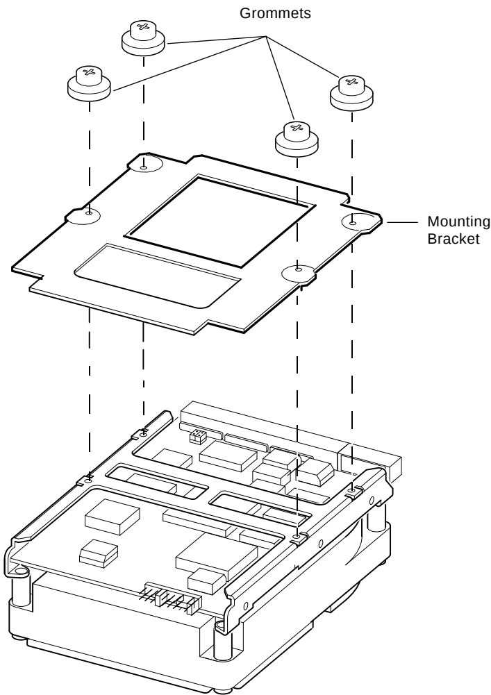
Figure 11–2 RZ26 Disk Drive with Mounting Bracket
