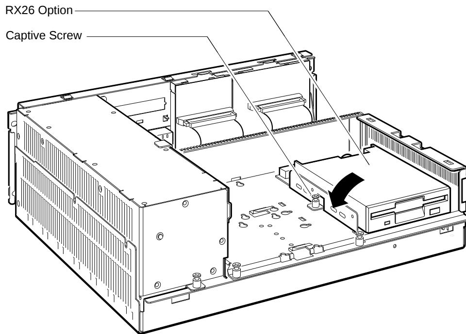
Figure 8-5 Installing the RX26-EL/RX23-EL Option
