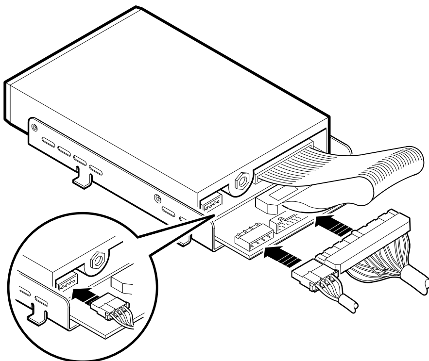
Figure 8–4 Connecting the Power Cables and the SCSI Cable
