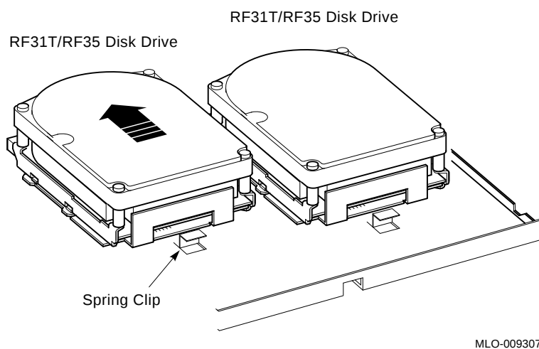
Figure 5–3 Installing a Sample RF31T/RF35/RF36 Disk Drive Option
