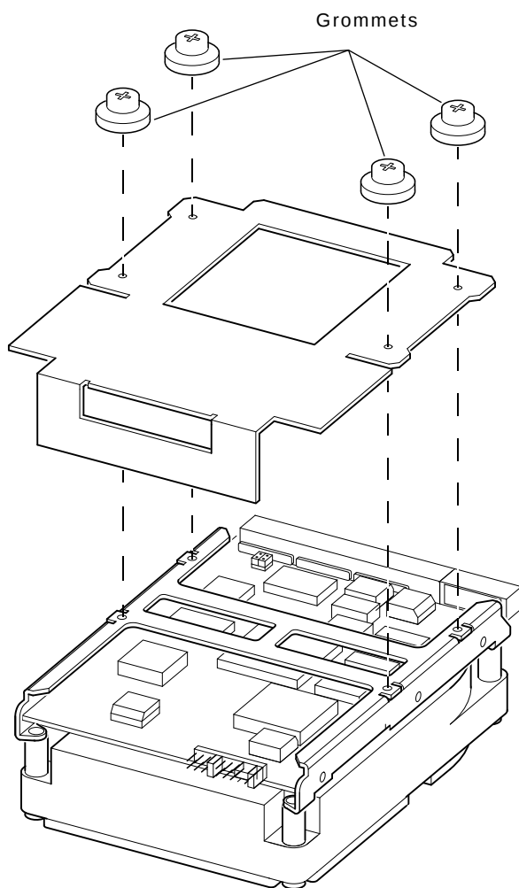
Figure 5-2 Sample RF31T/RF35/RF36 Disk Drive Option with Mounting Brackets
