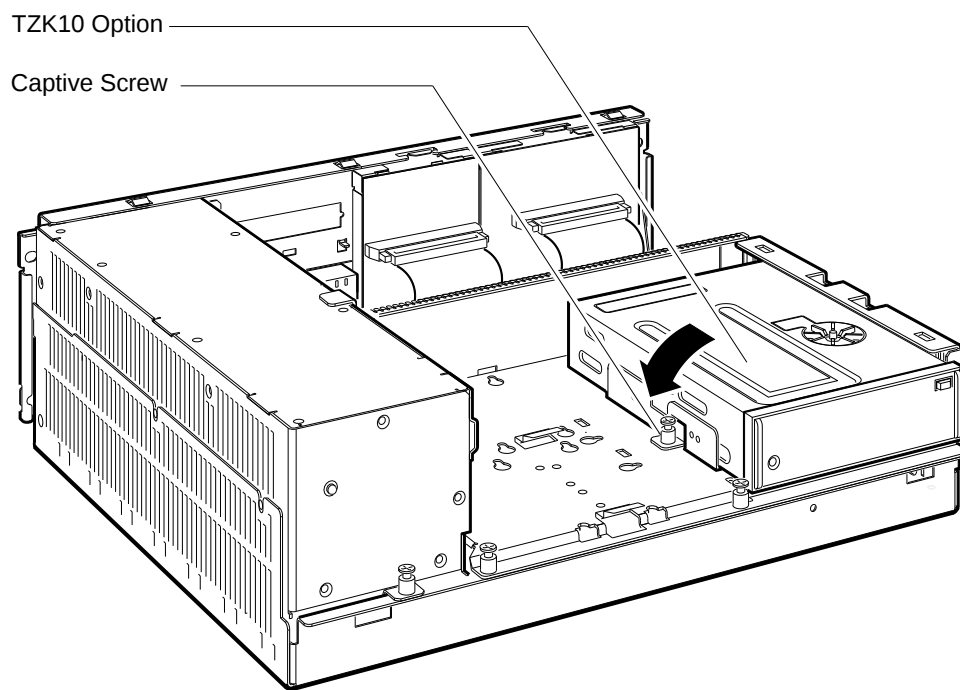
Figure 14–4 Installing the TZK10/TZK11 Option
