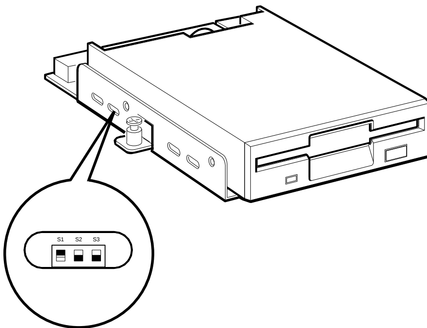
Figure 8-2 Ventilation Slot for SCSI ID Switch Access
