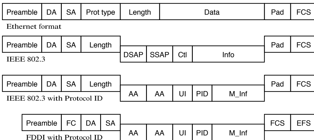
Figure 32: NI Frame Formats
