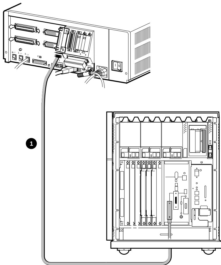
Figure 3-9 Connecting Systems Into a VAXcluster
