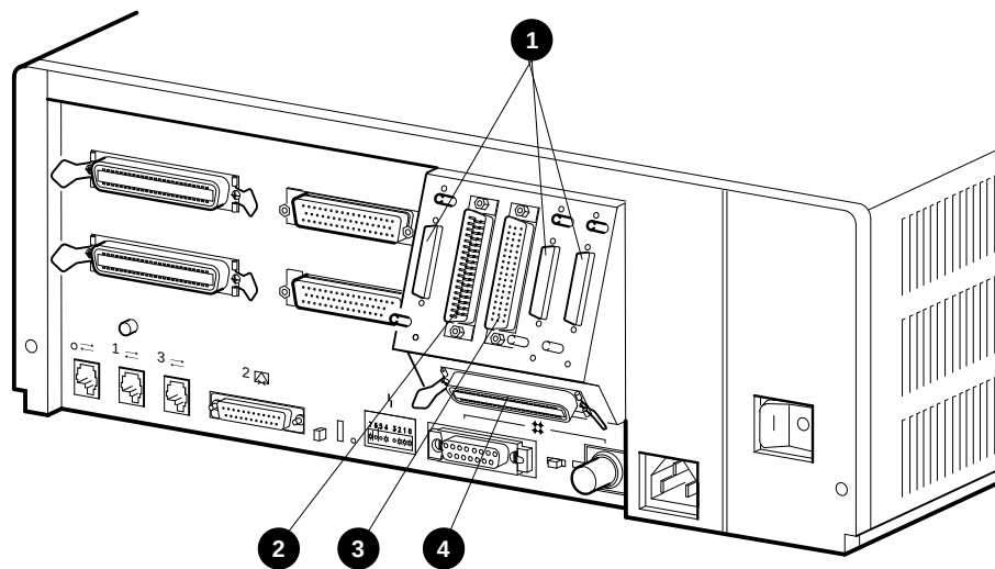
Figure 1-2 VAX 4000 Model 100A Expansion Ports
