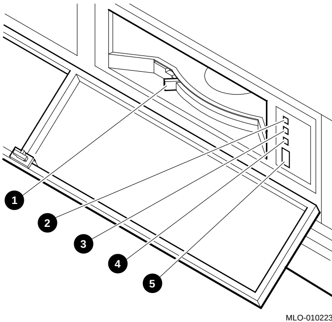
Figure 2-2 TZ30 Tape Drive Controls and LEDs
