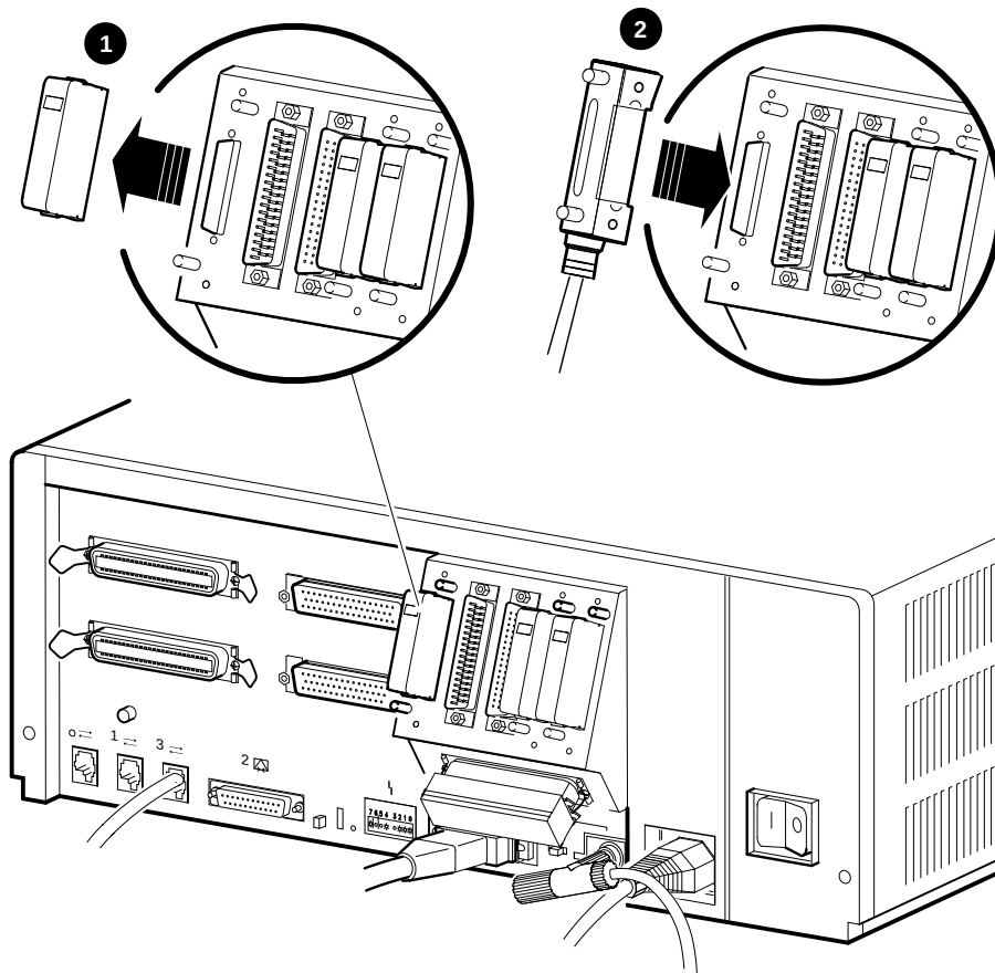
Figure 3–8 Connecting a DSSI Cable to the System Unit
