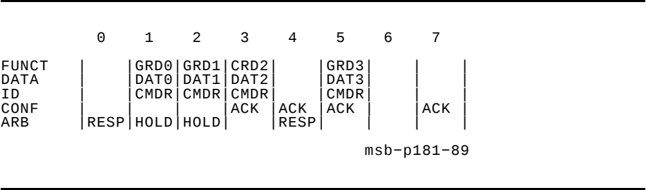
Figure 2–29 Hexword Read with Single Correctable Read Error
