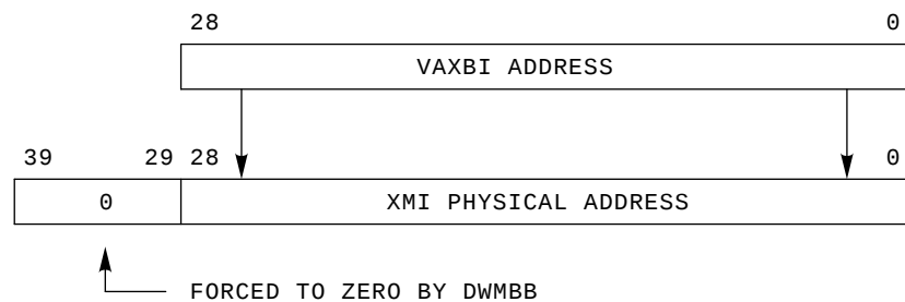
Figure 3-3 DWMBB Compatibility Mode Address
