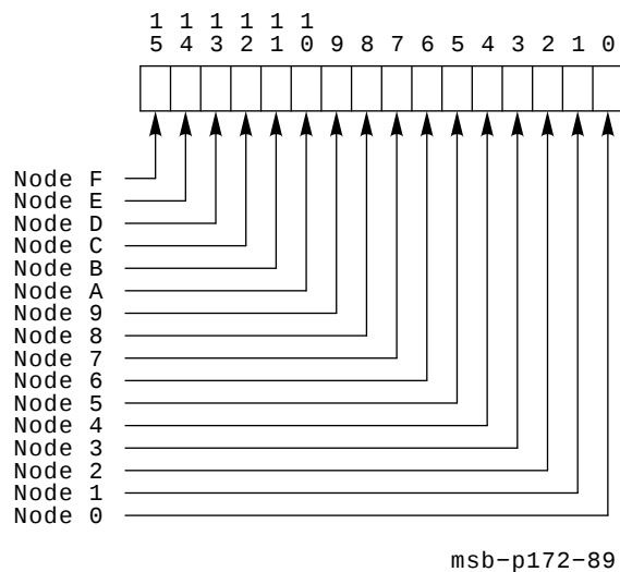
Figure 2–11 Node Specifier Field
