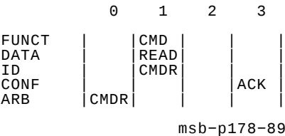
Figure 2–27 Four Longword Reads
