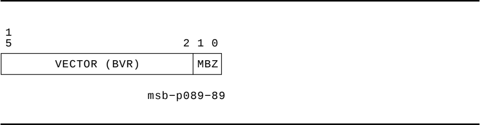
Figure 3–8 XMI Vector Format
