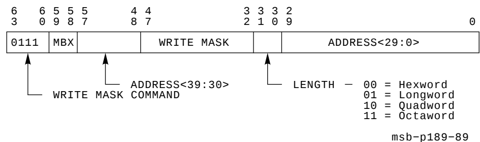
Figure 2–16 Write Mask Command
