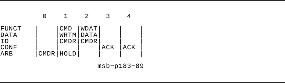
Figure 2–31 Longword and Quadword Writes
