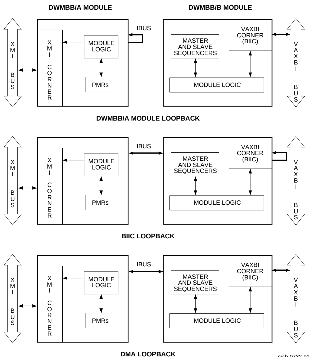
Figure 3–14 DWMBB Loopbacks
