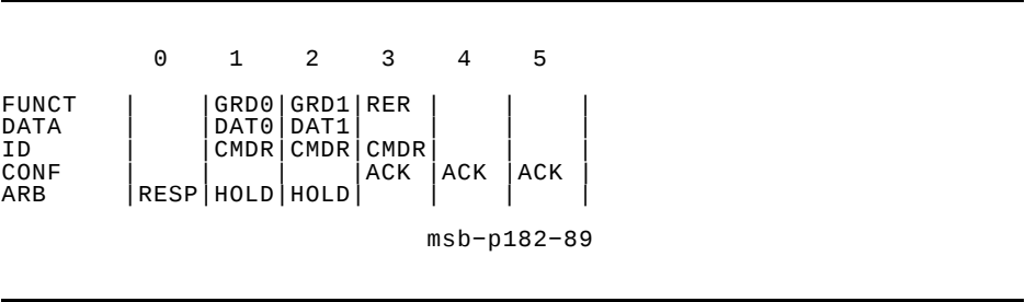
Figure 2–30 Hexword Data Return with Uncorrectable Read Error
