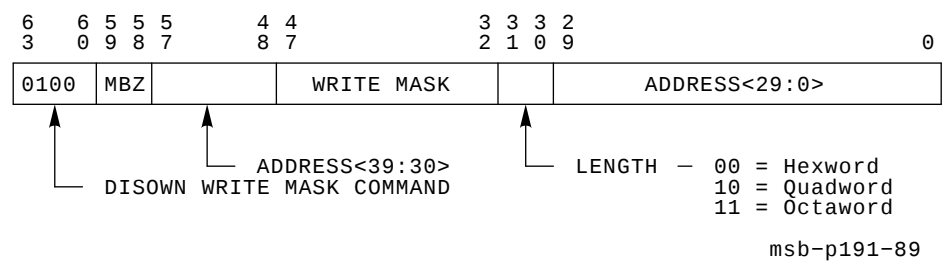
Figure 2-18 Disown Write Mask Command
