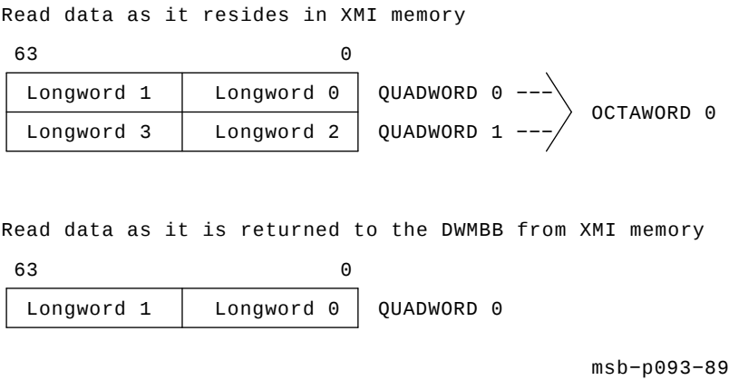
Figure 3–11 VAXBI Wrapped Read Transactions
