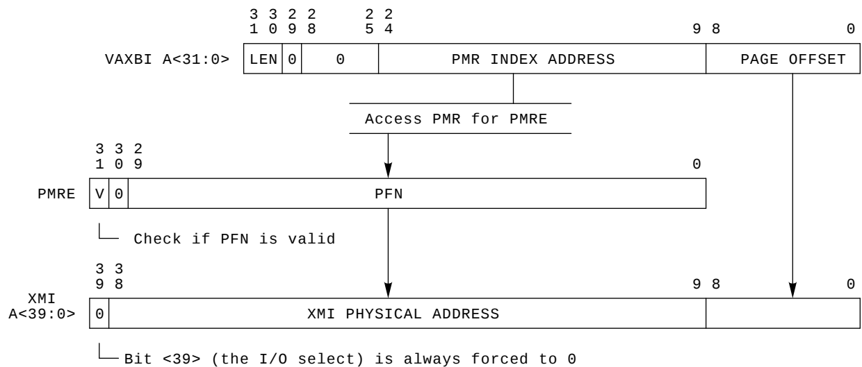
Figure 3–4 40-Bit Addressing Mode with 512-Byte Page Size
