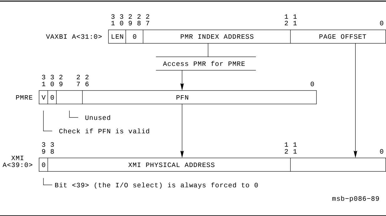
Figure 3–5 40-Bit Addressing Mode with 4-Kbyte Page Size
