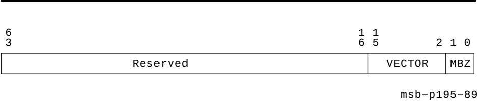
Figure 2–22 Identify Response
