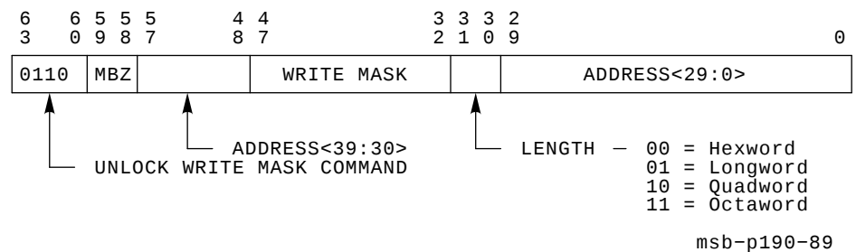
Figure 2–17 Unlock Write Mask Command
