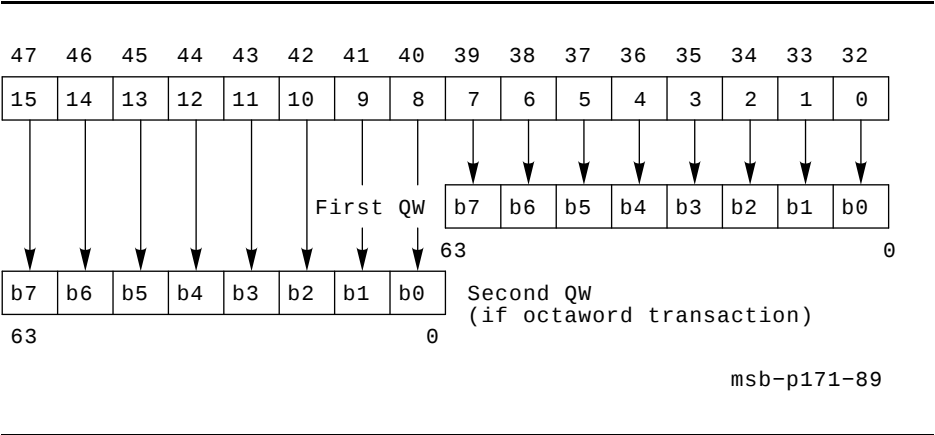
Figure 2–9 Mask Field Bit Assignments
