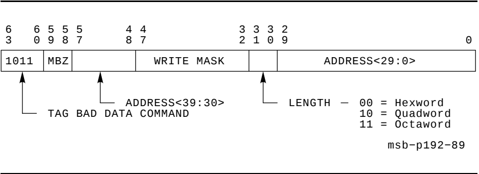
Figure 2–19 Tag Bad Data Command
