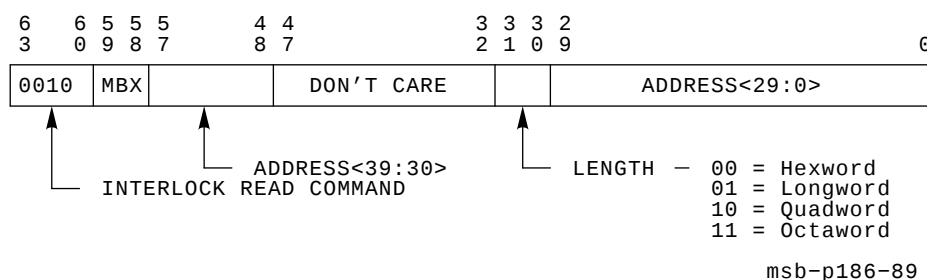
Figure 2–13 Interlock Read Command
