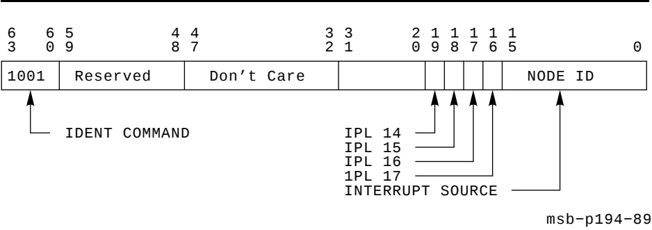
Figure 2–21 Identify Command
