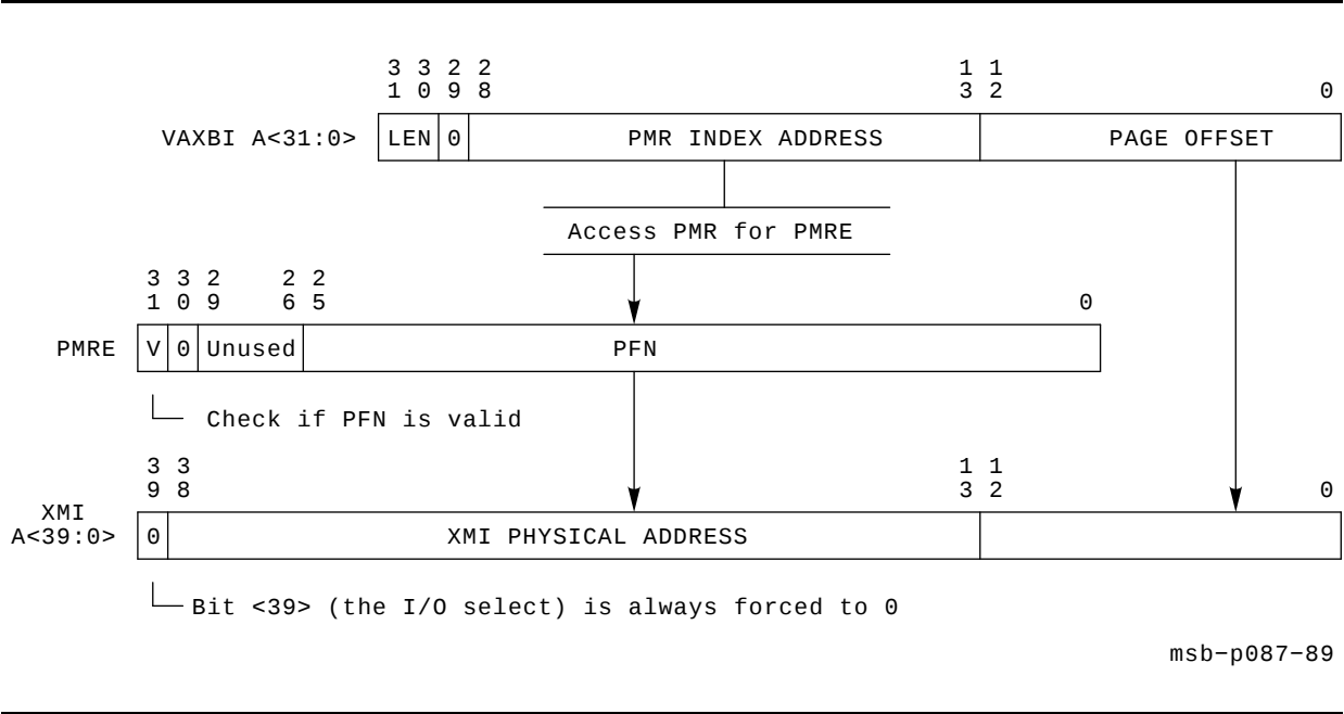
Figure 3-6 40-Bit Addressing Mode with 8-Kbyte Page Size
