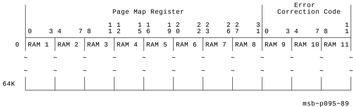
Figure 3–13 Page Map Register Organization
