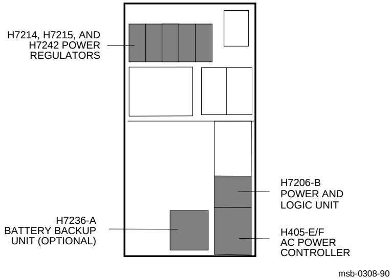
Figure 1-9 Power System (Rear View)
