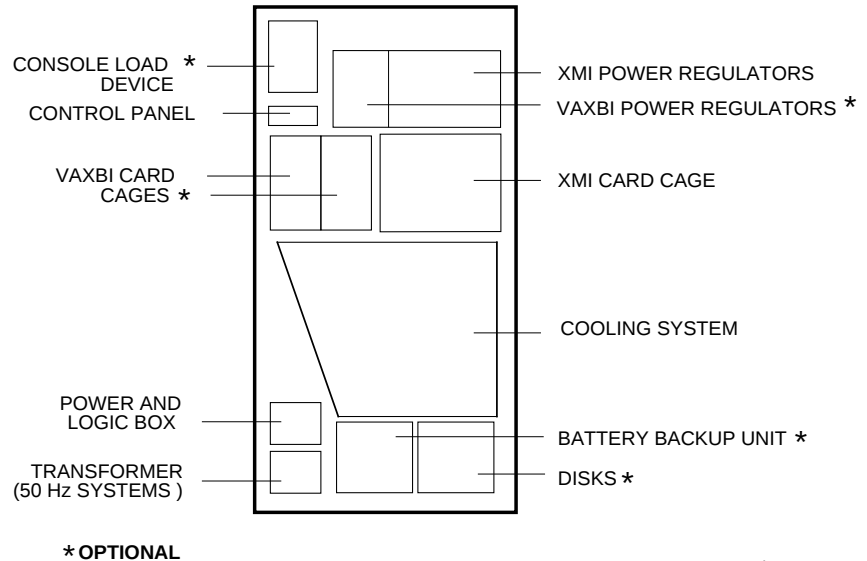
Figure 1-1 System Front View
