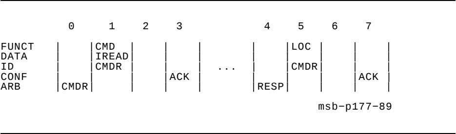
Figure 2–25 Interlock Read Transaction to a Locked Location
