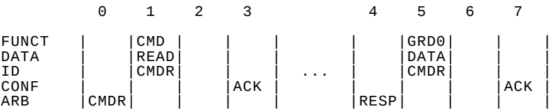
Figure 2–24 Read Transaction
