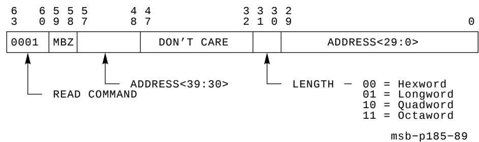
Figure 2–12 Read Command
