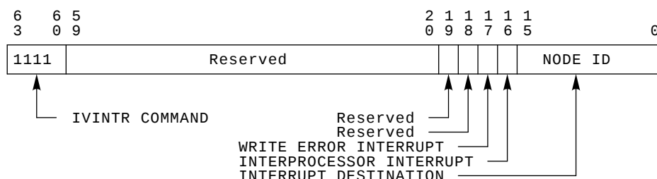
Figure 2–23 Implied Vector Interrupt Command
