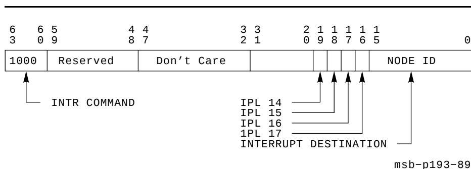
Figure 2-20 Interrupt Command
