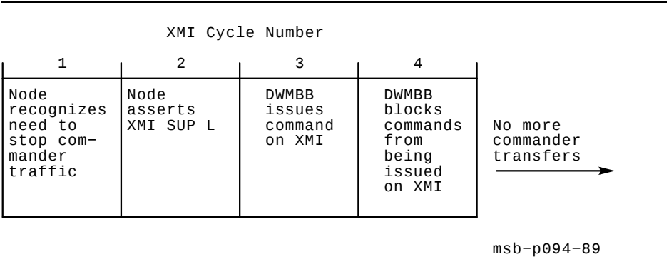
Figure 3–12 Responder Request and XMI SUP L Timing
