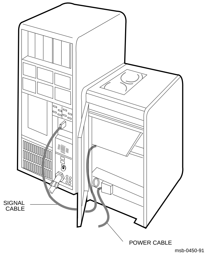
Figure 5-2: Tape Subsystem—Interface Cabling
