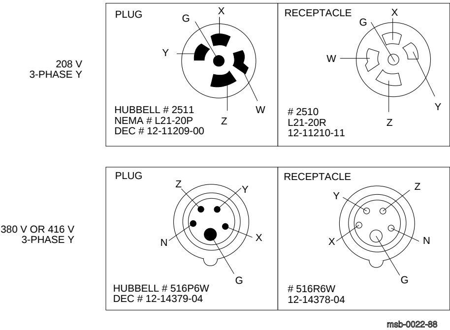
Figure 1–6: AC Power Connectors
