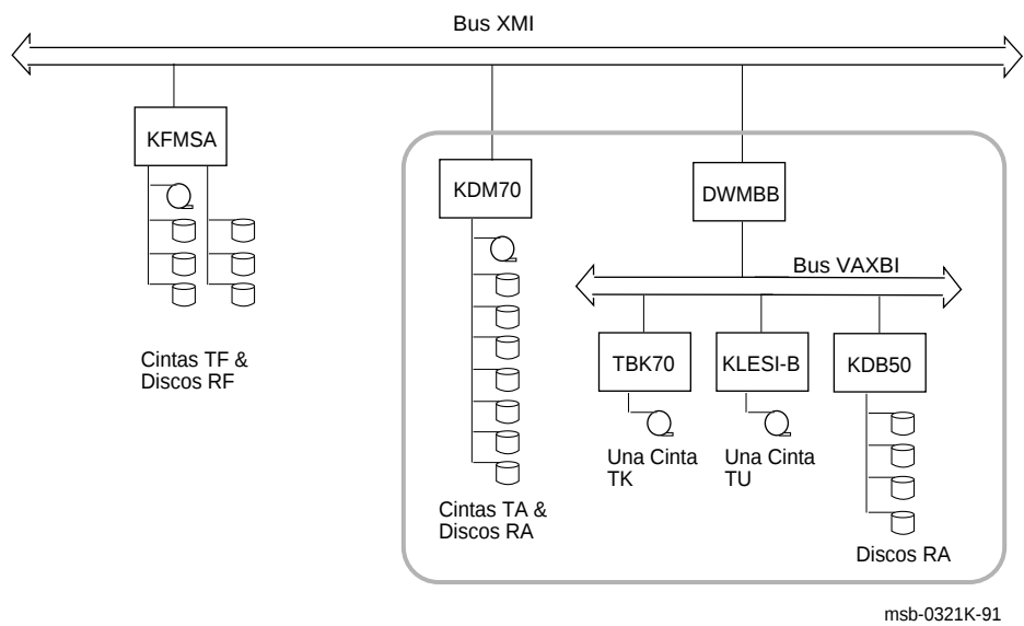
Figure 5-1: Architecture
