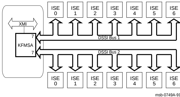
Figure 3–9: Sample Single-Host Configuration
