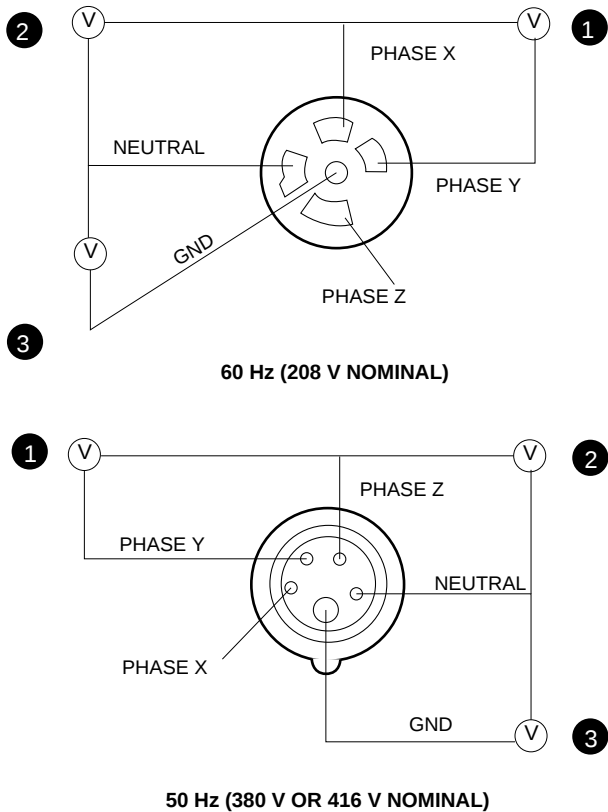
Figure 6-3: Measuring System Power
