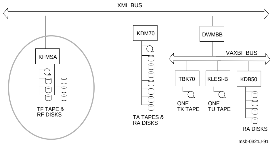
Figure 3-1: System Architecture with KFMSA
