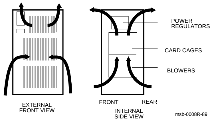
Figure 1-2: Airflow Pattern
