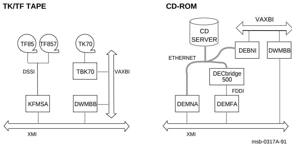
Figure 8-1: Console Load Devices
