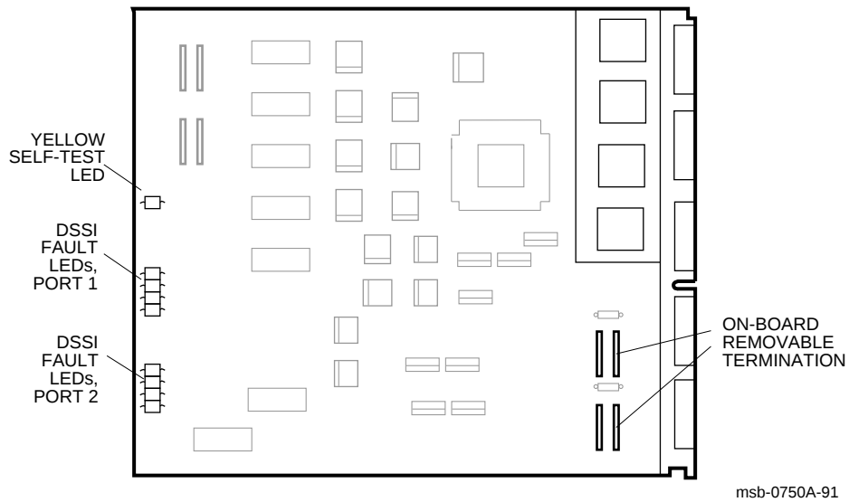
Figure 3-4: KFMSA LEDs
