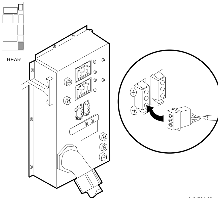
Figure C-5: DEC Power Bus Cable Connections (Rear View)
