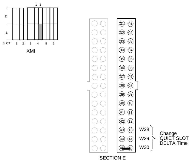
Figure 4-2: CIXCD Jumper to Set Quiet Slot DELTA Time to 10
