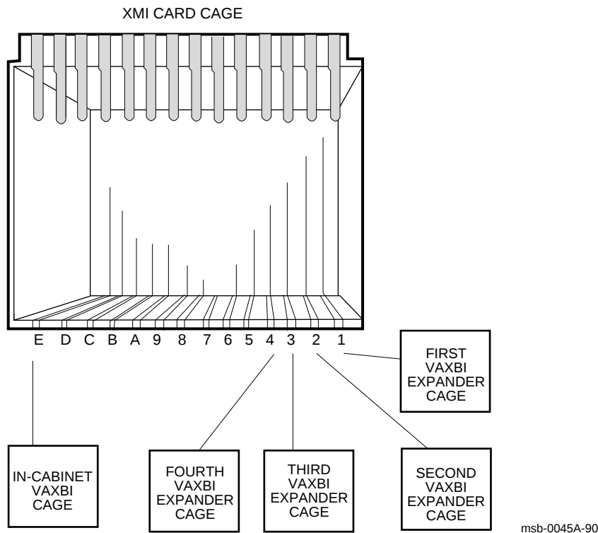
Figure C-7: DWMBB/A Slots for Additional Card Cages
