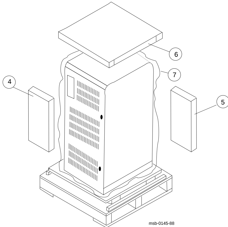
Figure 2-2: Packing Material
