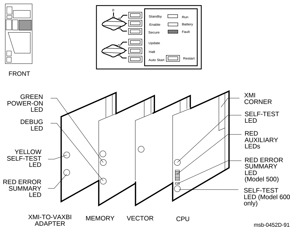
Figure 7-1: Control Panel Lights and Location of Module LEDs
