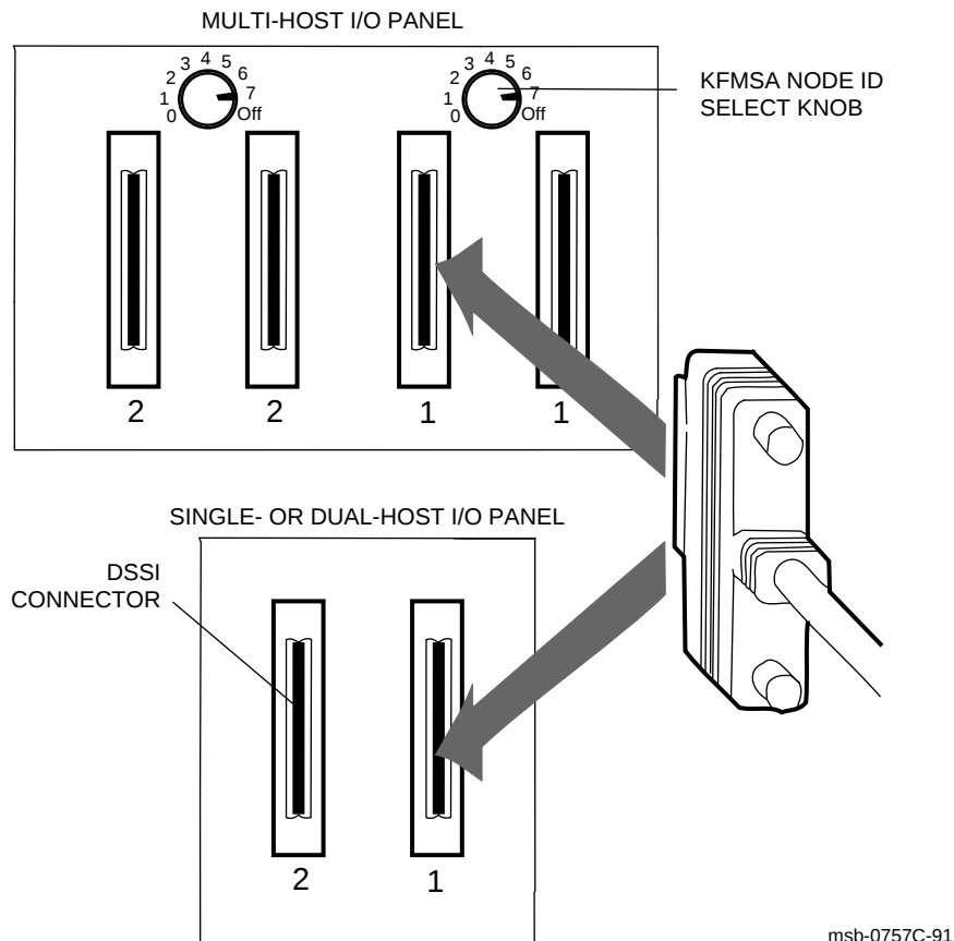
Figure 3-11: I/O Ports for DSSI Cables
