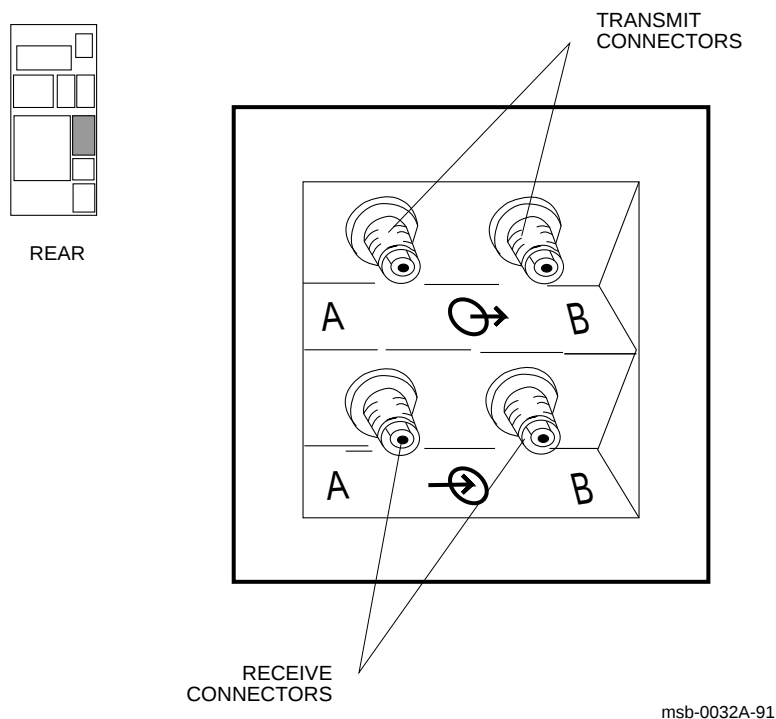
Figure 4-12: I/O Panel—VAXcluster Port
