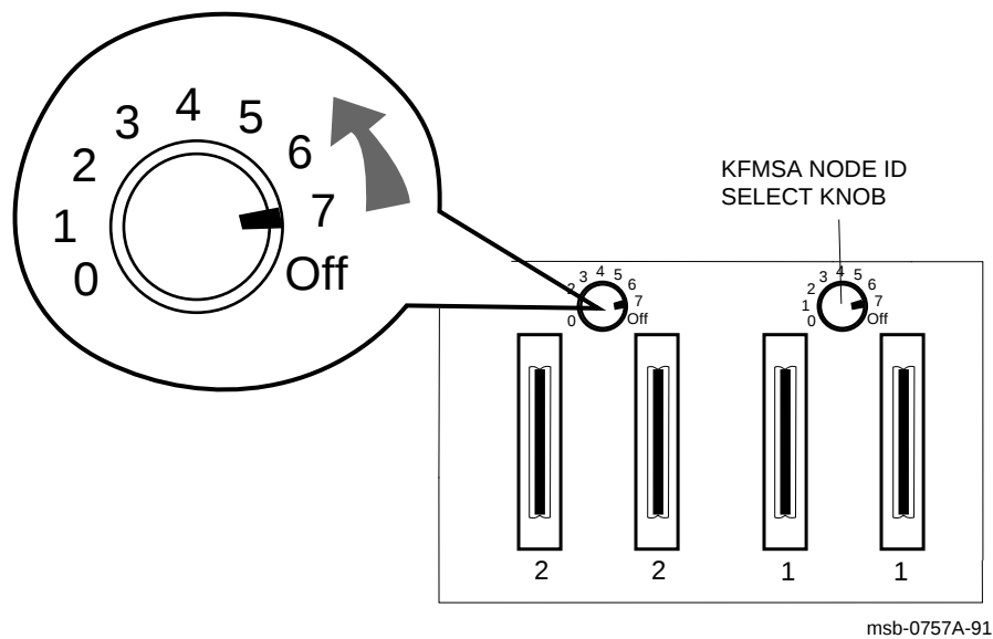
Figure 3–14: Setting the KFMSA Node ID on the I/O Panel
