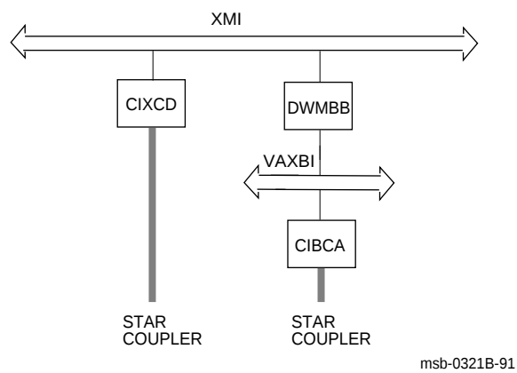
Figure 4-1: Adapters
