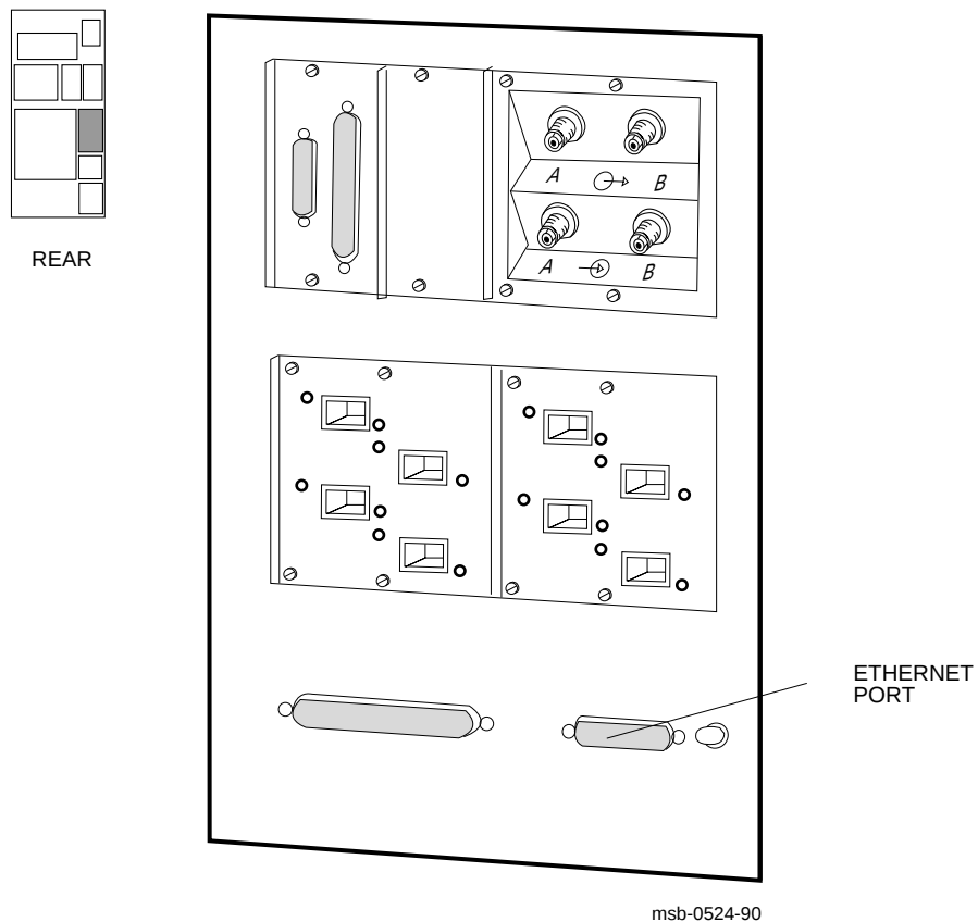
Figure 2-7: I/O Panel—Ethernet Port
