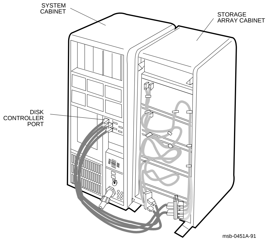
Figure 5-3: Disk Subsystem—Interface Cabling
