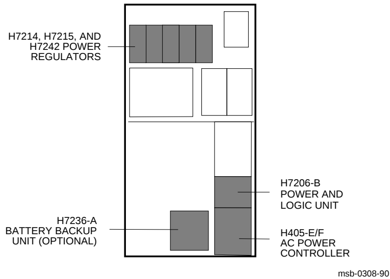
Figure 1-5: Location of Power Modules (Rear View)
