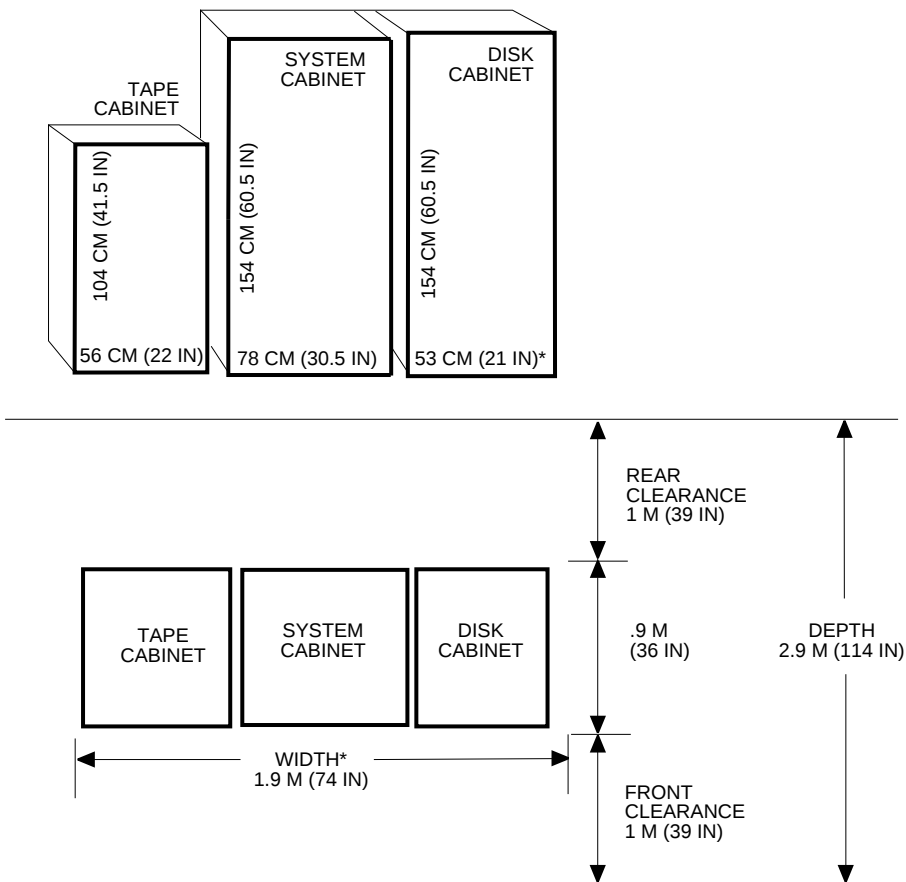
Figure 1-1: Sample Configuration
