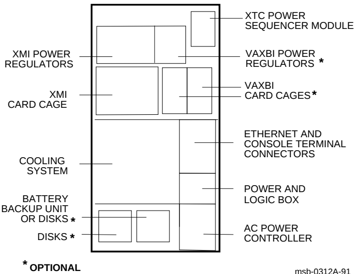
Figure 1-5: System Rear View
