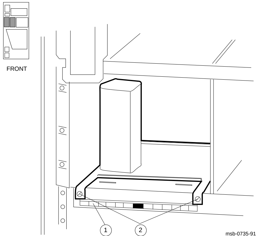
Figure 2-1: Baffle Assembly
