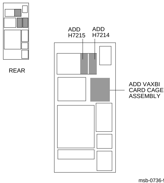
Figure 1-2: Overview of VAXBI Installation
