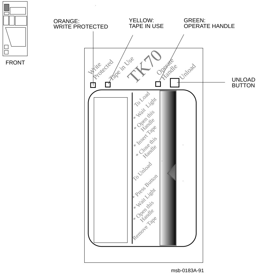
Figure A-1: TK Tape Drive
