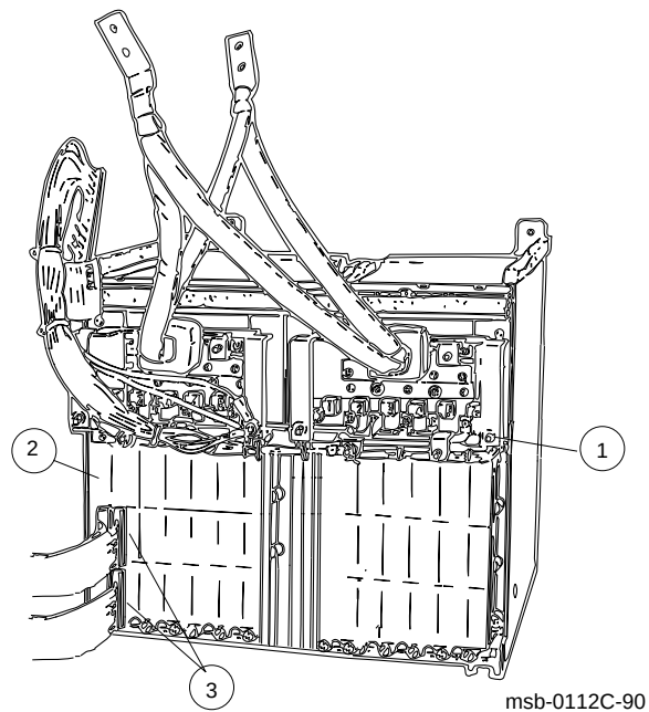
Figure 2-5: VAXBI Backplane Cables and Power Connections
