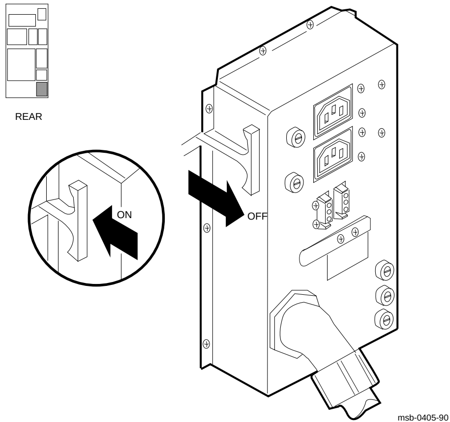
Figure 3-1: AC Power Controller Circuit Breaker
