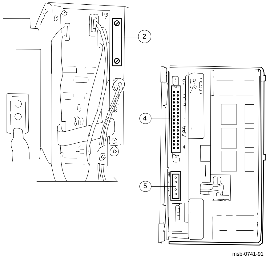
Figure 4-4: Plate Removal and TK70 Tape Drive Connectors
