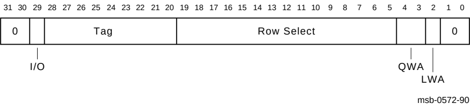
Figure 2-7 Physical Address Division
