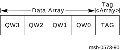
Figure 2-6 Cache Arrangement
