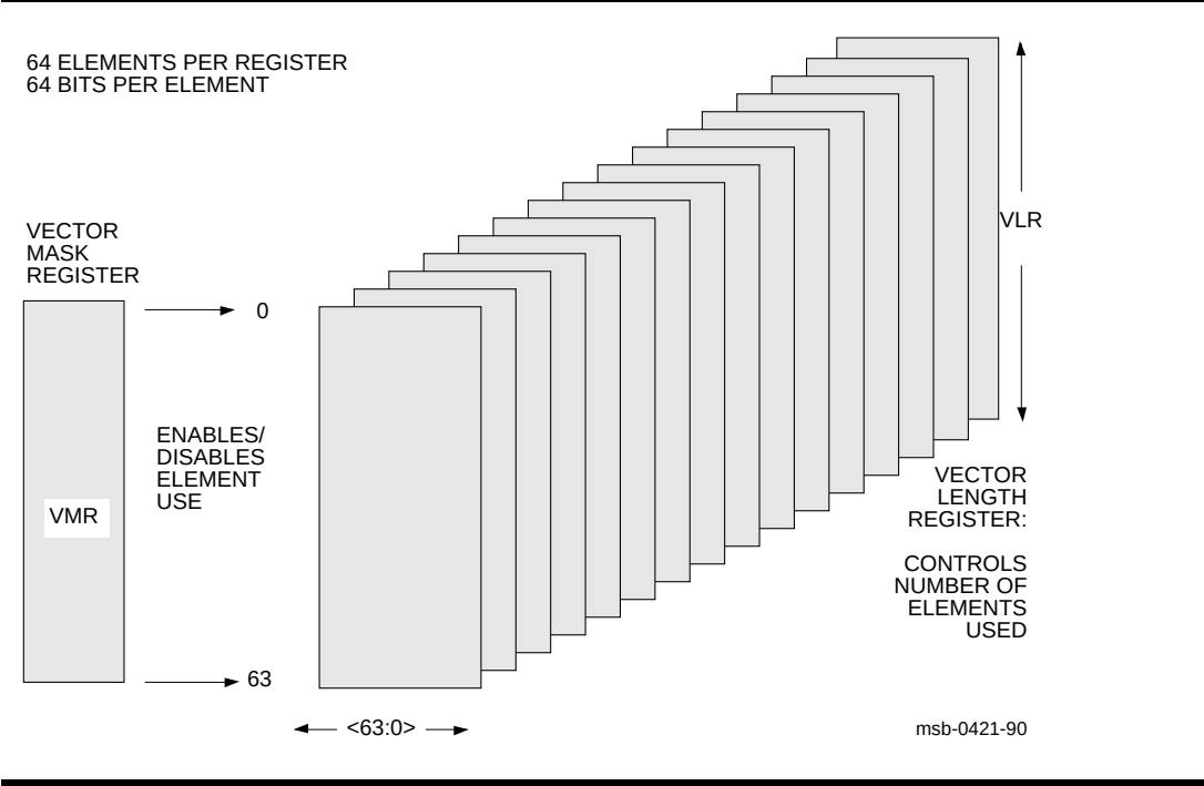
Figure 1-2 Vector Registers
