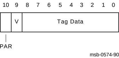
Figure 2-8 Main Tag Memory Organization
