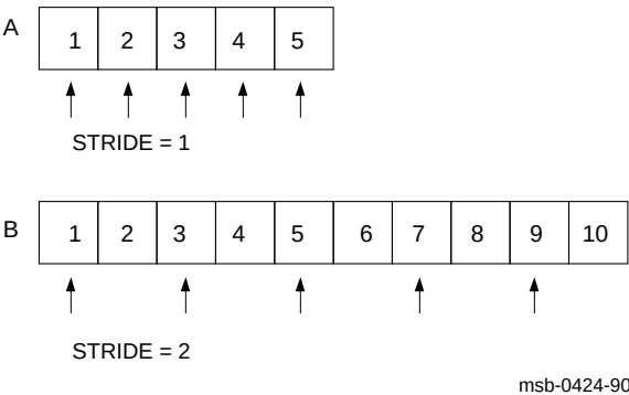
Figure 1-5 Constant-Strided Vectors in Memory
