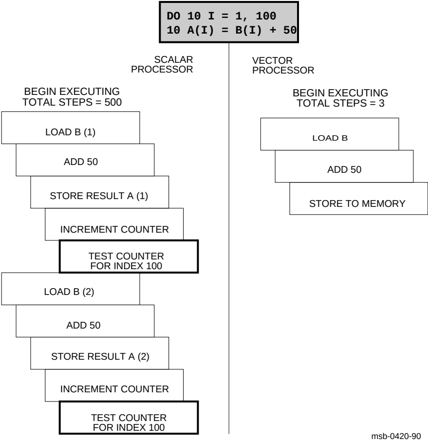
Figure 1-1 Scalar vs. Vector Processing
