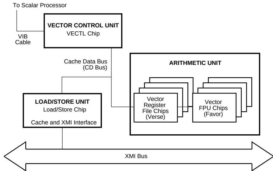
Figure 2-2 FV64A Vector Processor Block Diagram
