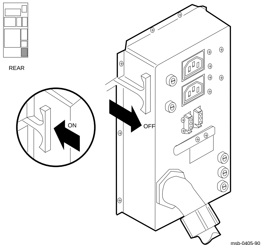
Figure 3-5: AC Power Controller Circuit Breaker
