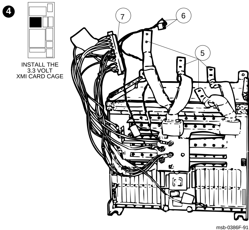
Figure 2-12: XMI-2 Card Cage
