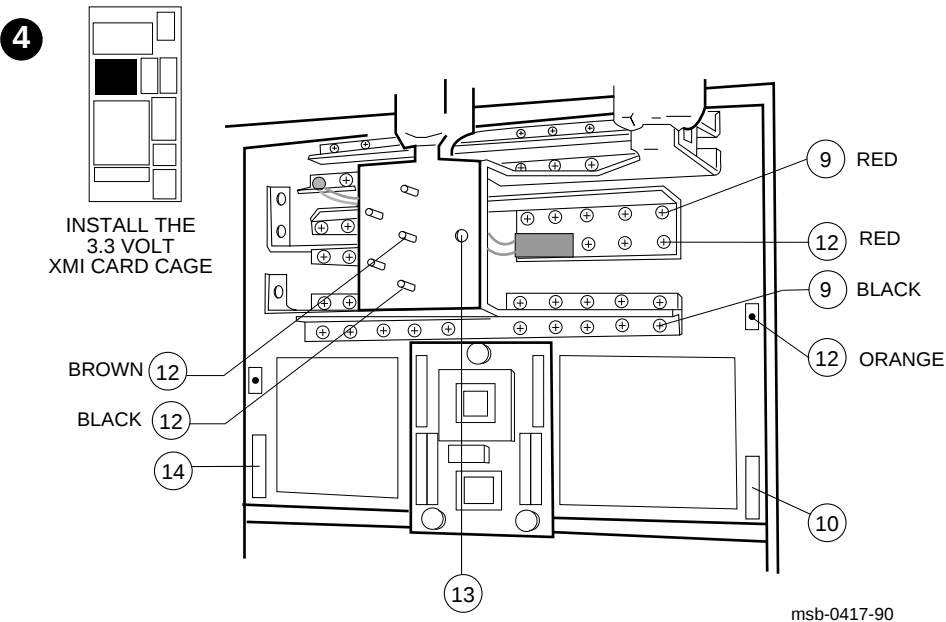
Figure 2-15: Complete XMI-2 Cabling
