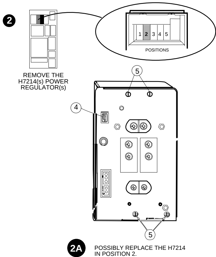
Figure 2-7: Replace the H7214 in Position 2
