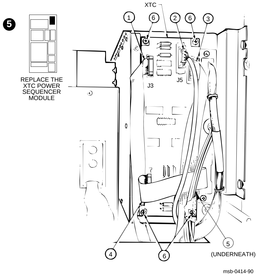
Figure 2-16: Replace the XTC Power Sequencer Module
