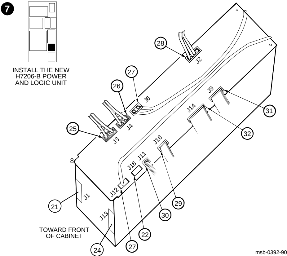
Figure 2-20: H7206-B Power and Logic Unit (Top View)
