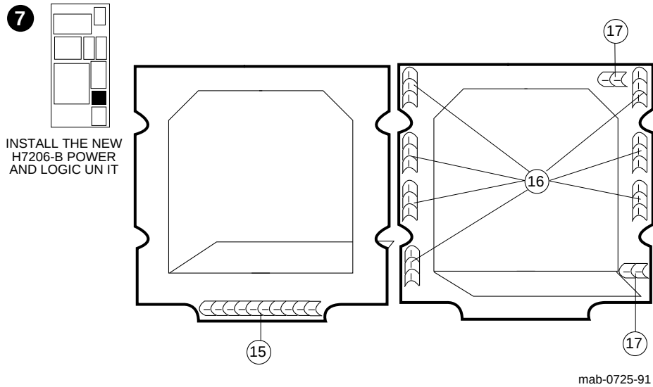
Figure 2-19: Attaching BeCu Clips to New Mounting Plate
