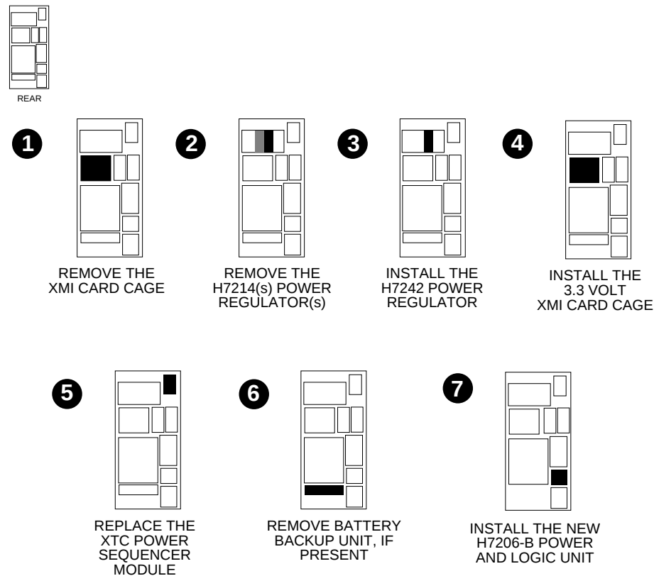
Figure 2-1: Upgrade Overview
