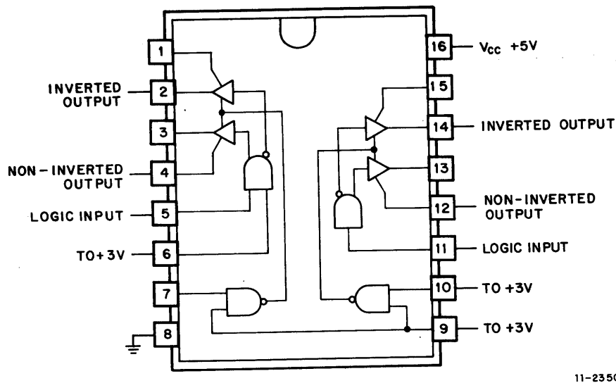
Figure 4-13 Dual Differential Driver Pin Connection Diagram
