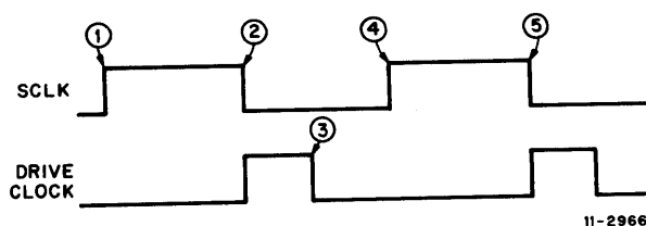
Figure 4-8 Massbus Data Transfer Sequence
