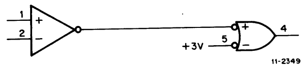
Figure 4-14 Simplified Line Receiver Logic Diagram
