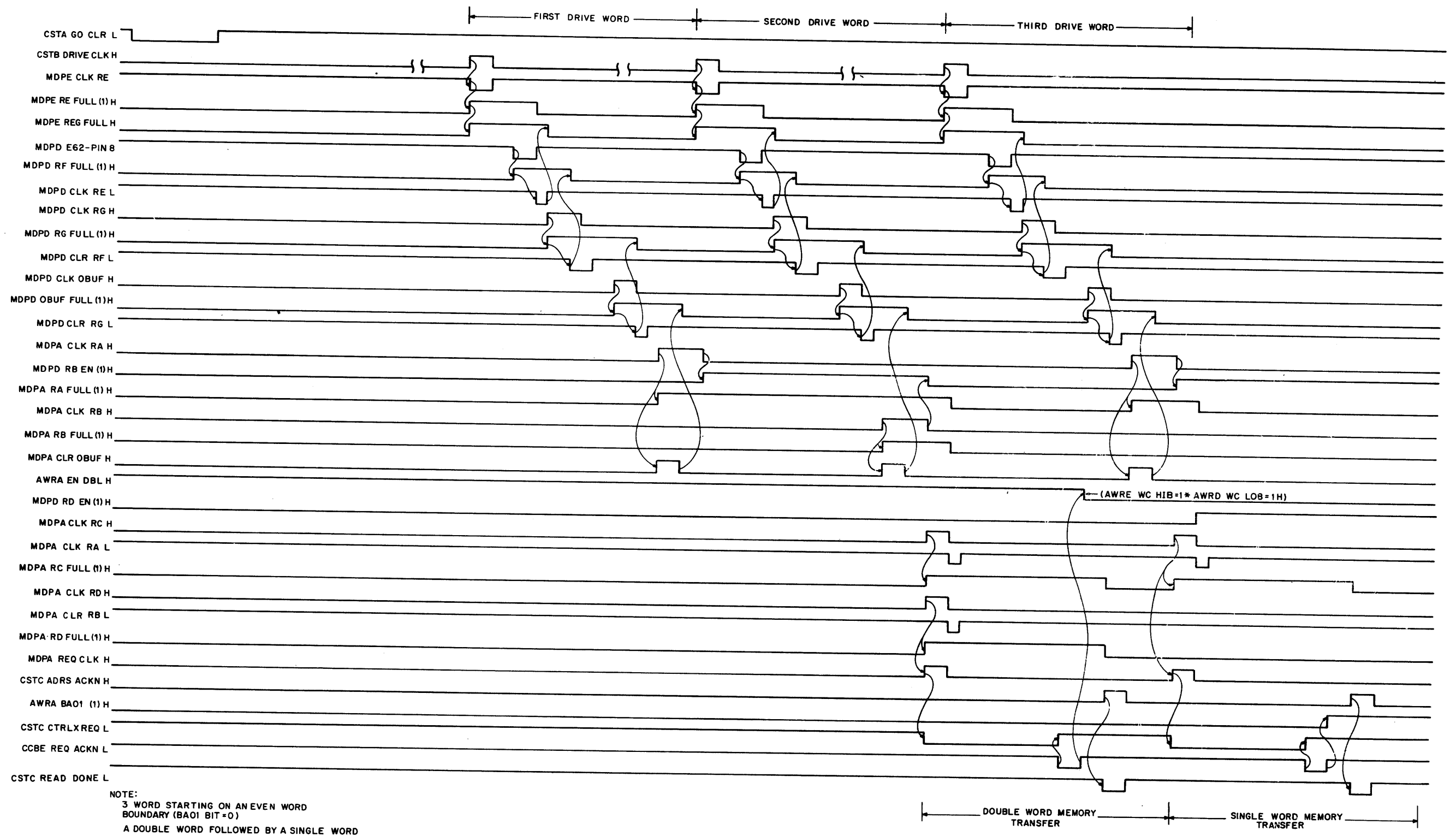
Figure 4-5 Data Buffer Read Command Timing Diagram
