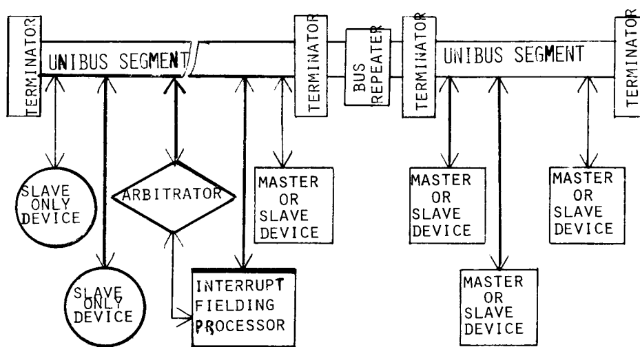
(B) TWO-SEGMENT UNIBUS WITH SLAVE DEVICES ON BOTH SIDES OF ARBITRATOR
