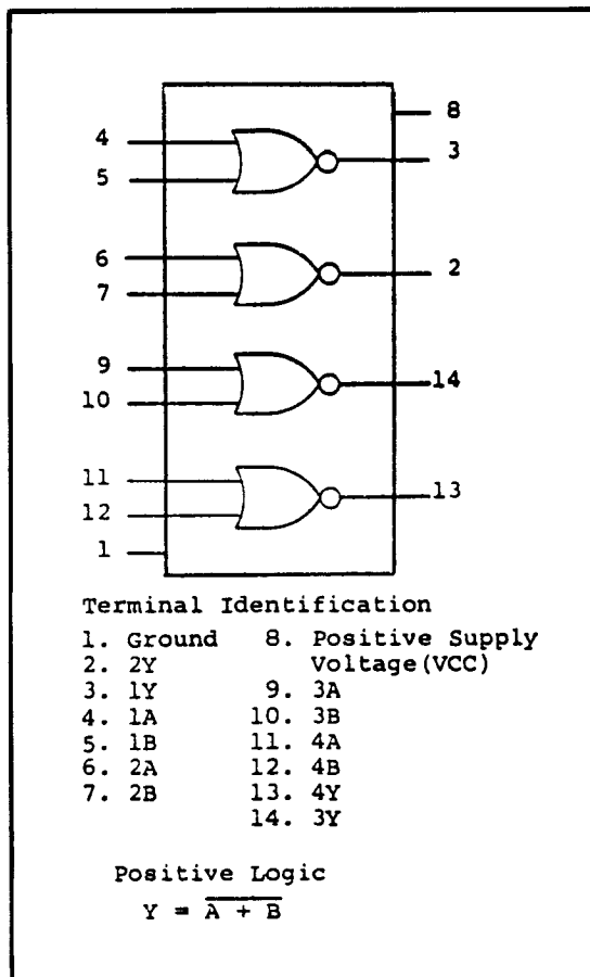
Figure 4-1. 8640 Bus Receiver
