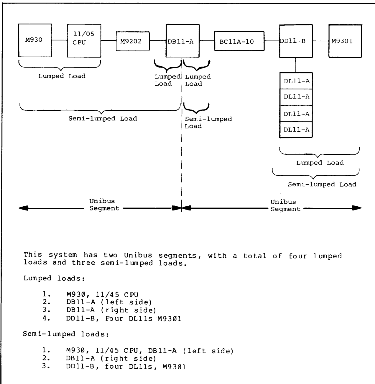
Figure 5-3. Semi-Lumped Loads (Example C)
