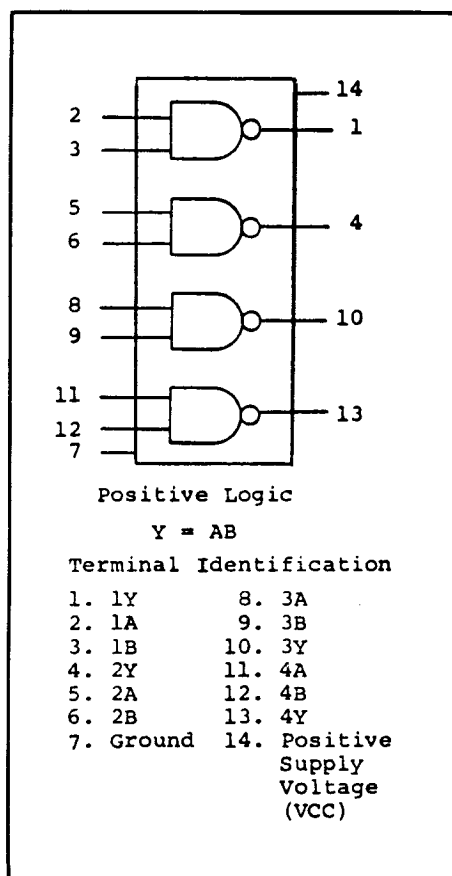
Figure 4-3. 8881 Bus Driver
