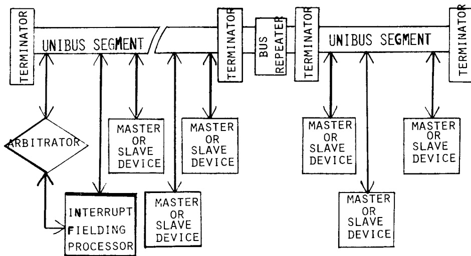
(A) TWO-SEGMENT UNIBUS
