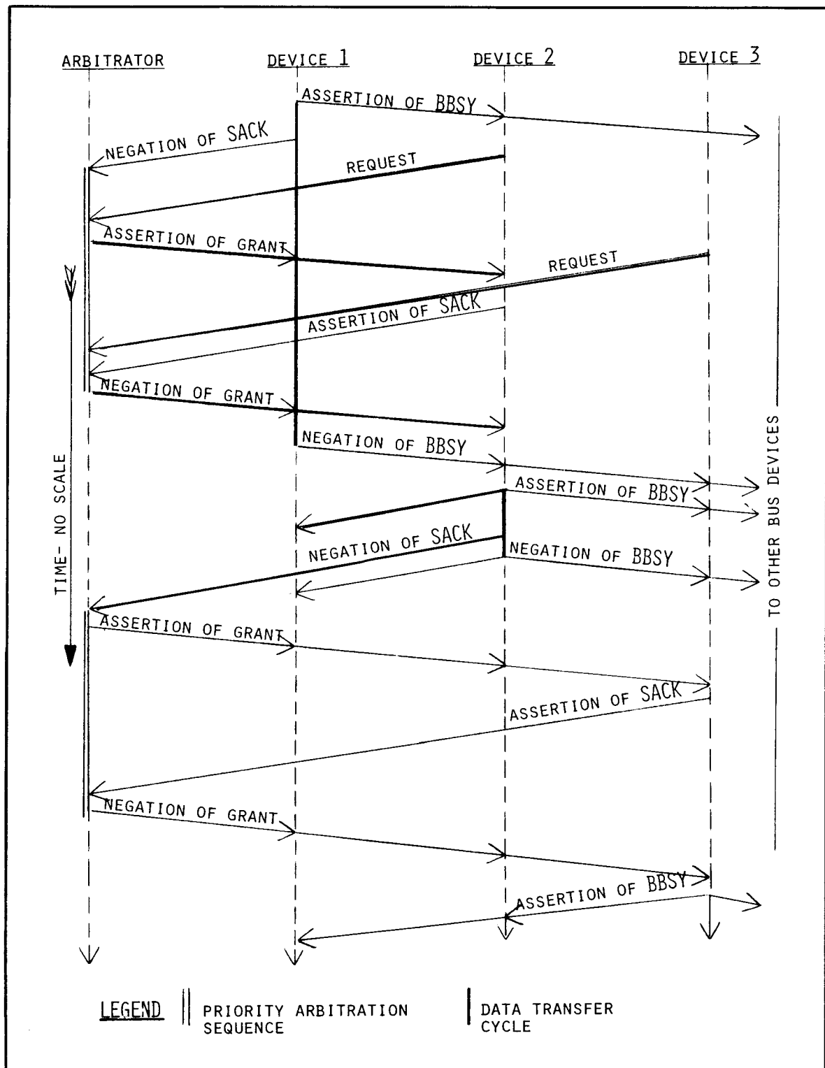
Figure 3-4. Typical Arbitration Sequence
