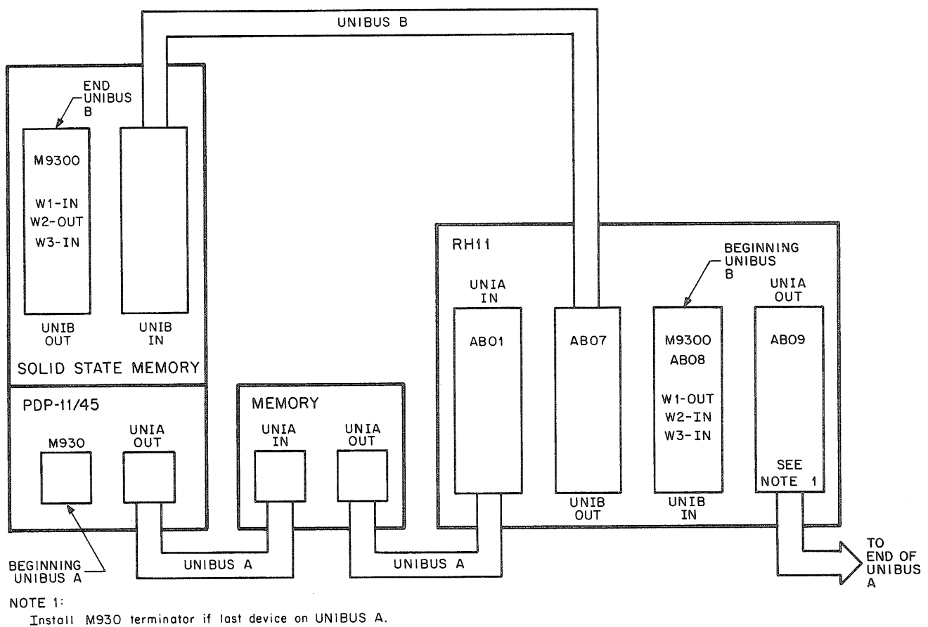
Figure 6-3 Dual Port Configuration - Memory on UNIBUS B
