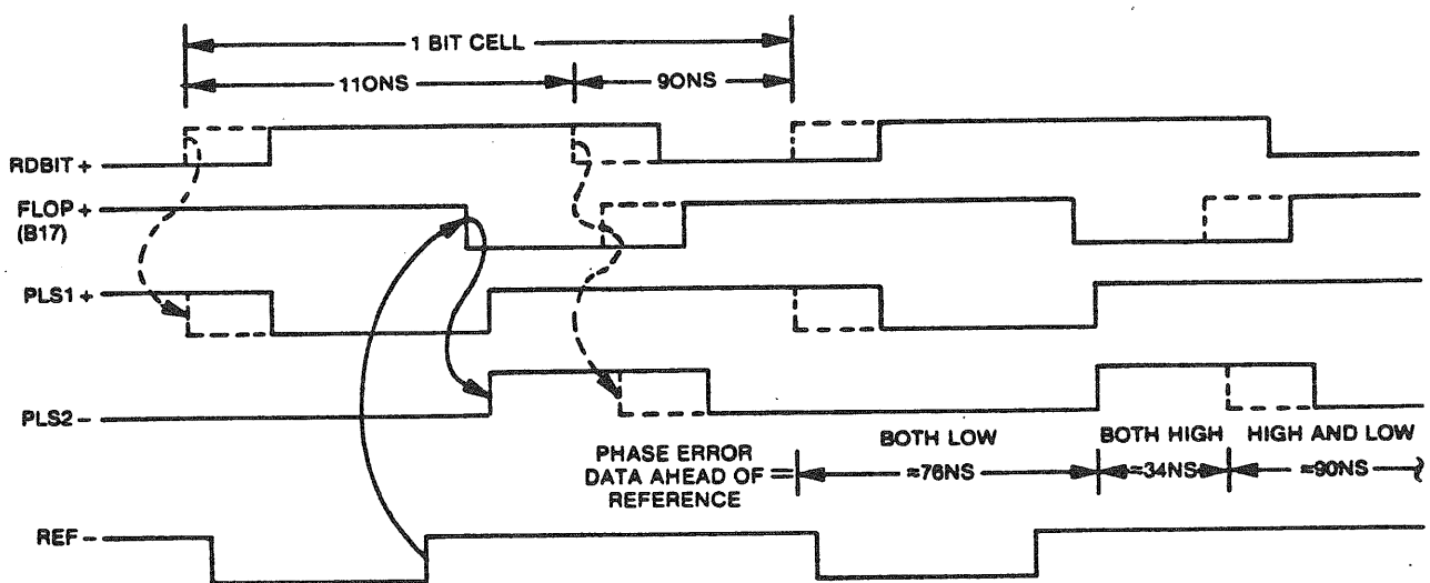
Figure 5-5. PLL Timing with Phase Error
