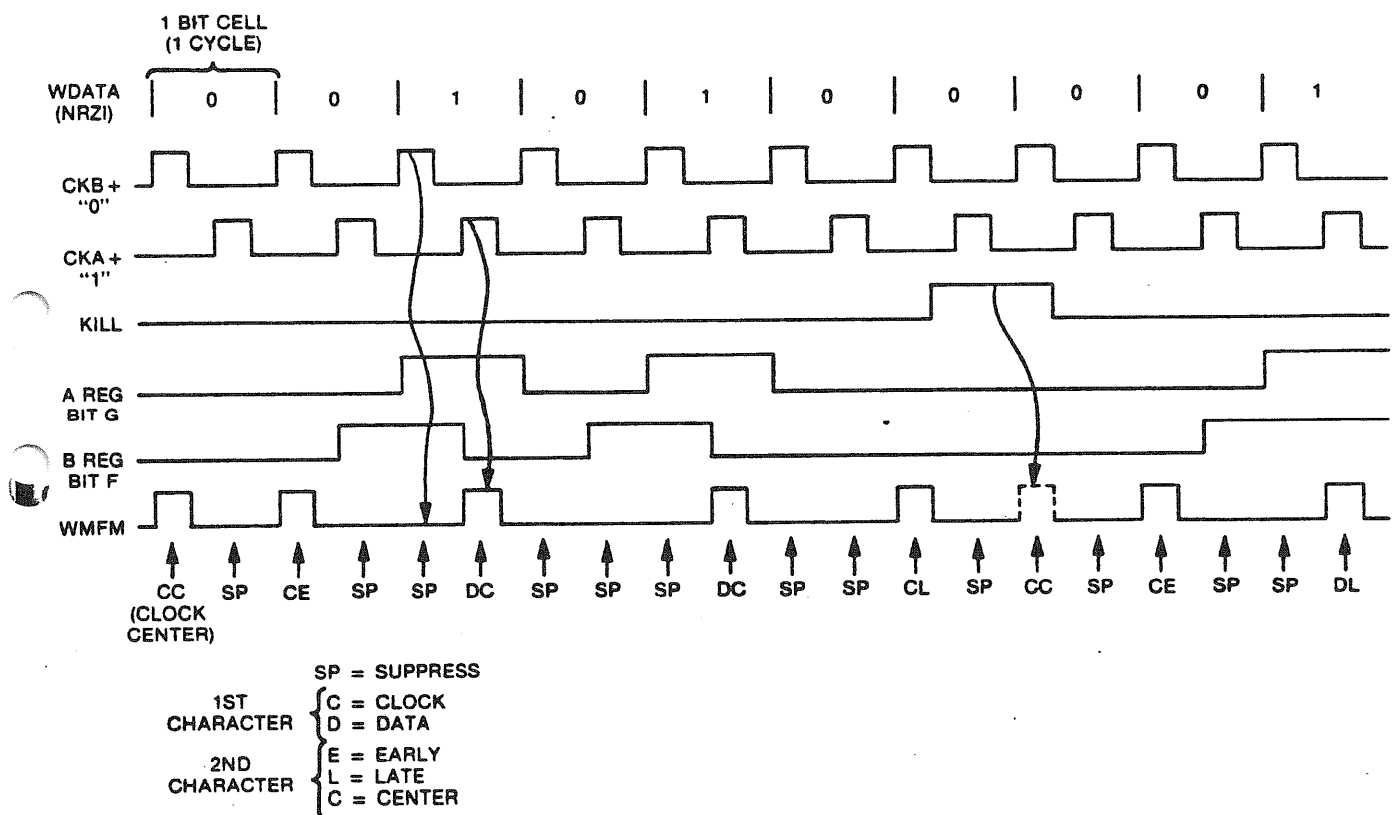
Figure 5-7. MFM Timing
