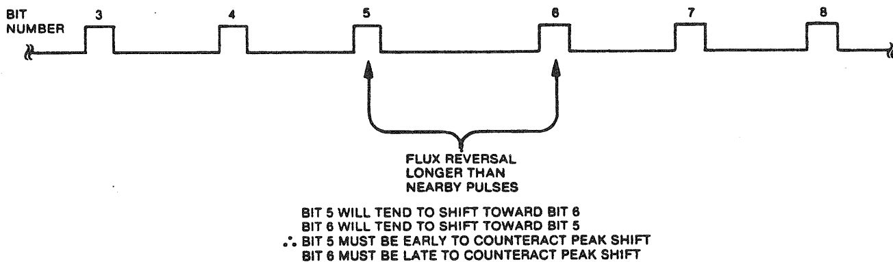
Figure 5-8. Peak Shift
