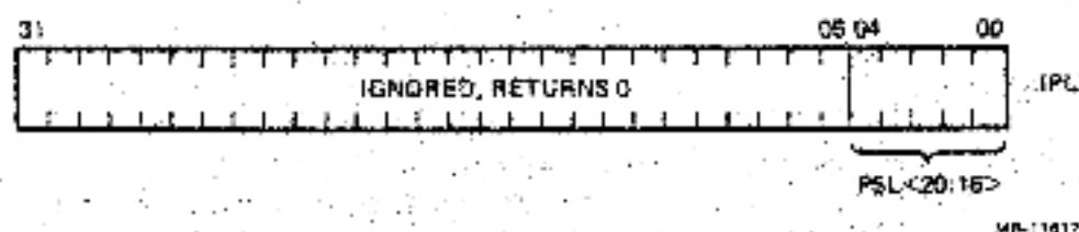
Figure 2-31 Interrupt Priority Level Register
