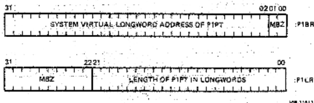
Figure 2-25 P1 Region Mapping Registers
