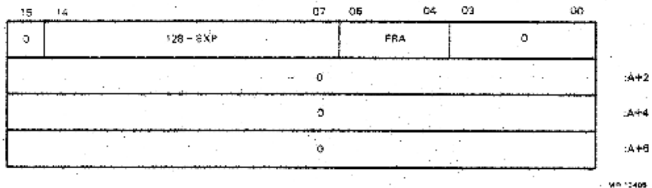
Figure 3-17 F_floating and D_floating Operand
