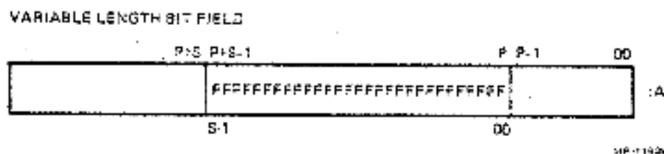
Figure 2-5 Variable Length Bit Field
