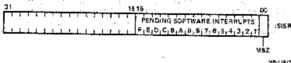
Figure 2-29 Software Interrupt Summary Register
