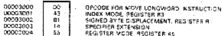
Figure 3-31 MOVL 8(X14(R1))[R3],R5 Move Longword
