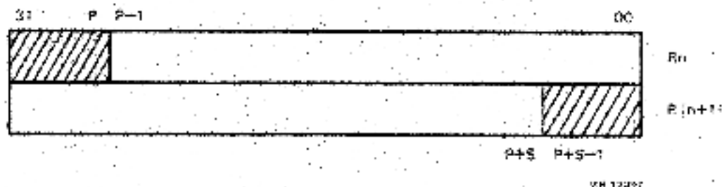
Figure 2-7 Variable Length Bit Field Across Registers
