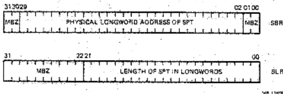
Figure 2-22 System Mapping Registers
