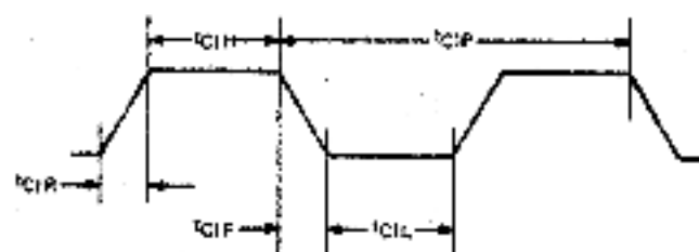
Figure A-1 CLK1 Timing
