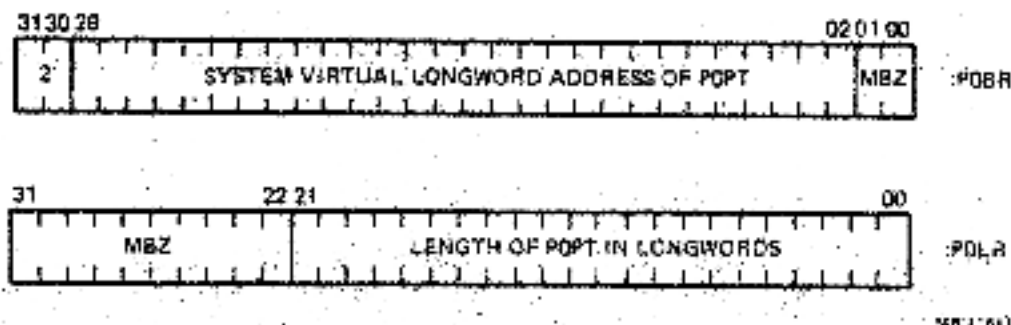
Figure 2-23 P0 Region Mapping Registers
