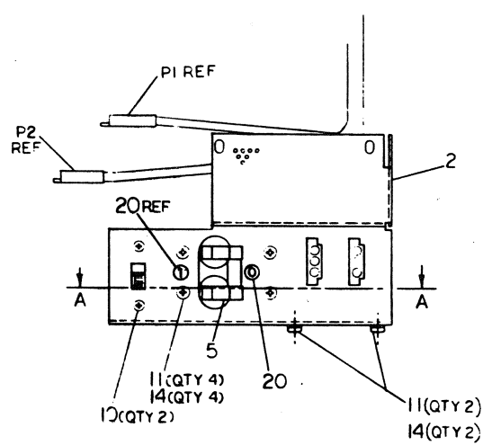
VIEW SHOWN WITH ITEM 1 (HAPPINESS) REMOVED FOR CLARITY
