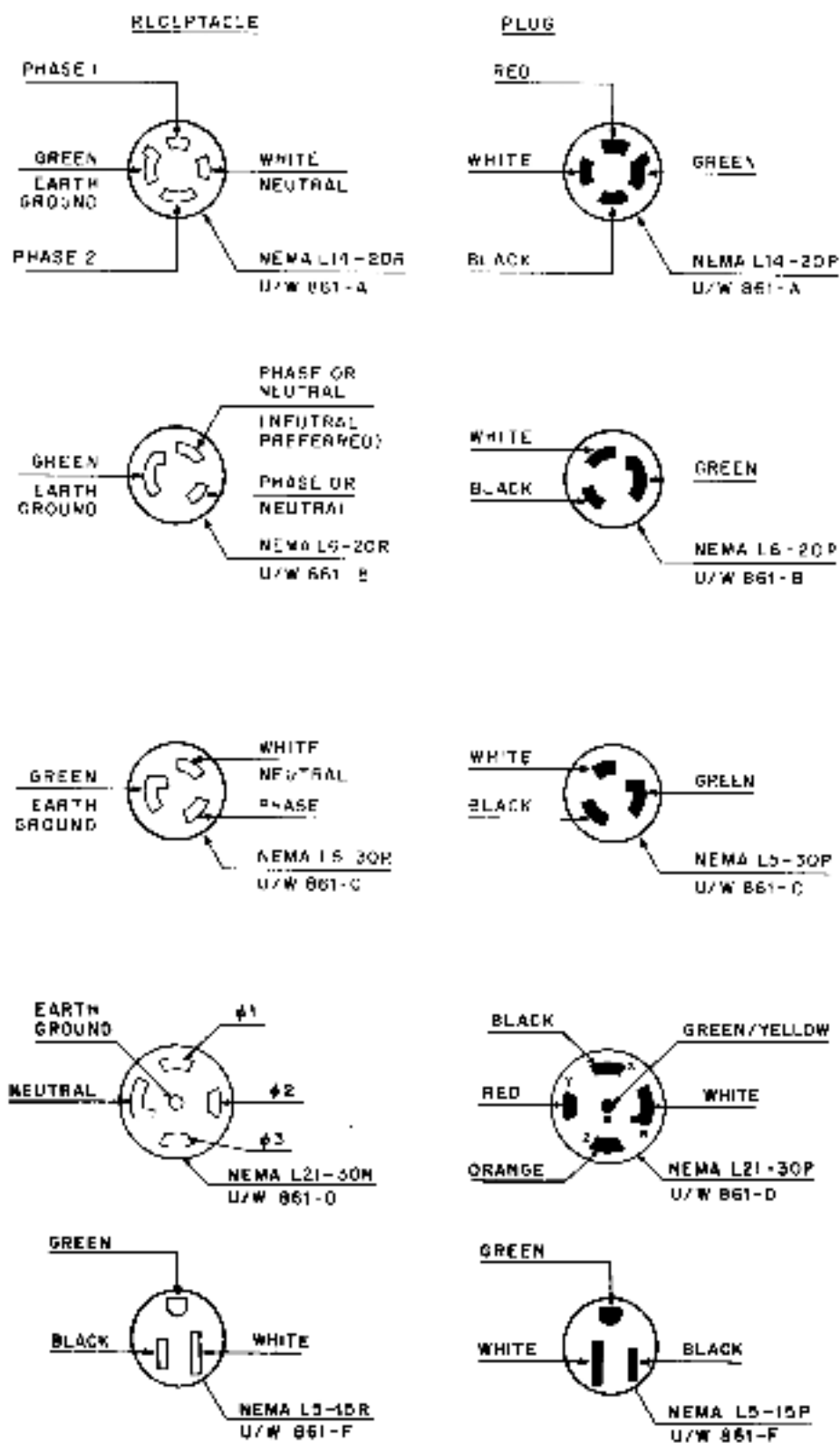
Figure 2-4 Connector Wiring
