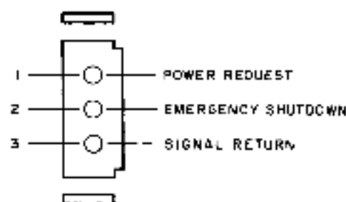
Figure 2-2 Signal Bus Connector
