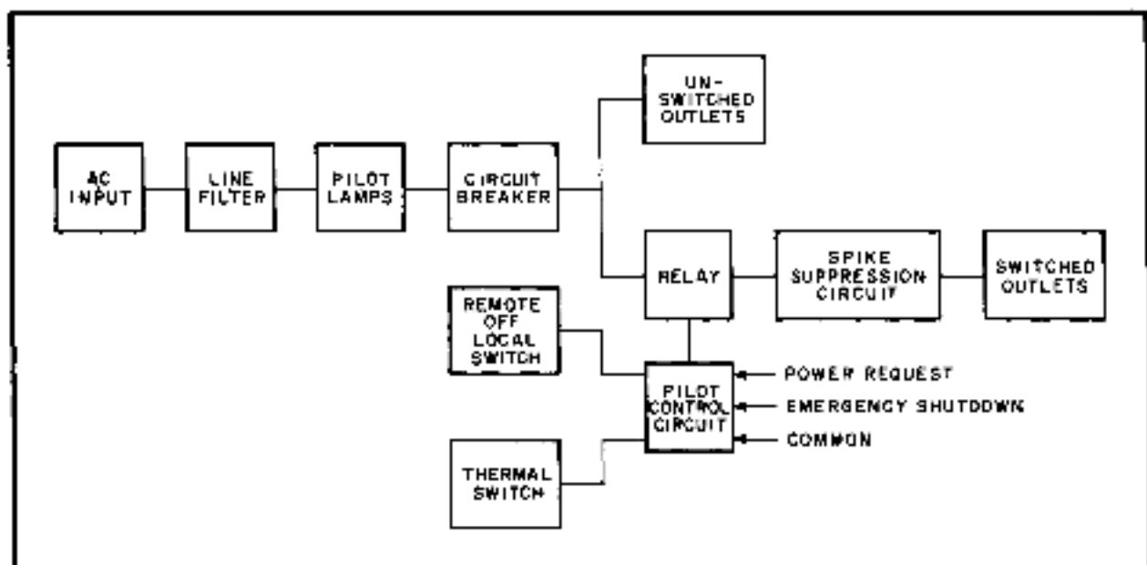
Figure 1-1 Simplified Block Diagram - 861-A,-B,-C,-D
