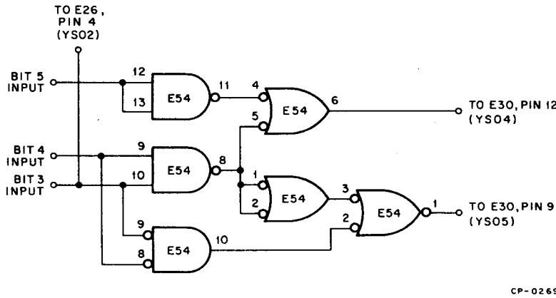
Figure 3-16 LOAD Y-ADDRESS Inhibit Logic
