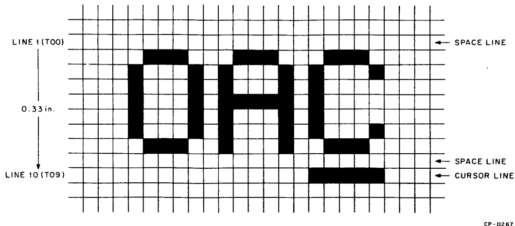
Figure 3-6 Raster Line Scanning and Timing
