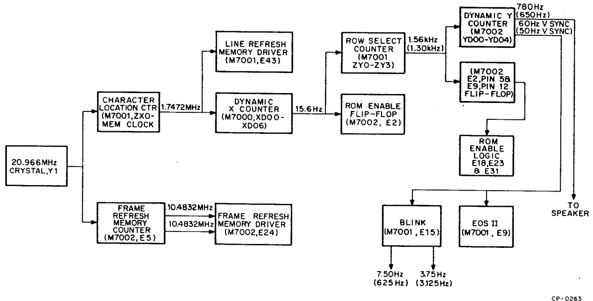
Figure 3-1 VT05 Basic Operating Frequencies
