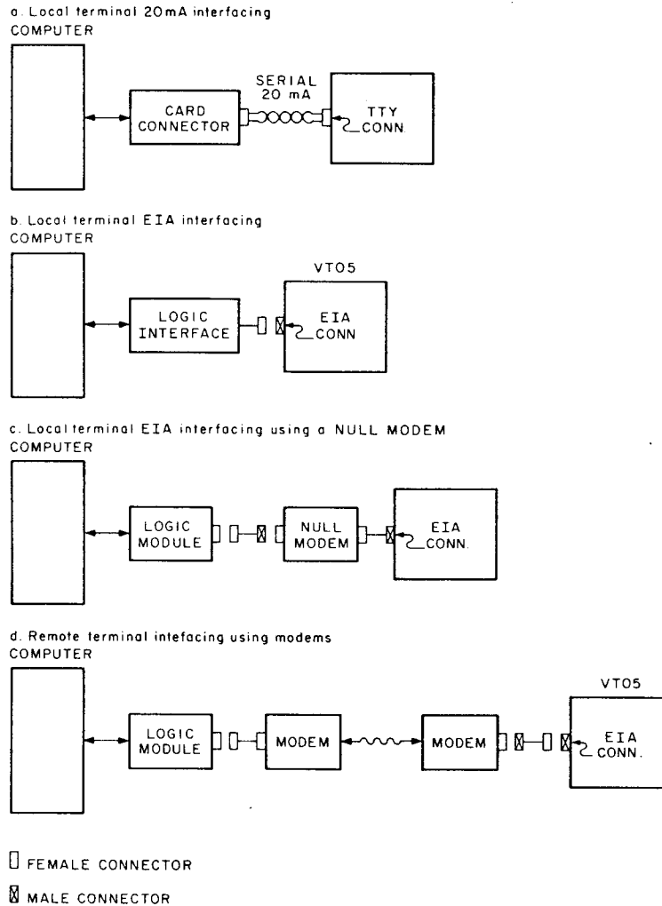
Figure 2-2 Typical VT05 Interfacing Configurations
