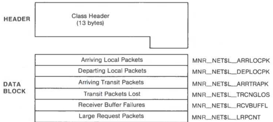
Figure MON-15 DECNET Class Record Format
