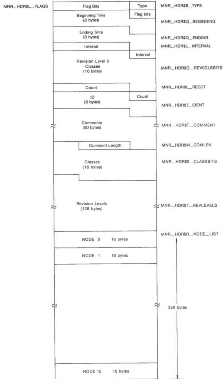
Figure MON-1 File Header Record Format
