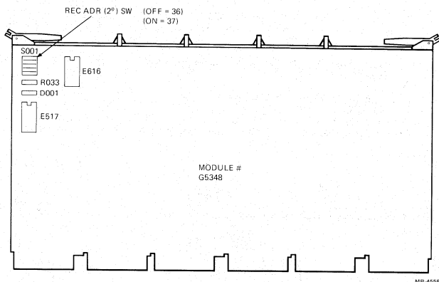
Figure 4 Recorder Address Switch Location
