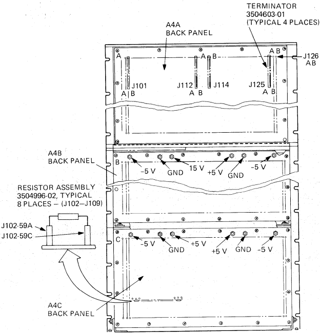
Figure 7 Terminator and Resistor Assemblies
