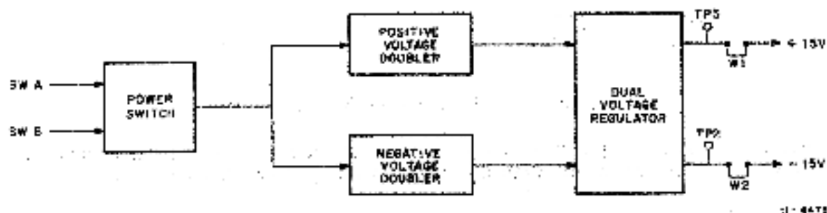
Figure 6-2 Analog Power Supply Block Diagram
