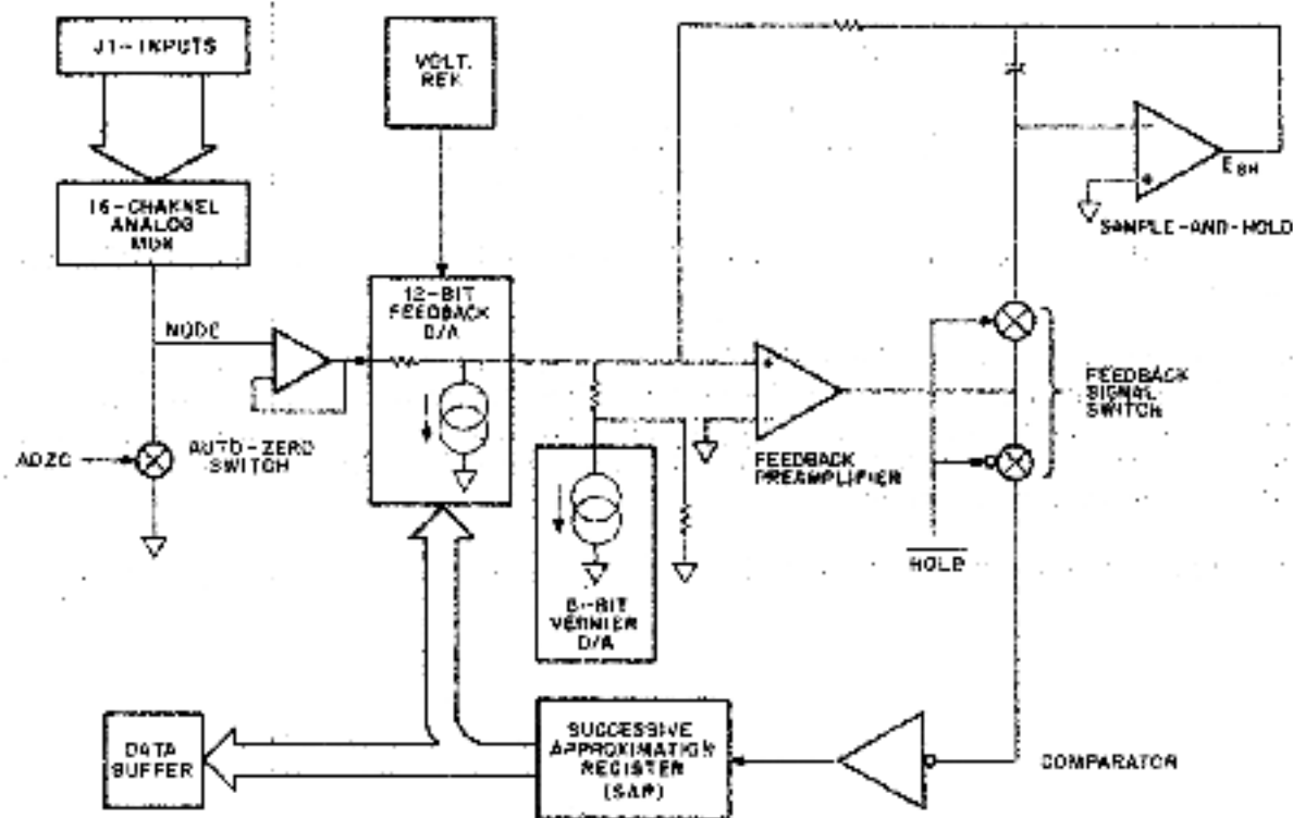
Figure 6-5 ADV11-A A/D Conversion Circuit Block Diagram
