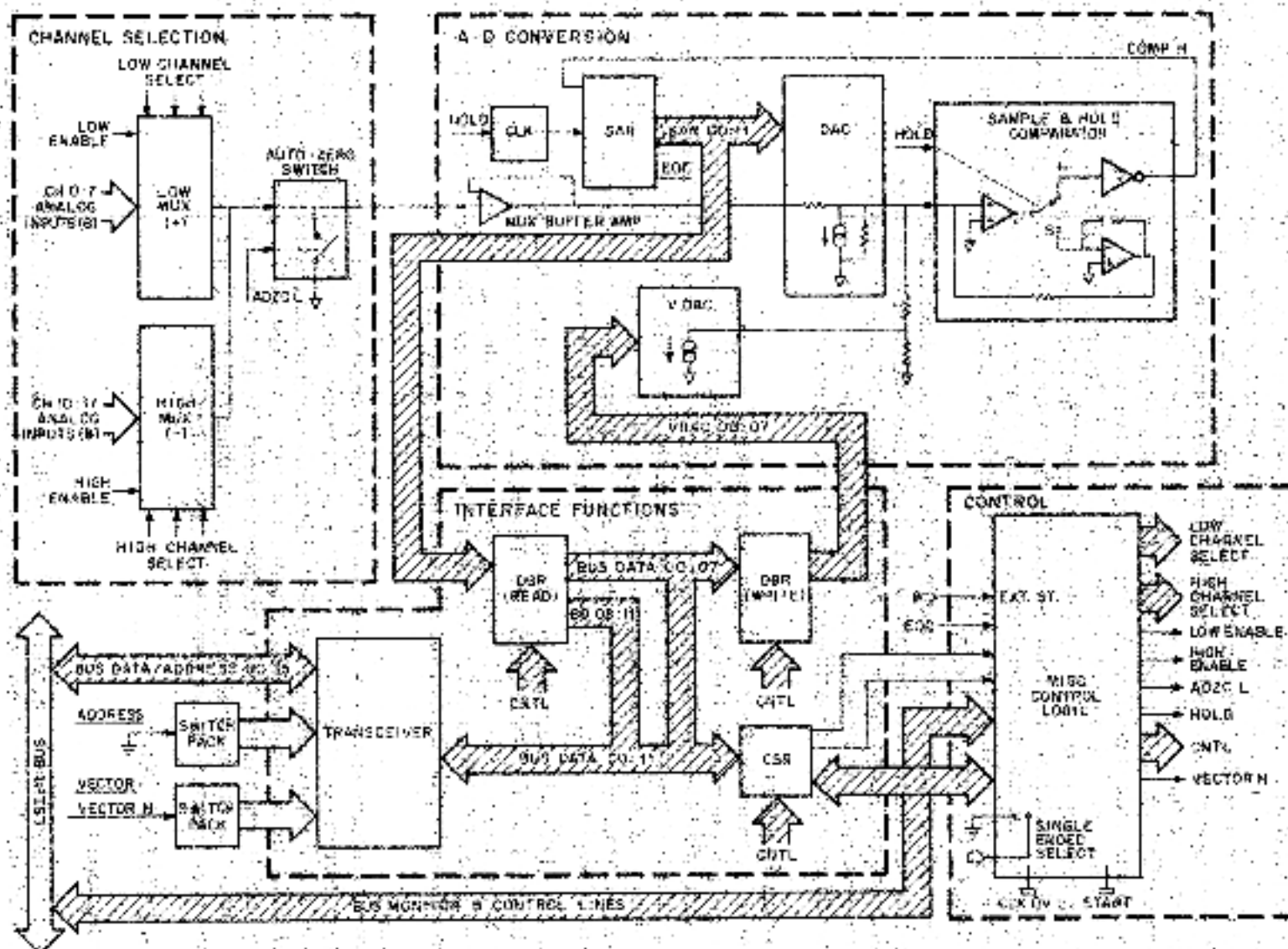
Figure 2-1 ADV11-A Functional Block Diagram
