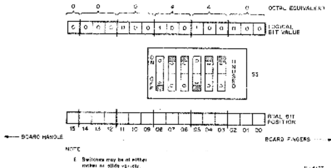
Figure 3-6 KWV11-A Vector Address Switches (Set for 000440)
