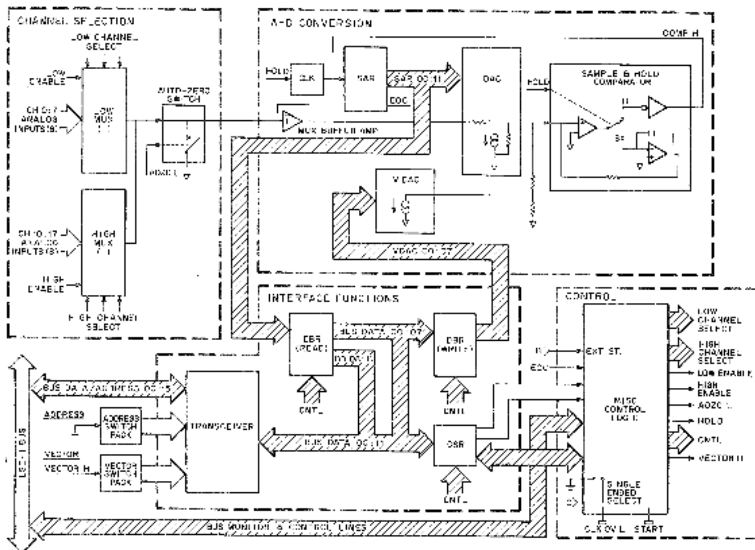
Figure 2-1 ADV11-A Functional Block Diagram
