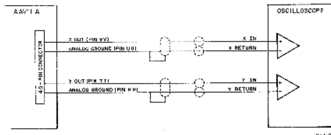
Figure 4-6 Connection to Oscilloscope with Differential Input
