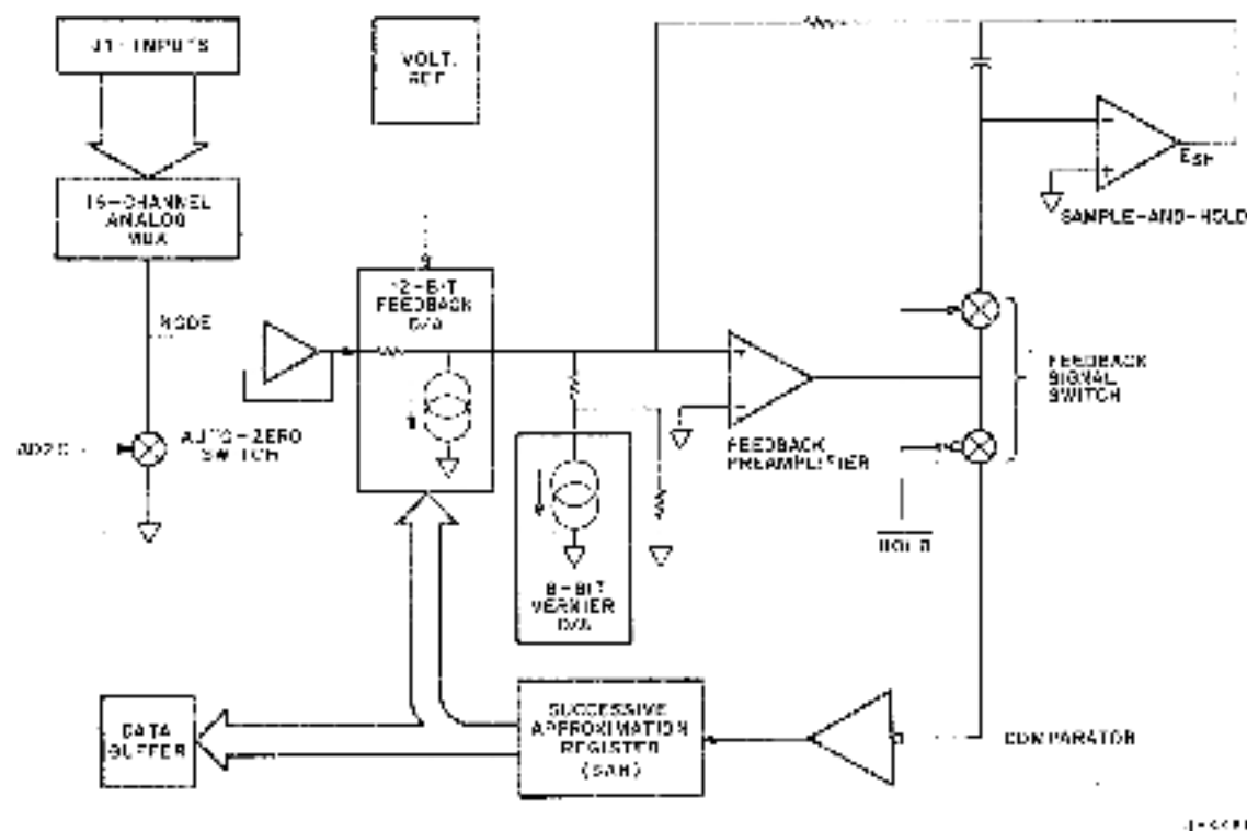
Figure 6-5 ADV11-A A/D Conversion Circuit Block Diagram
