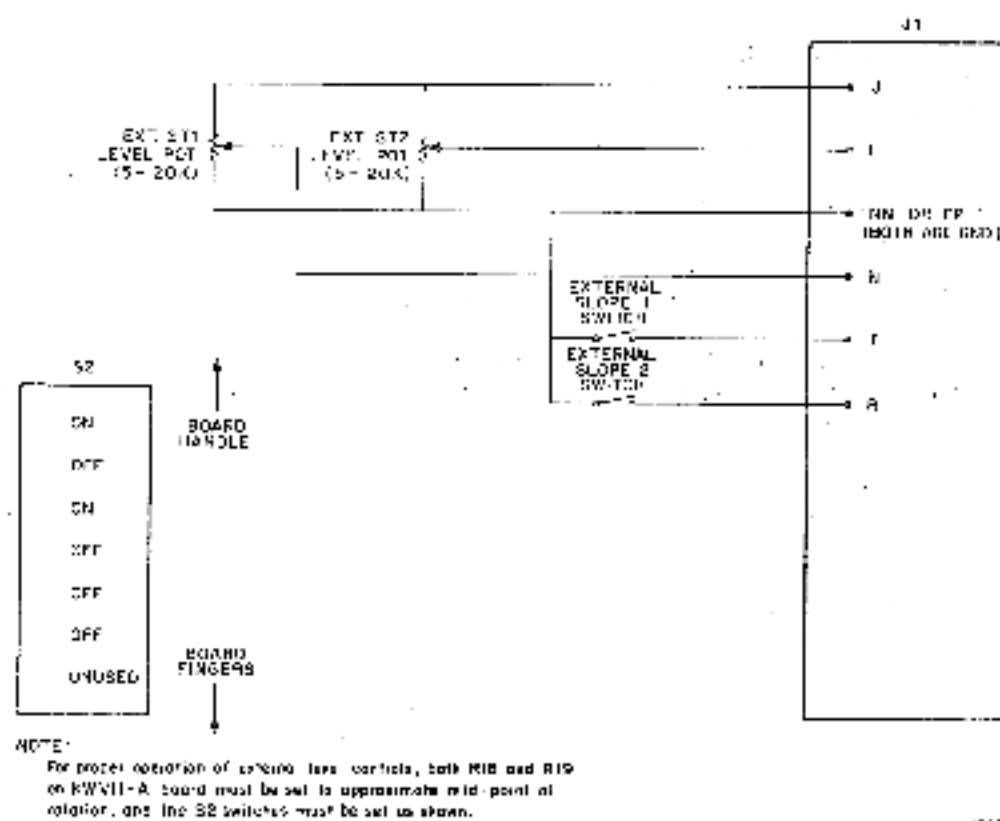
Figure 3-3 Connecting External User-Supplied Slope and Level Controls
