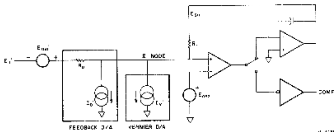
Figure 6-7 A/D During Conversion
