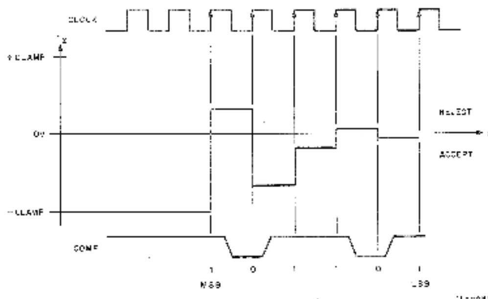
Figure 6-8 \Sigma Node During Conversion
