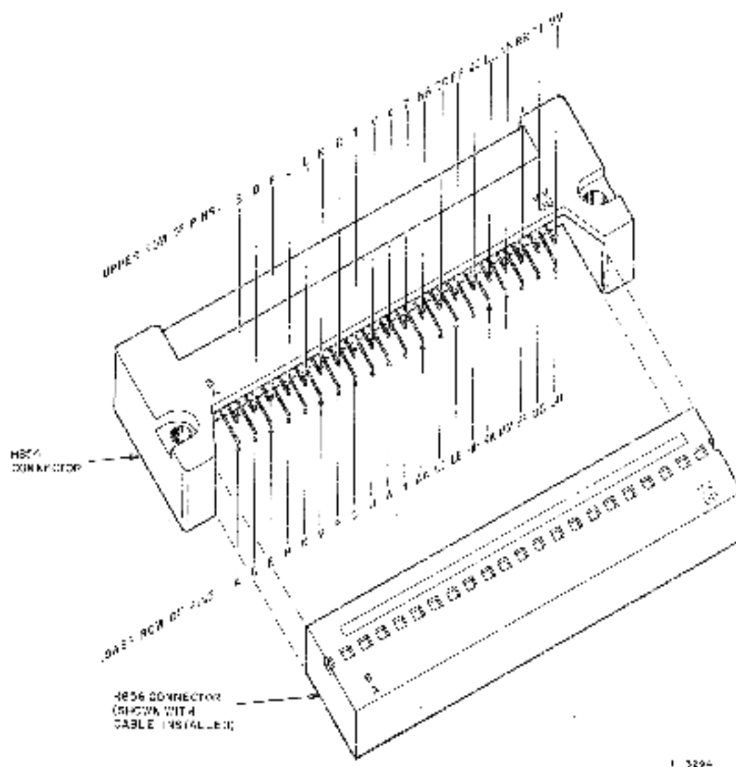
Figure S-5 J1 or J2 Connector Pin Locations
