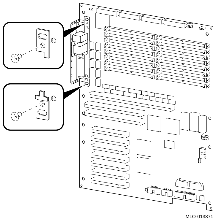
Figure 2-17 Attaching EMI Clips
