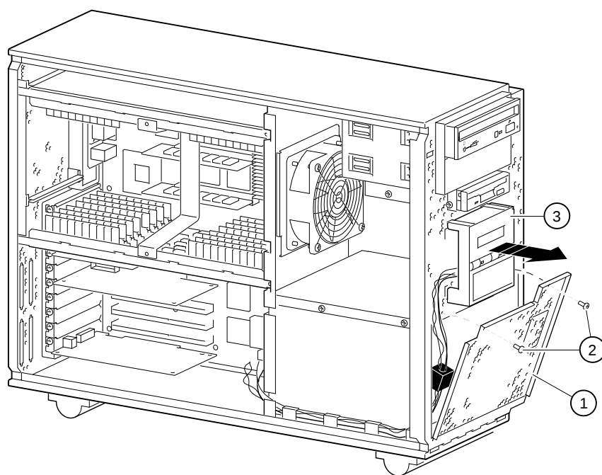
Figure 2-10 Removing Power Supply Cover and OCP
