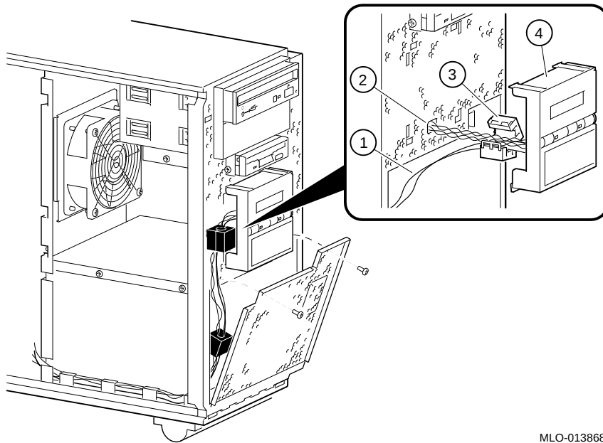
Figure 2-13 Attaching Ferrite Bead to OCP Cables
