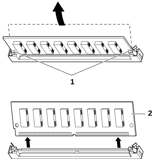
Figure 2-2 Removing a Memory Module
