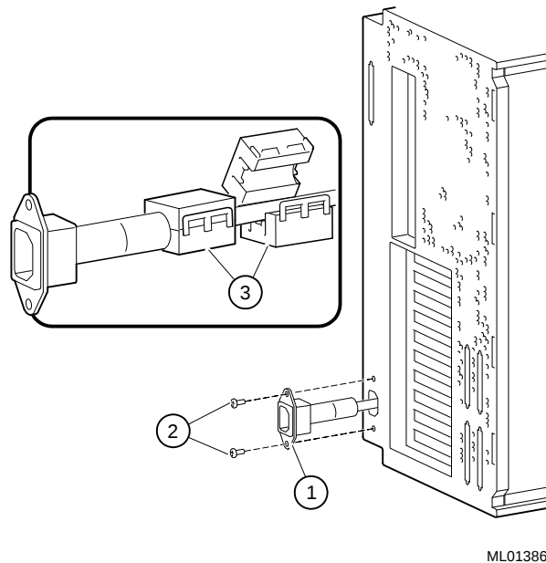
Figure 2-12 Attaching Ferrite Beads to Harness
