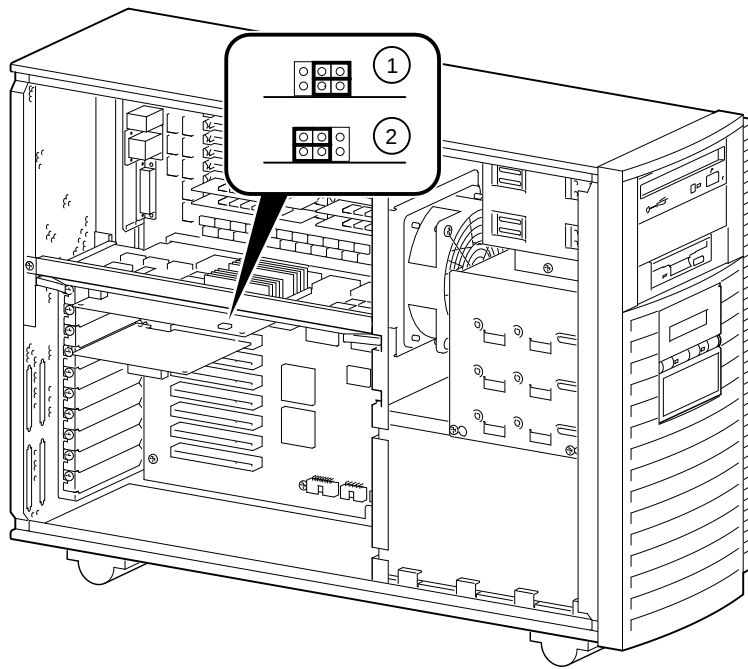
Figure 2-21 Moving Sound Card Jumpers
