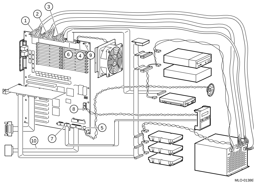
Figure 2-25 Reconnecting Cables
