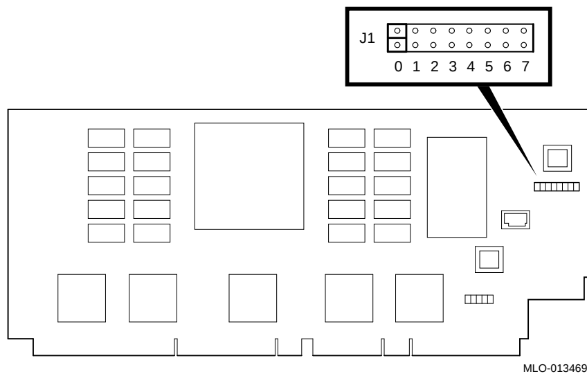
Figure 2-26 J1 Jumper on the CPU Card (Normal Position)
