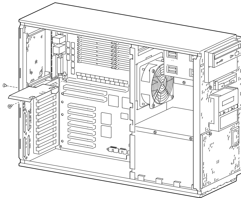
Figure 2-18 Installing the EMI Shield
