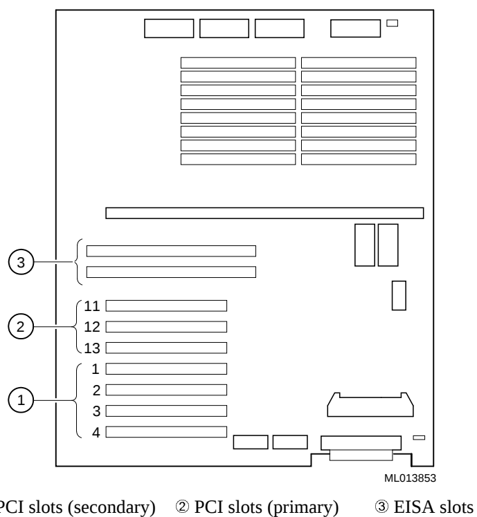
Figure 2-22 Option Module Slots on the 600A System Board
