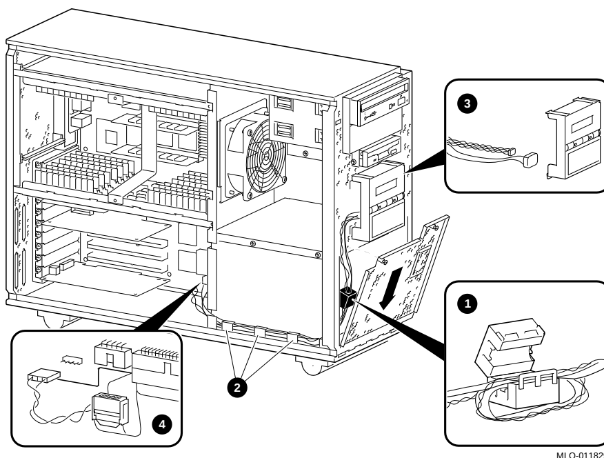
Figure 2-15 Rerouting the OCP Cable
