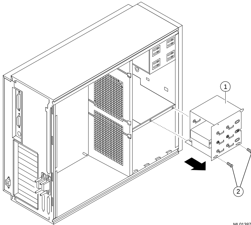
Figure 2-5 Removing the Drive Assembly
