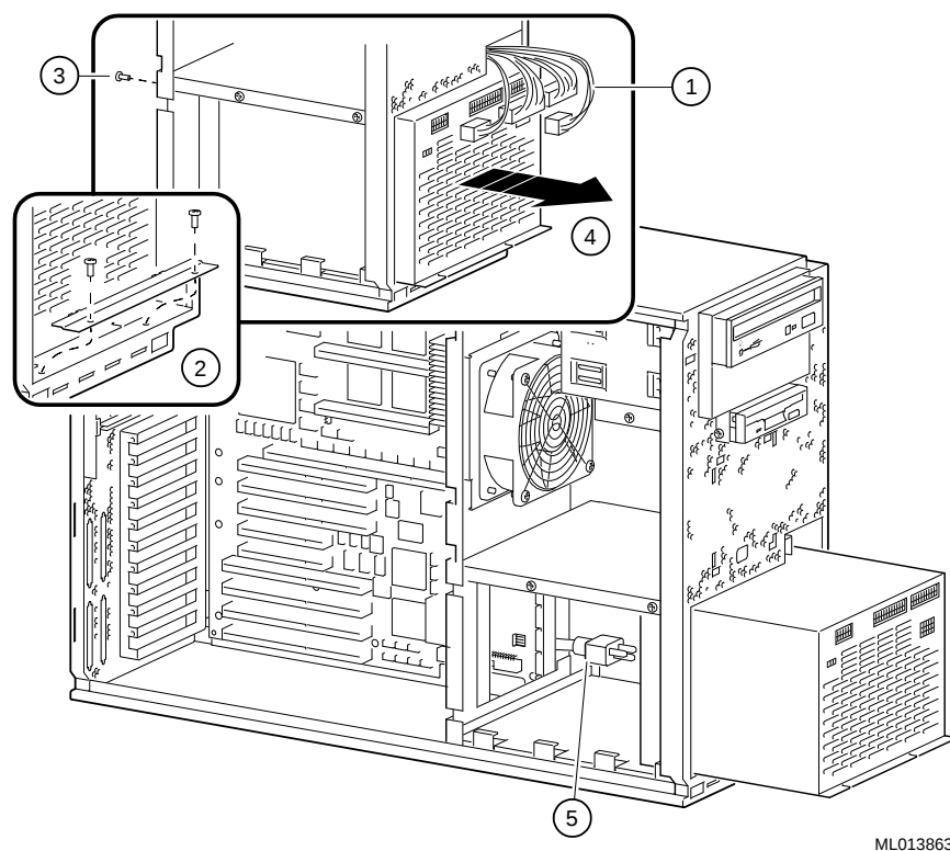
Figure 2-11 Removing Power Supply
