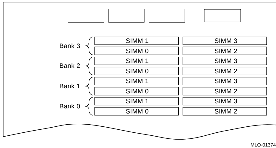
Figure 2-19 Memory Banks and Connectors
