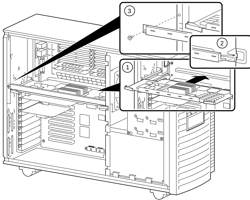
Figure 2-24 Installing CPU Card
