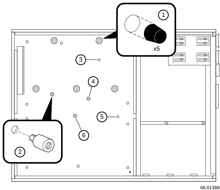
Figure 2-7 Rubber Bumpers and Metal Standoffs
