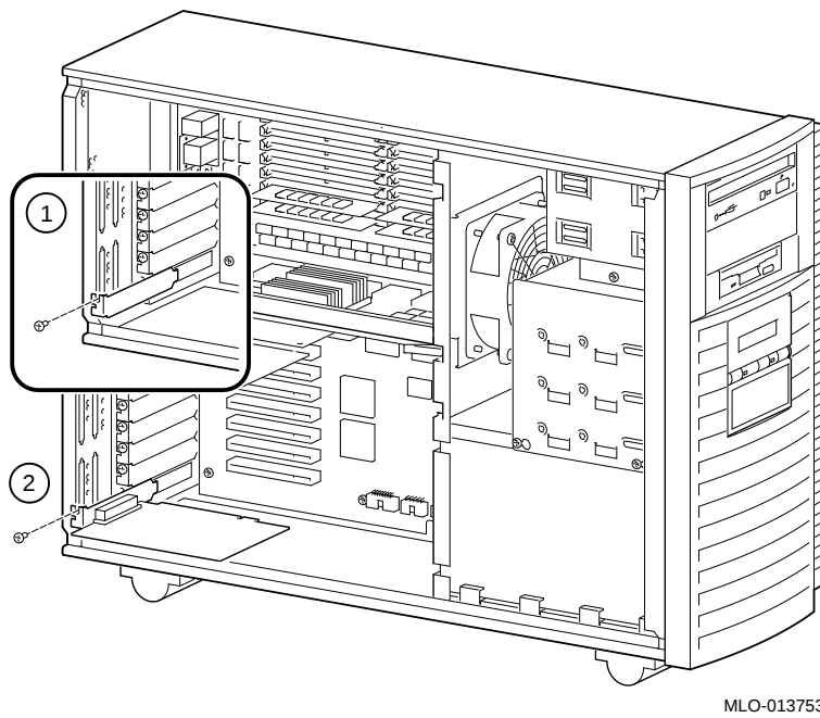
Figure 2-23 Installing Option Modules
