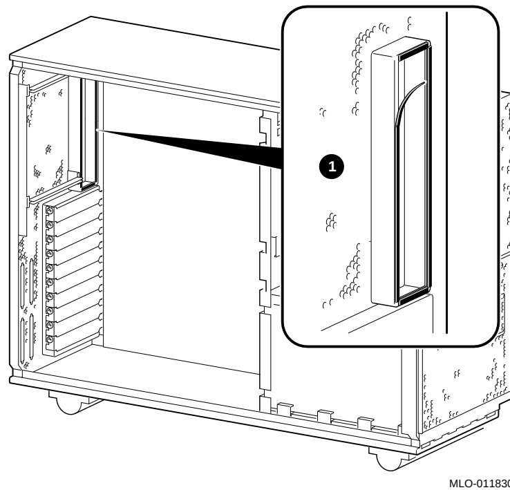
Figure 2-16 Installing the EMI Gaskets
