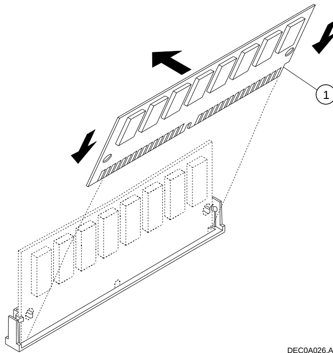
Figure 2-20 Installing a Memory Module
