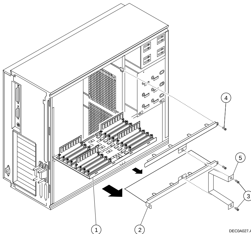
Figure 2-1 Removing a Memory Tower Board
