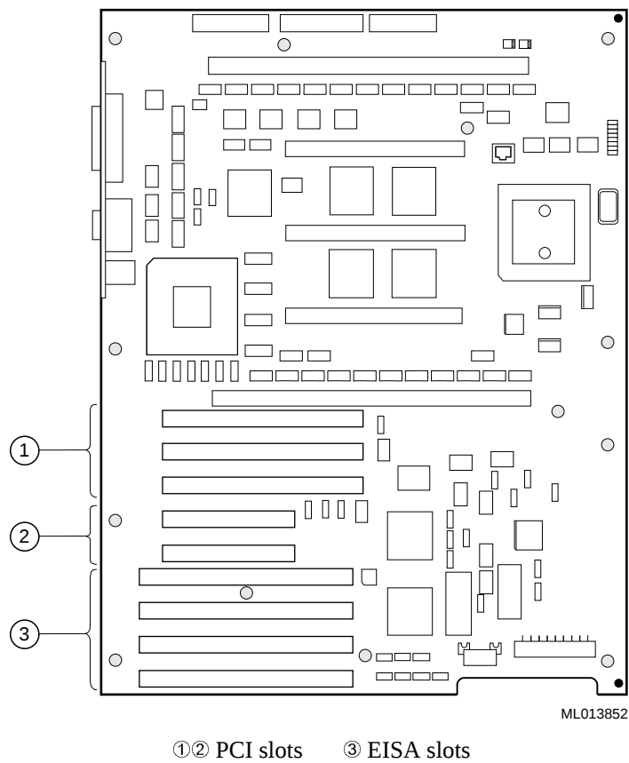
Figure 2-4 Option Module Slots on the Model 600 System Board
