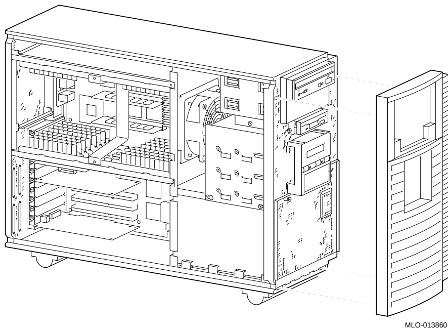
Figure 2-9 Removing the Front Panel
