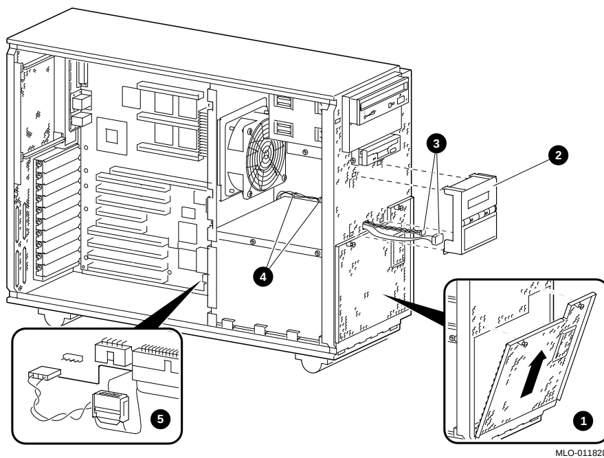
Figure 2-14 Removing the OCP Cables
