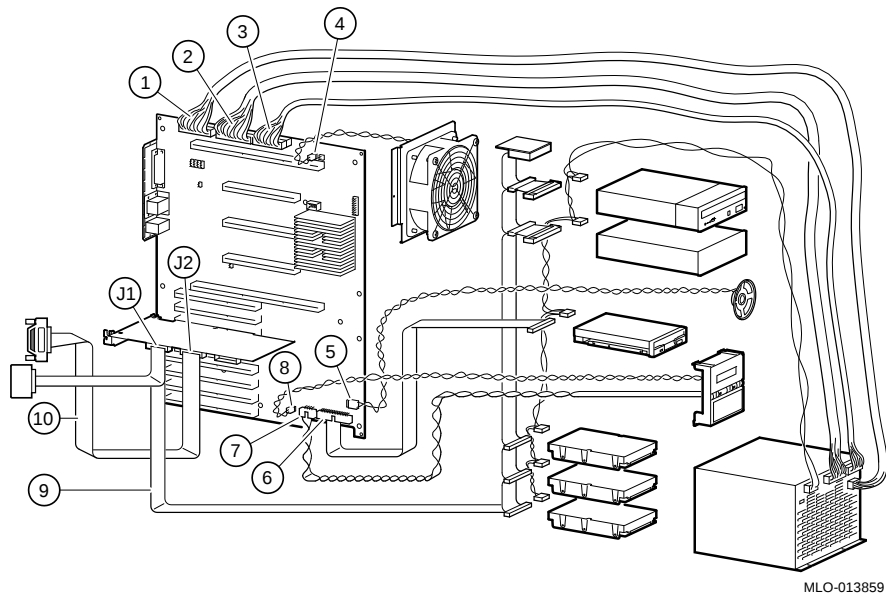
Figure 2-6 Disconnecting Cabling
