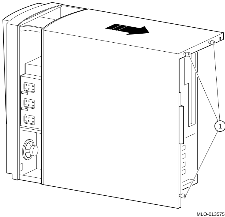
Figure 1-1 Unlocking and Removing the System Cover
