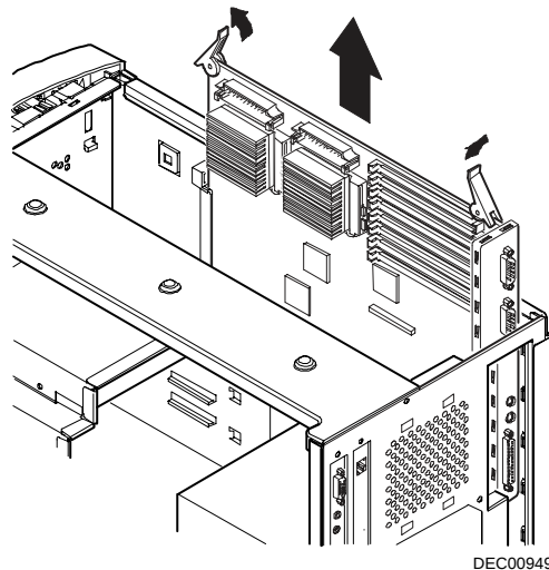
Figure 1-2 Removing the MLB
