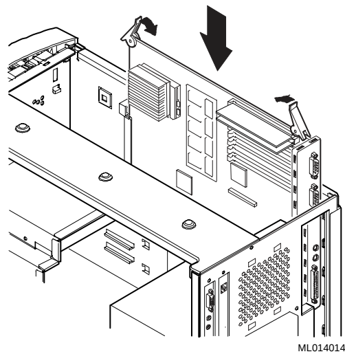
Figure 1-4 Installing the New MLB
