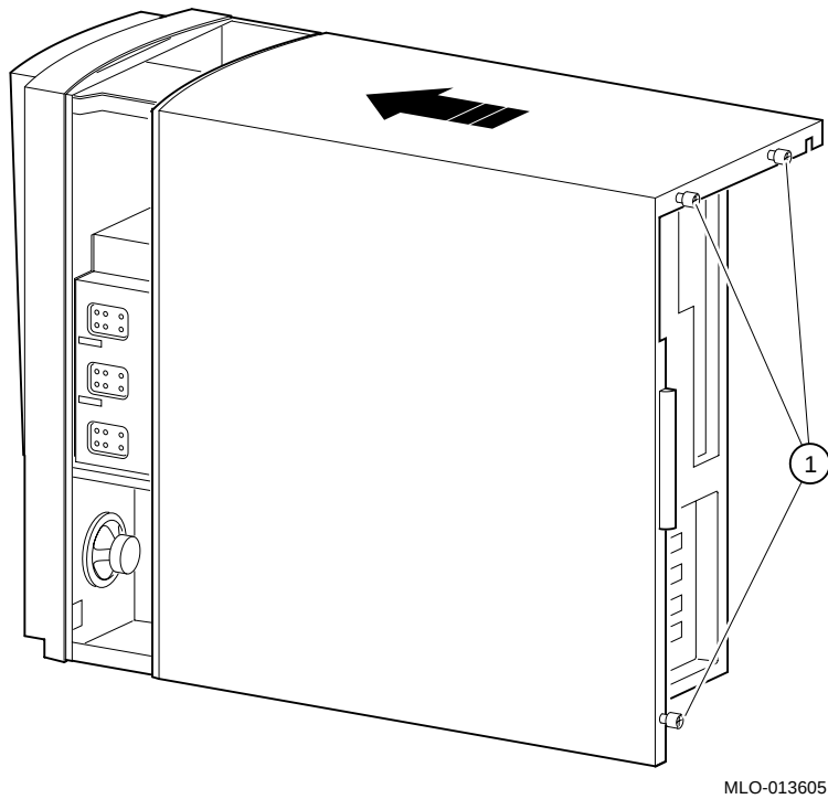
Figure 1-7 Replacing the Cover
