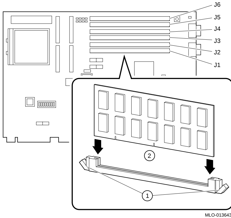
Figure 1-3 Installing the Memory
