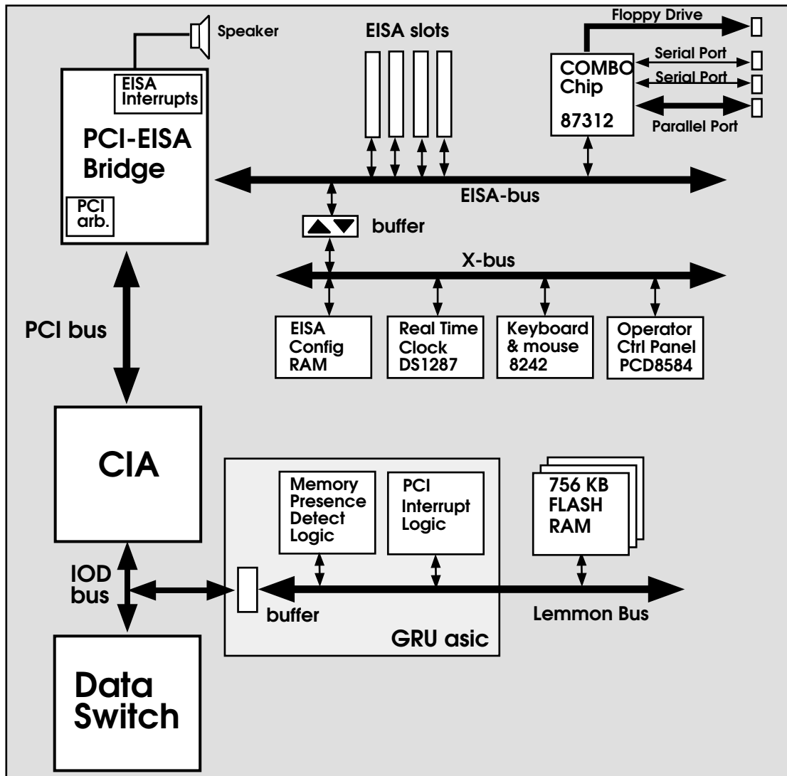
Figure 10-1 AlphaStation 600 Standard I/O Busses
