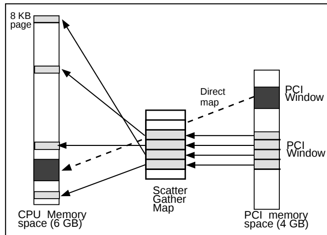
Figure 2-7 Scatter/Gather TLB
