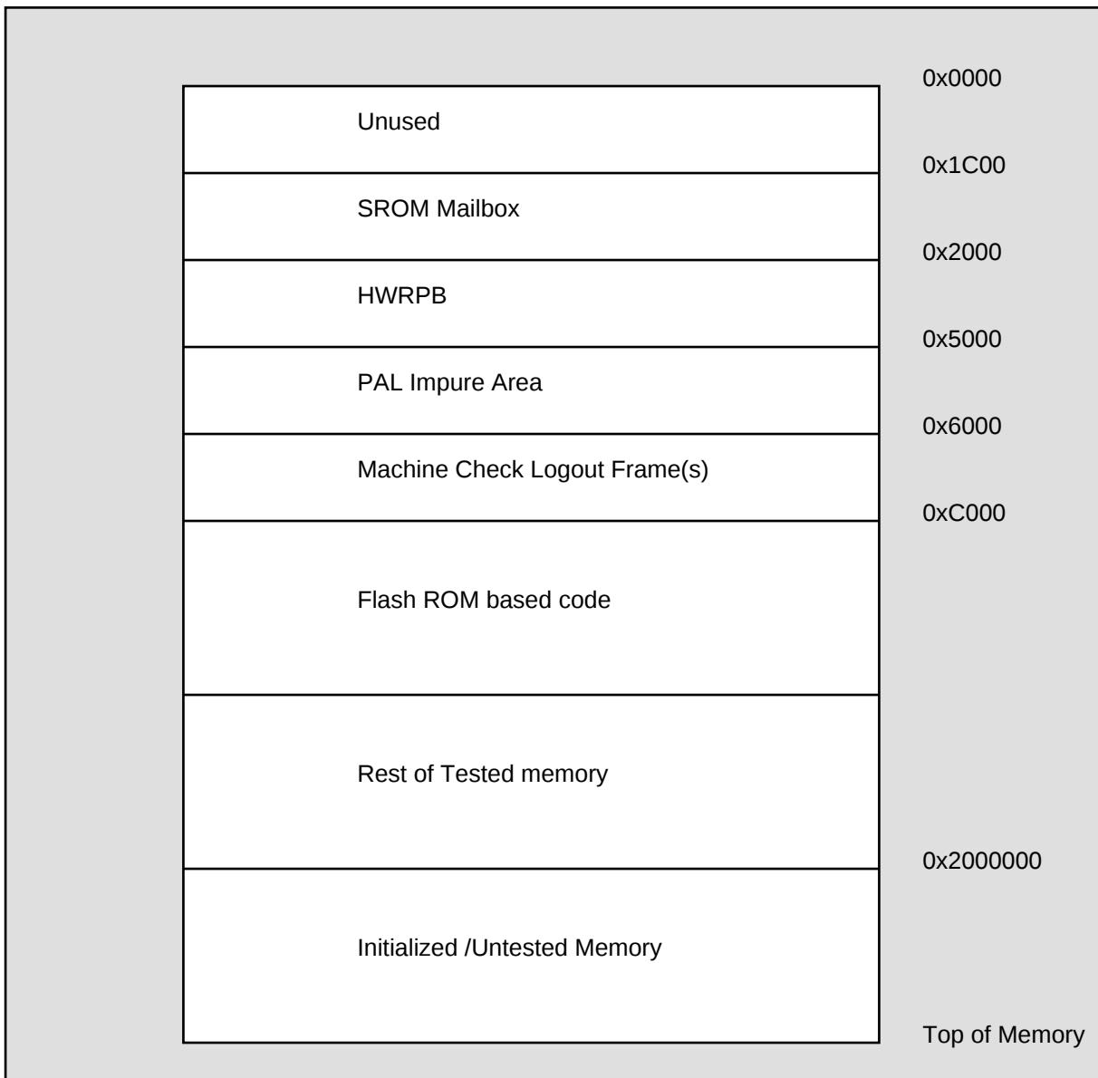
Figure 9-1 AlphaStation 600 Memory Map After Initialization
