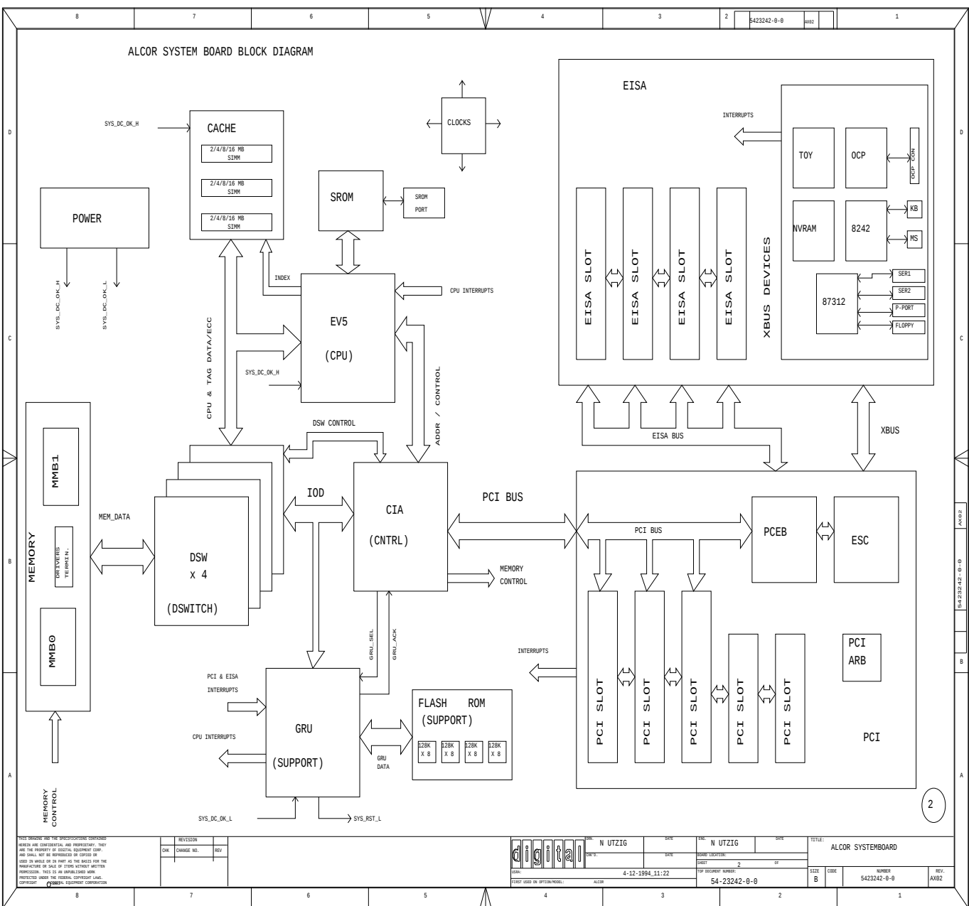
Figure 6-1 AlphaStation 600 System Block Diagram
