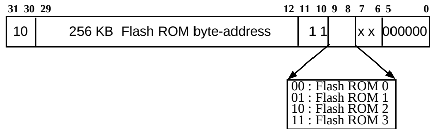
Figure 2-8 Flash ROM Address scheme
