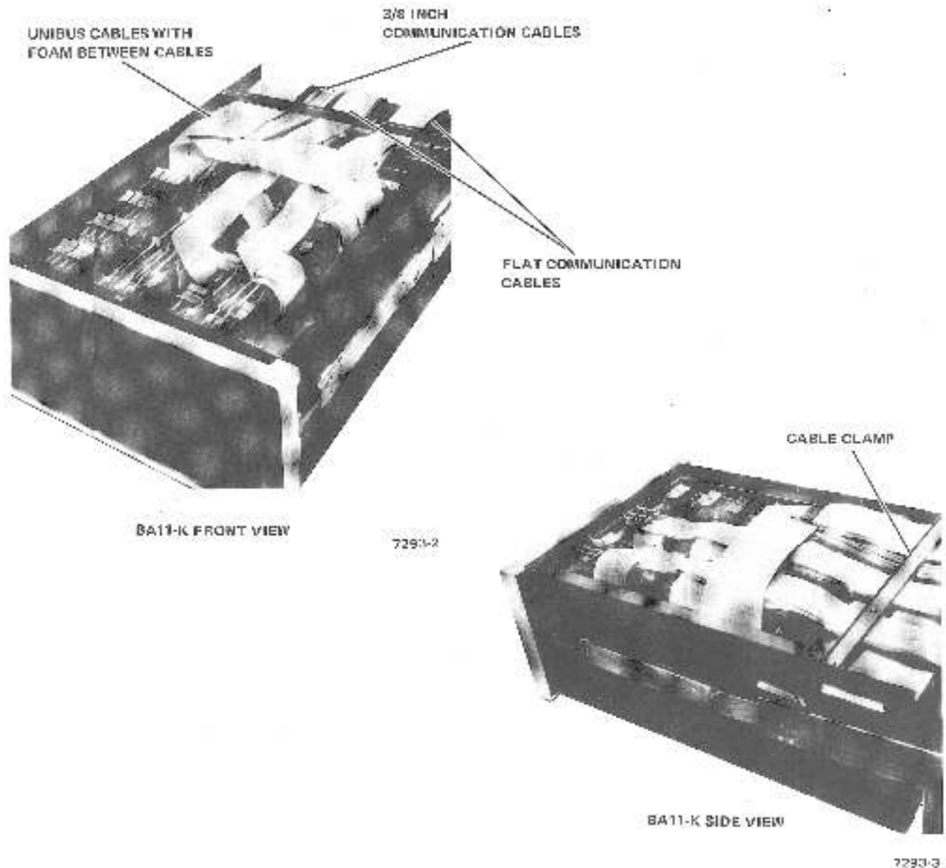
Figure 2-5 Cable Routing
