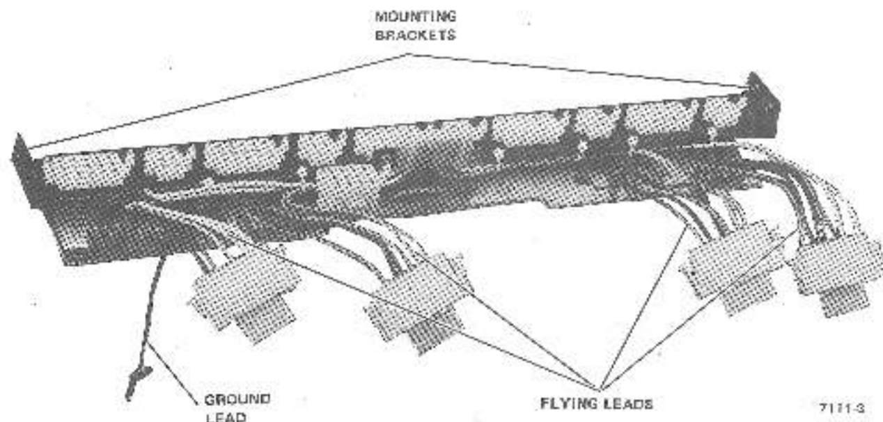
Figure 4-10 Power Distribution Board
