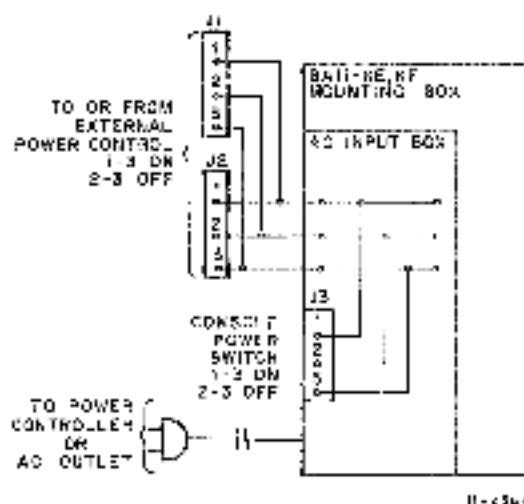
Figure 5-3 Power Control
