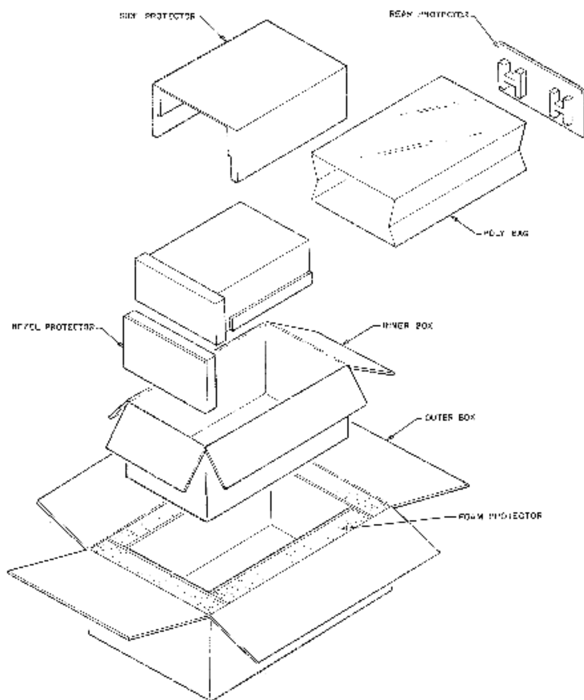
Figure 5-1 BA11-K Packaging
