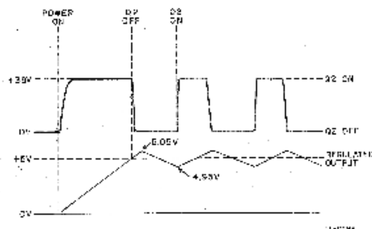
Figure 3-10 H744 Regulator Waveforms
