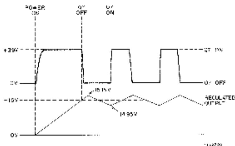
Figure 3-7 5411086 Regulator Waveforms
