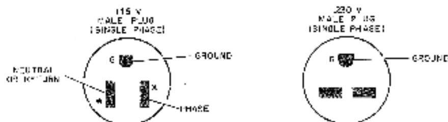
CONNECTOR SPECIFICATIONS
