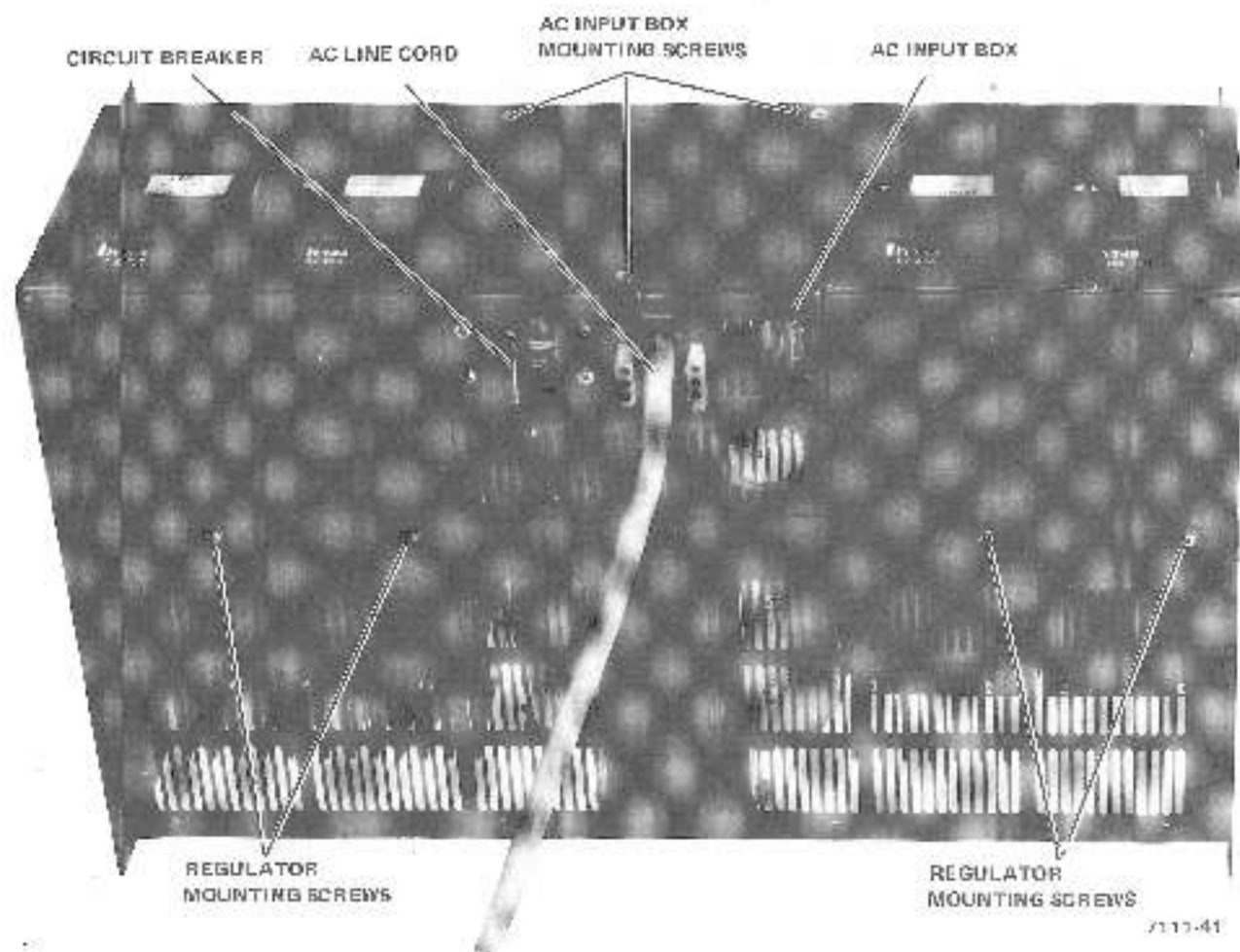
Figure 4-6 H765 Power System
