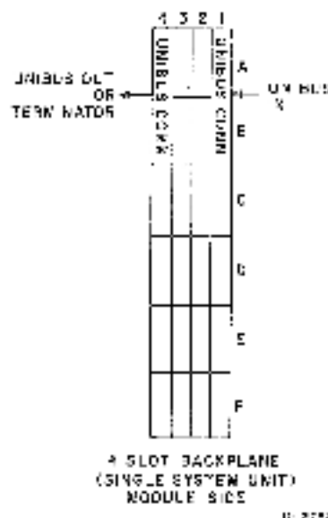
Figure 2-1 Standard Unibus Connection
