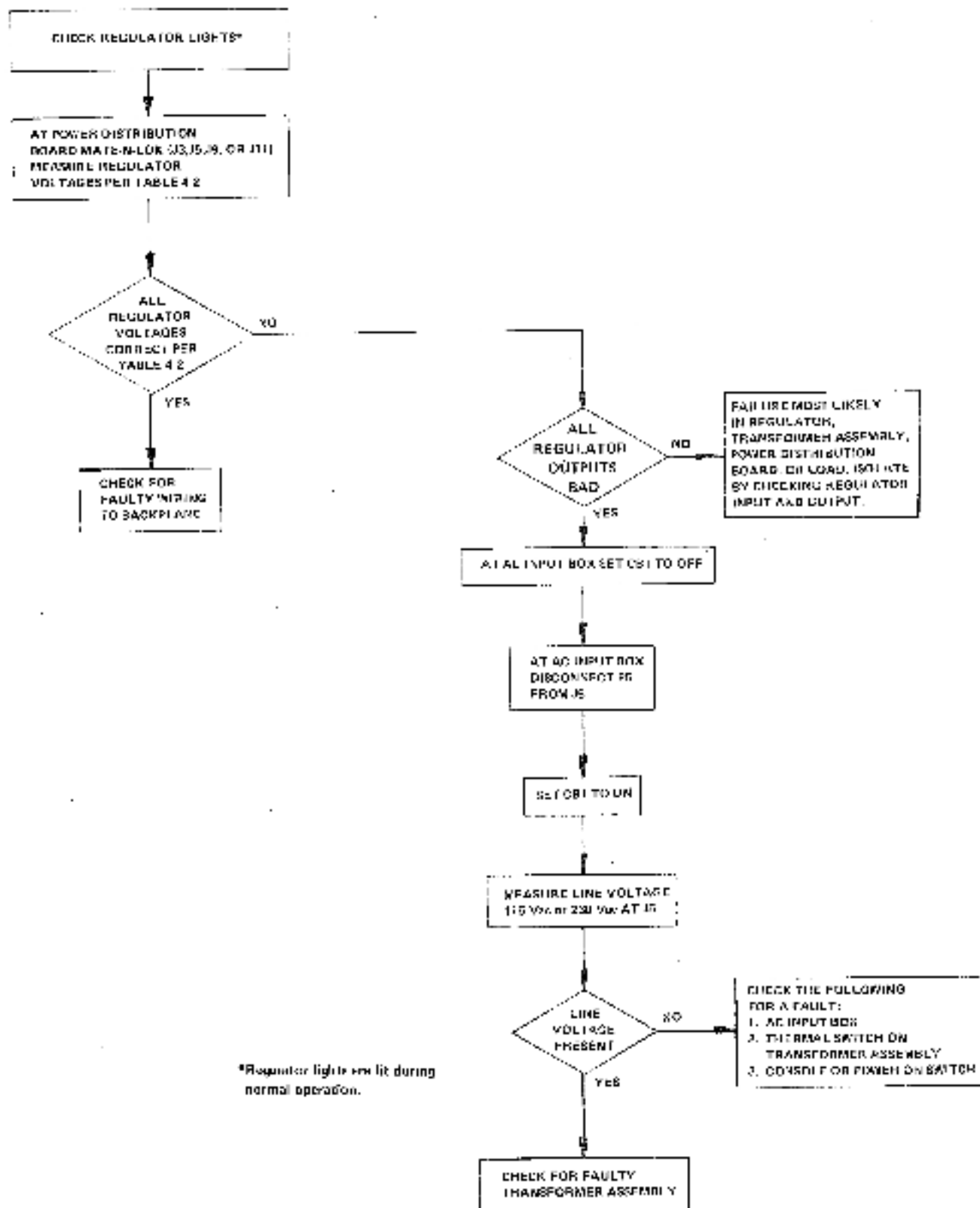
Figure 4-1 H765 Fault Isolation Flowchart
