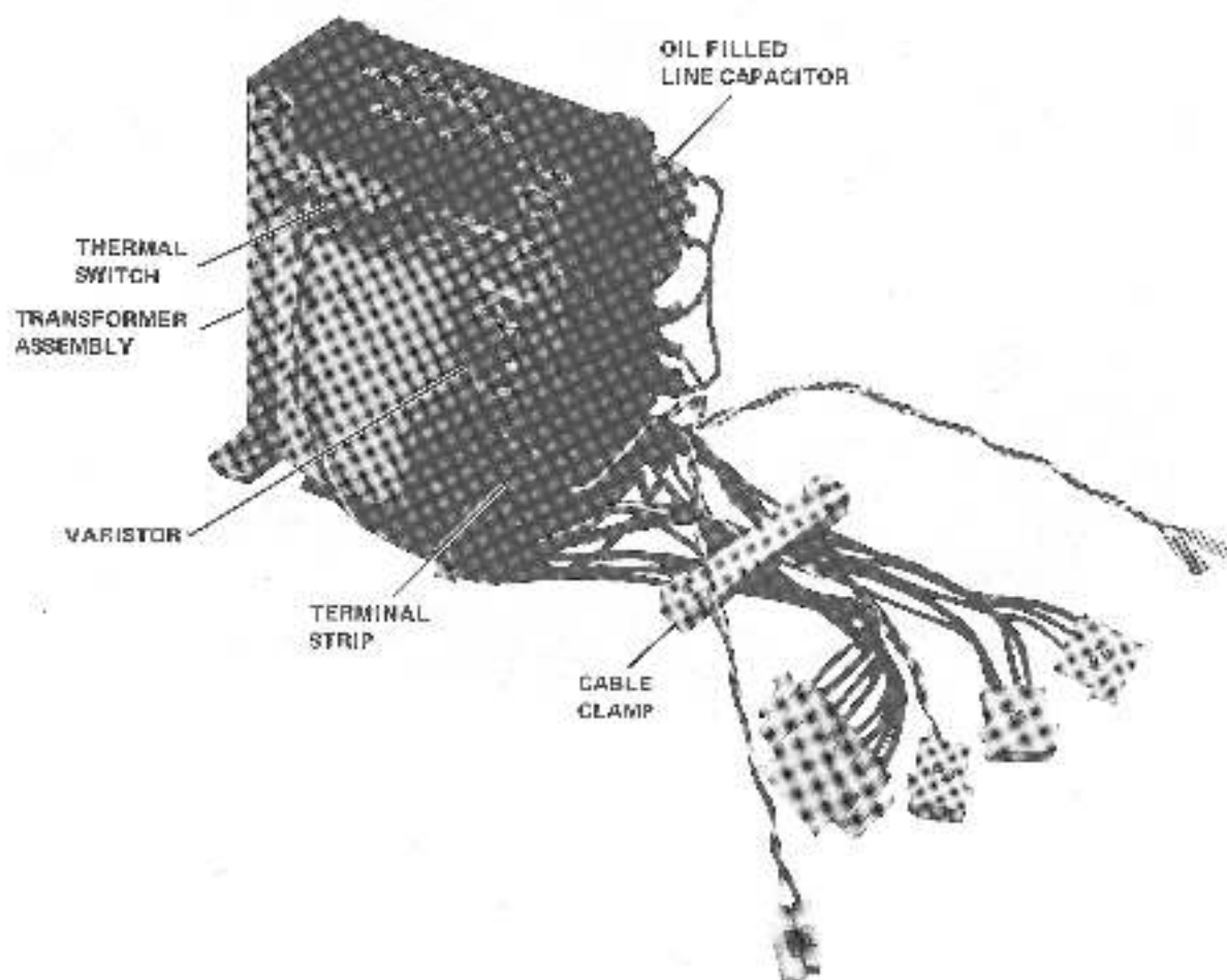
Figure 4-8 Transformer Assembly
