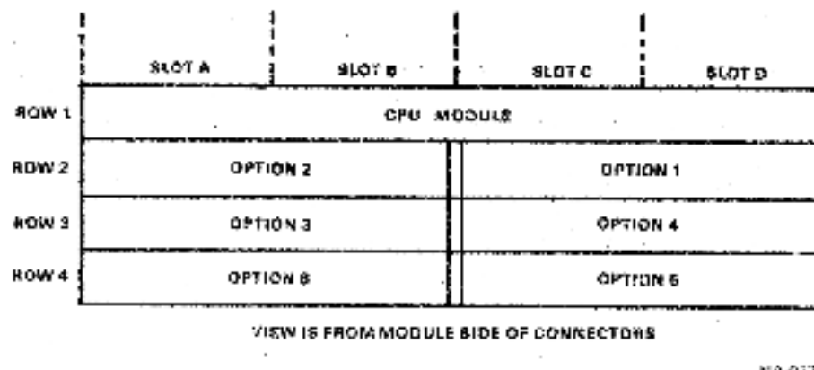
Figure 1-7 Module Installation in the H9270 Backplane
