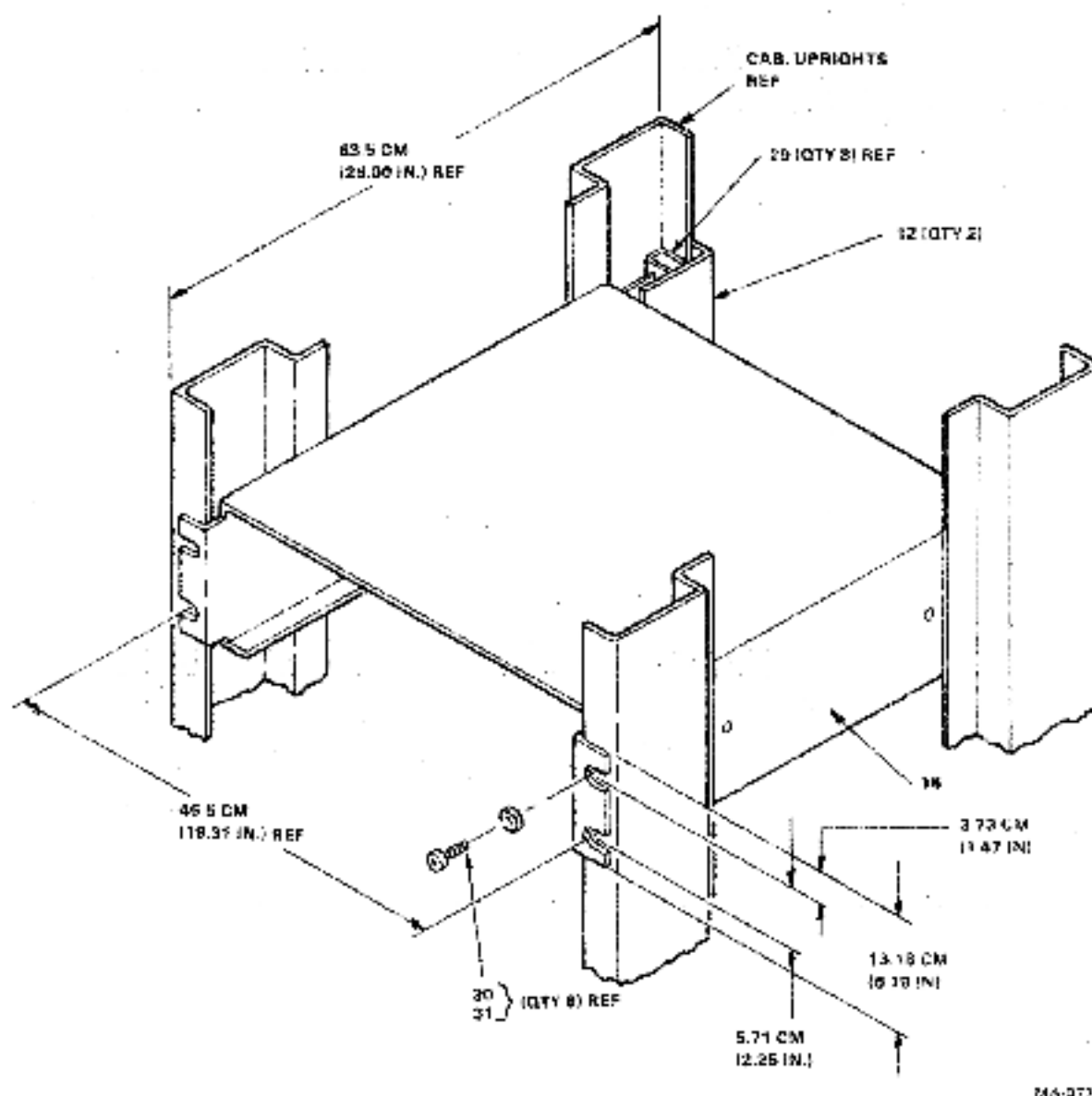
Figure 2-5 BA11-N Cover Mounting Dimensions
