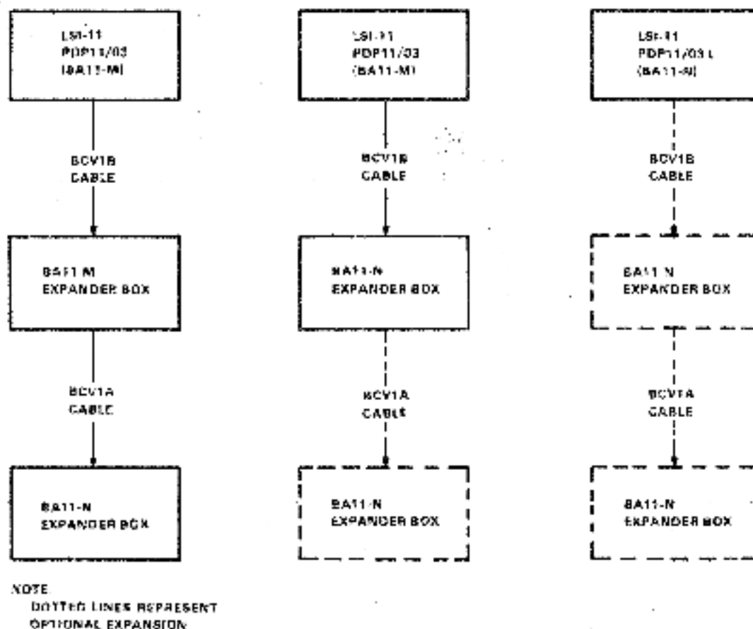
Figure 1-5 BA11-N System Applications
