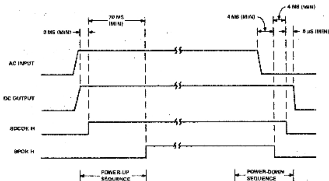
Figure I-11 Power Up/Power Down Timing
