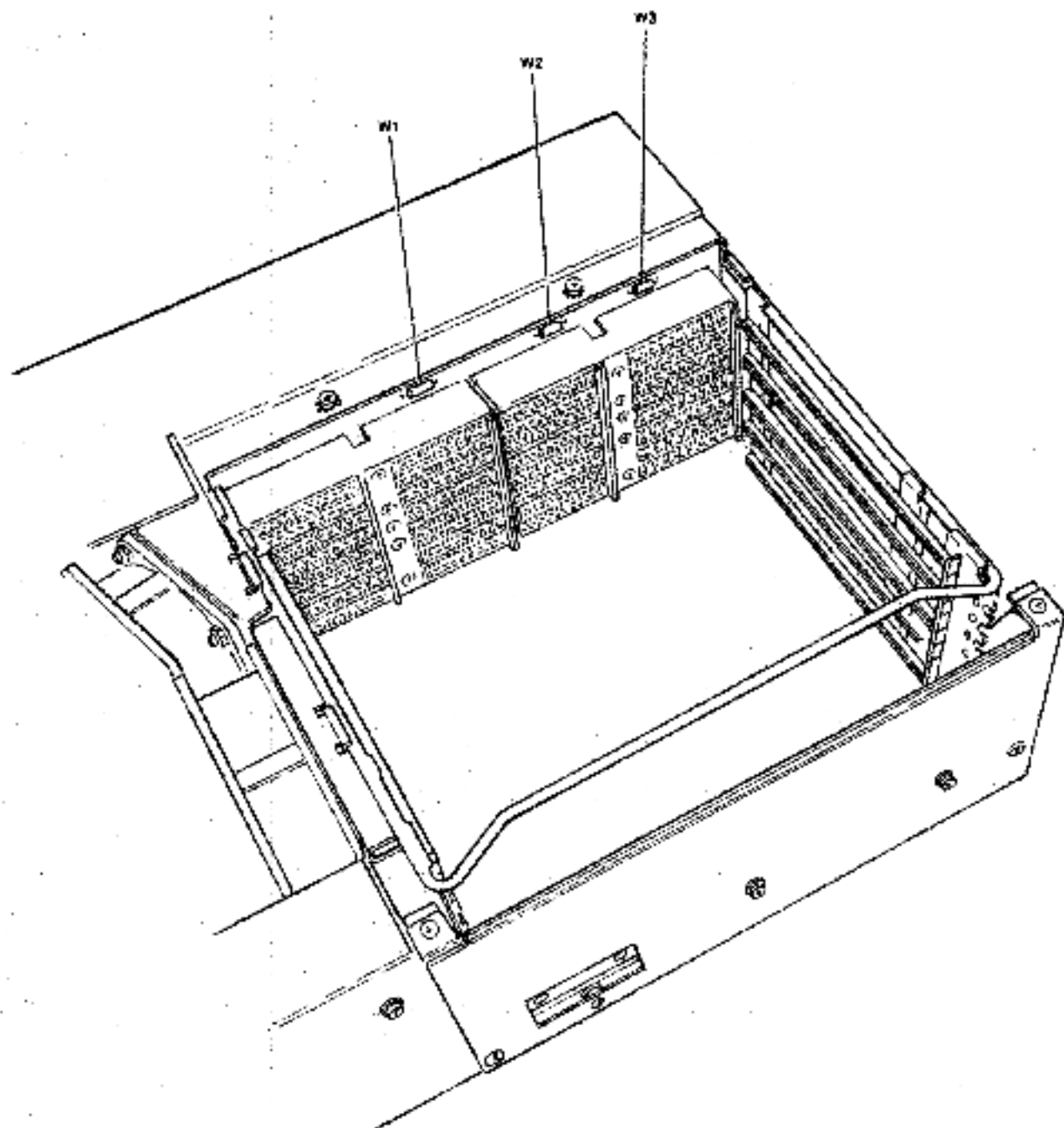
Figure 2-2 Backplane Jumpers
