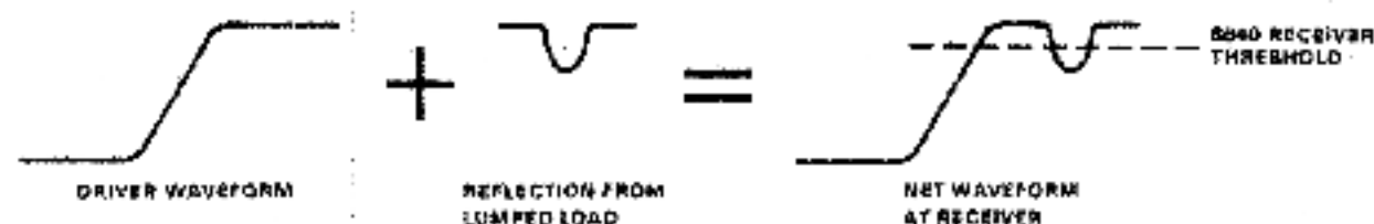
Figure 1-10 AC Loading Violation
