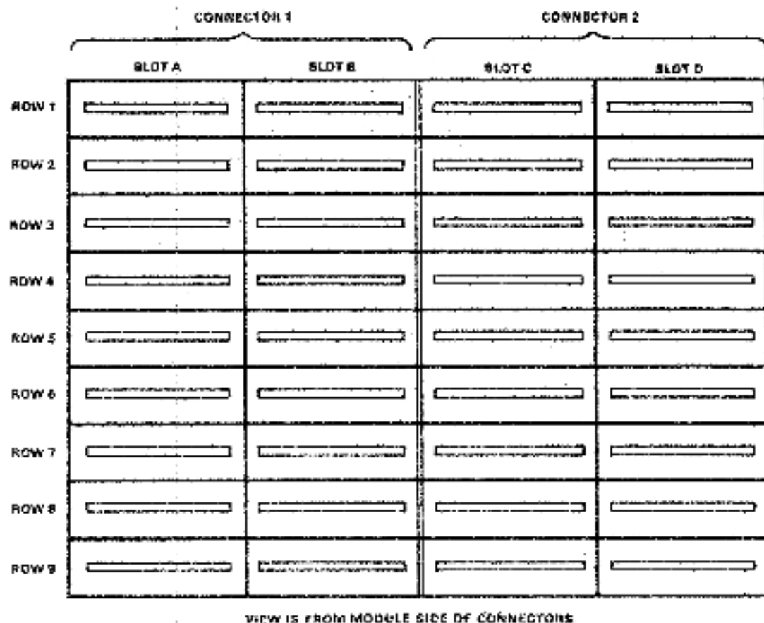
Figure 1-8 H9273 Backplane Connectors
