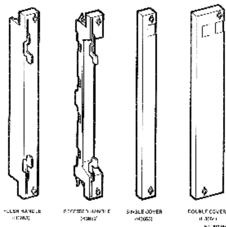
Figure 1-6: Examples of BA200 Series Handles and Covers
