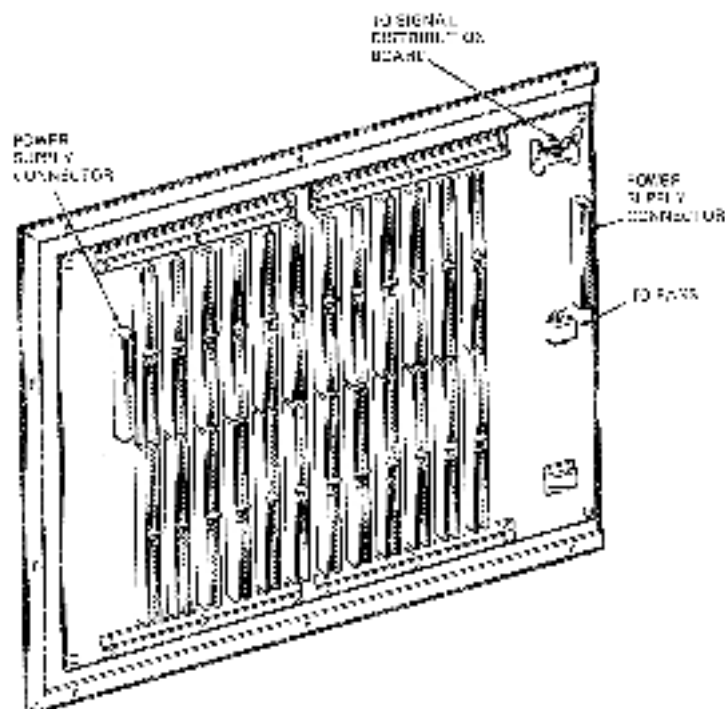
Figure B-3: BA213 Backplane
