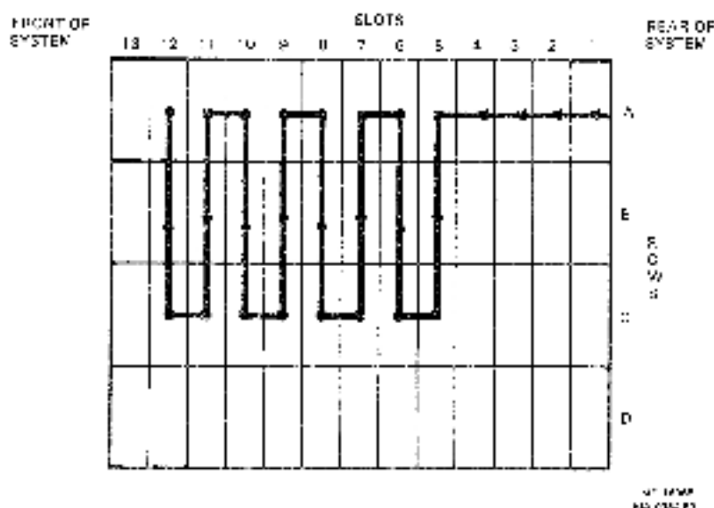
Figure B-1: BA123 Series Backplane Grant Continuity
