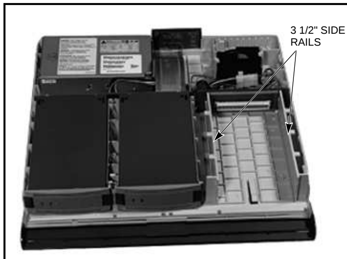
Figure 4-6 3½-Inch Side Rails Installed
