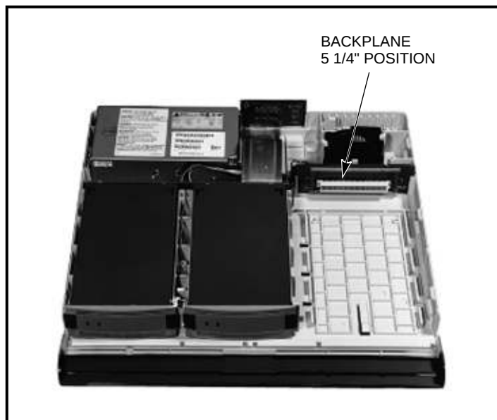
Figure 4-4 Backplane In 5¼-Inch Position
