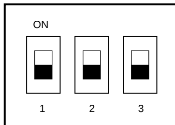
Figure 2-5 Typical Device Address Switch
